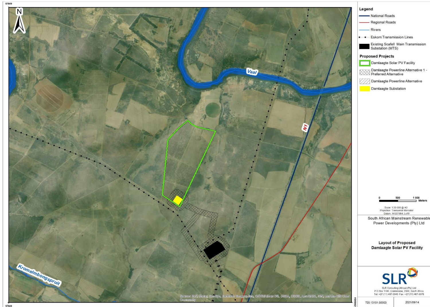
Figure 2: Location of the proposed grid connection infrastructure for the proposed grid connection infrastructure for the Damaagte Solar PV Facility in relation to the surrounding area.
