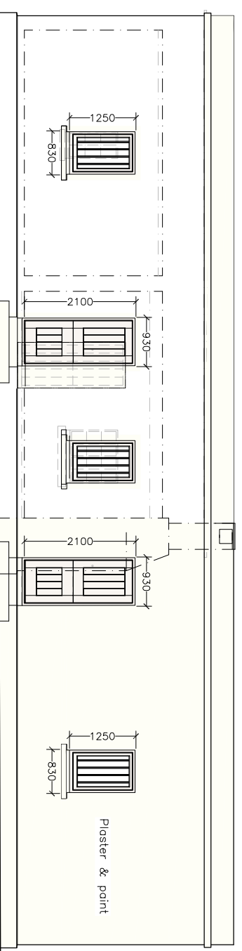
EAST ELEVATION
