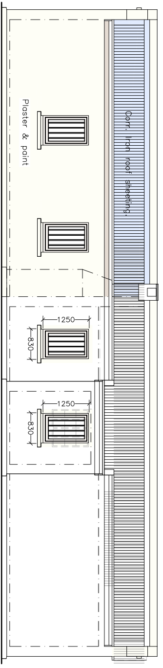
WEST ELEVATION
