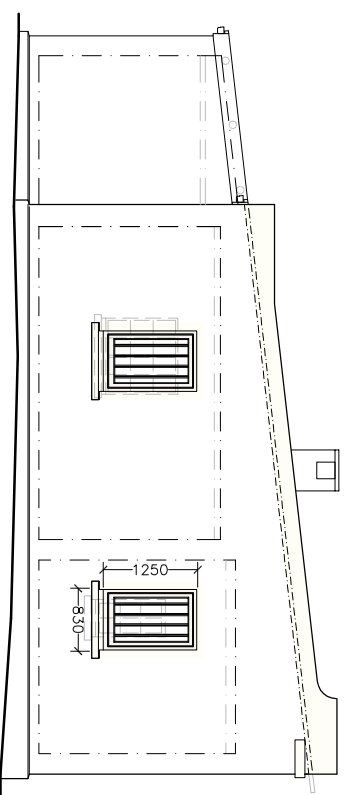
NORTH ELEVATION
