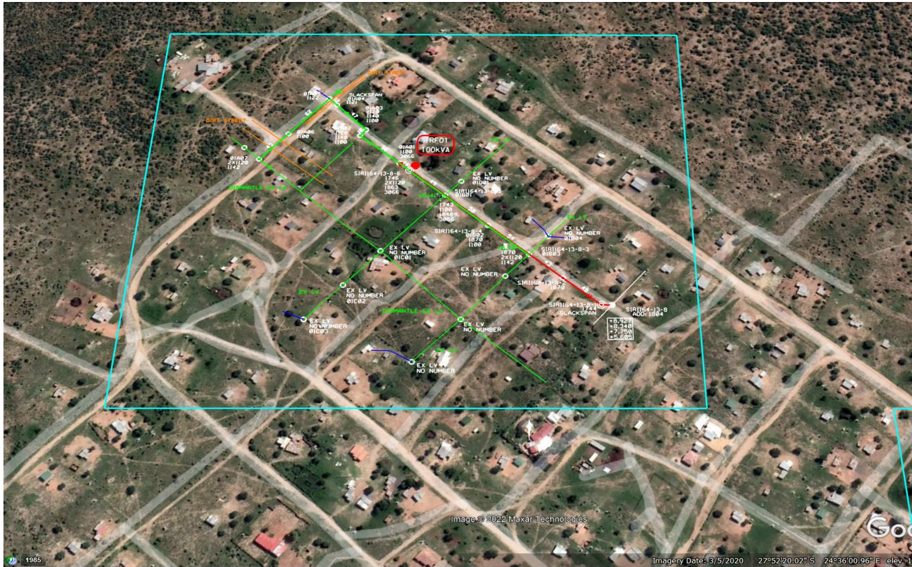
Image 2. Proposed power line in green and red. Existing power line in white and orange.
