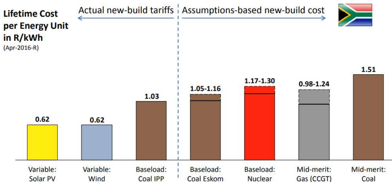
Figure 1-1: Power cost per kWh for the main generation types under consideration by South Africa (CSIR, 2016)
