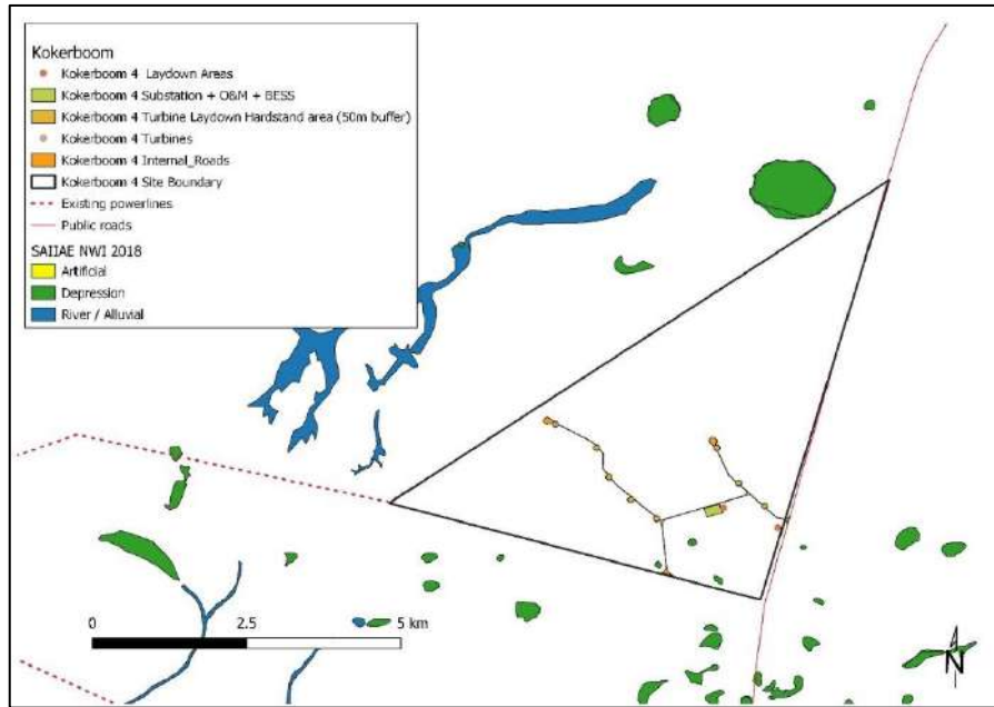
Figure 6-10: National Wetland Inventory wetlands and waterbodies (van Deventer et al. , 2018) for the wind farm
