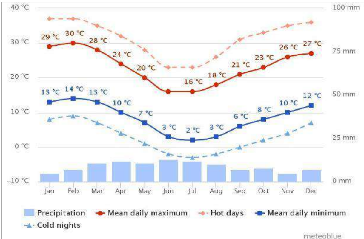
Figure 6-1: Average temperature and rainfall for Loeriesfontein
