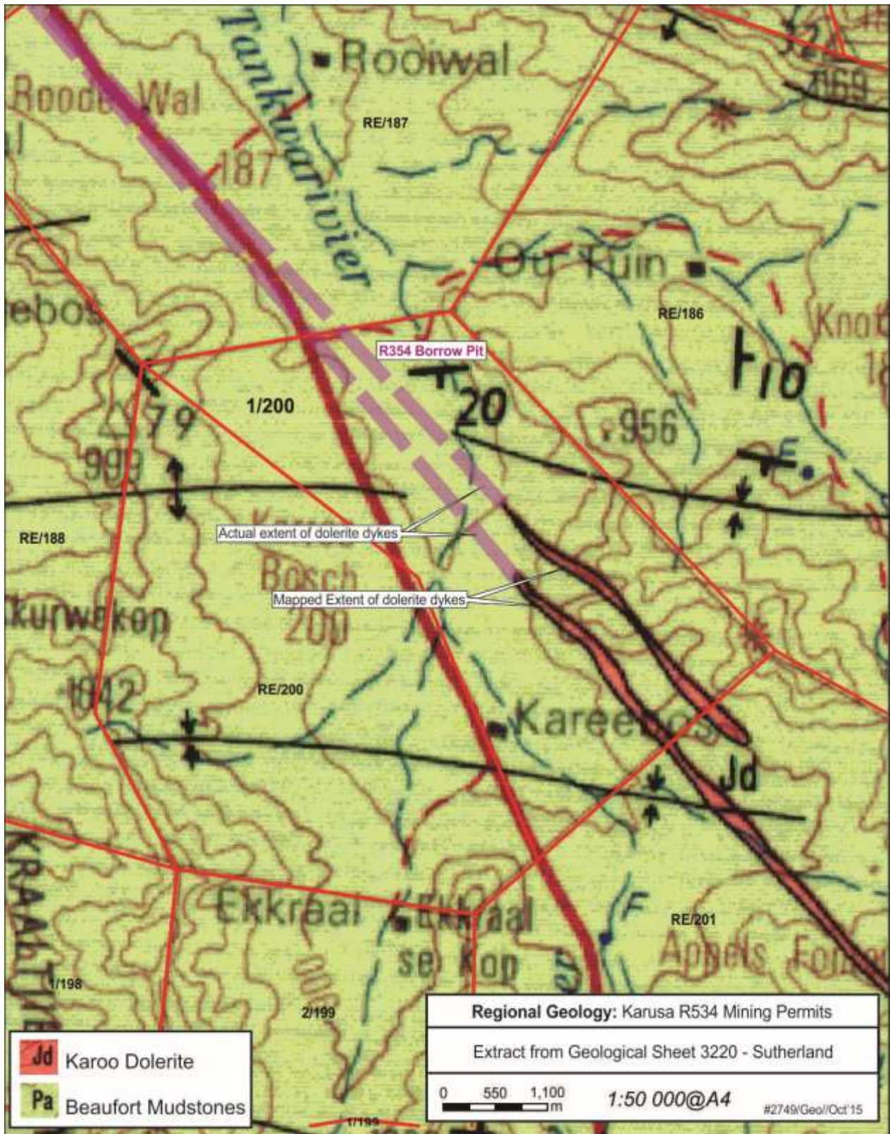
Figure 3: Regional Geology
