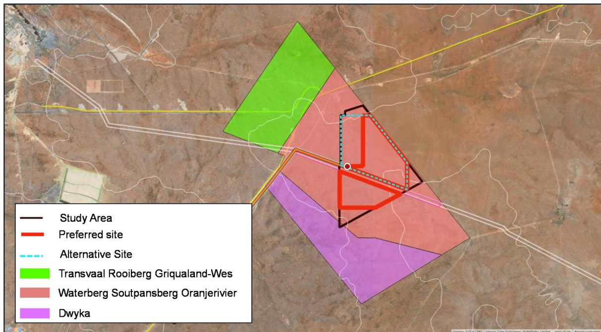
Figure 3: Geology
