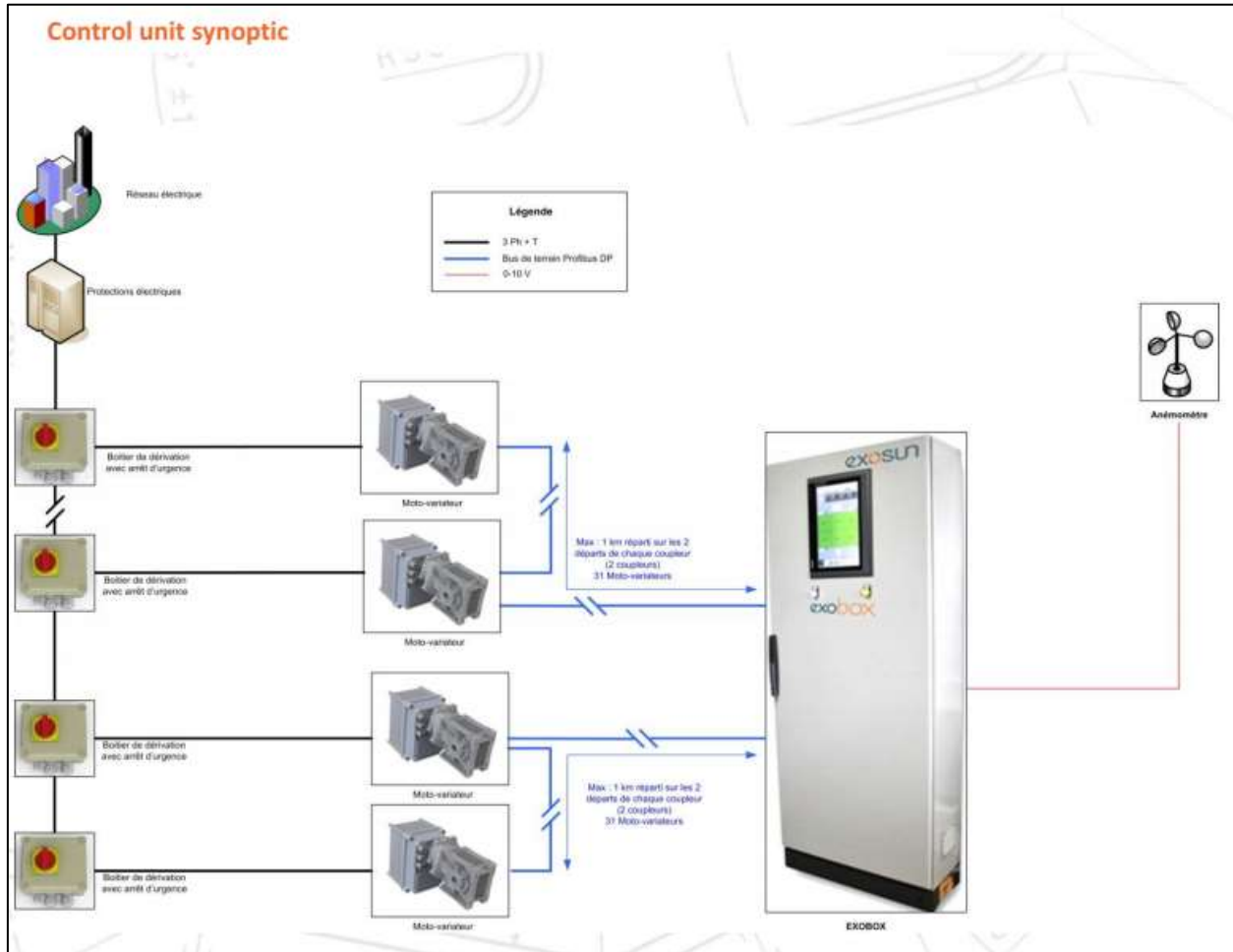
Figure 2: Control system diagram
