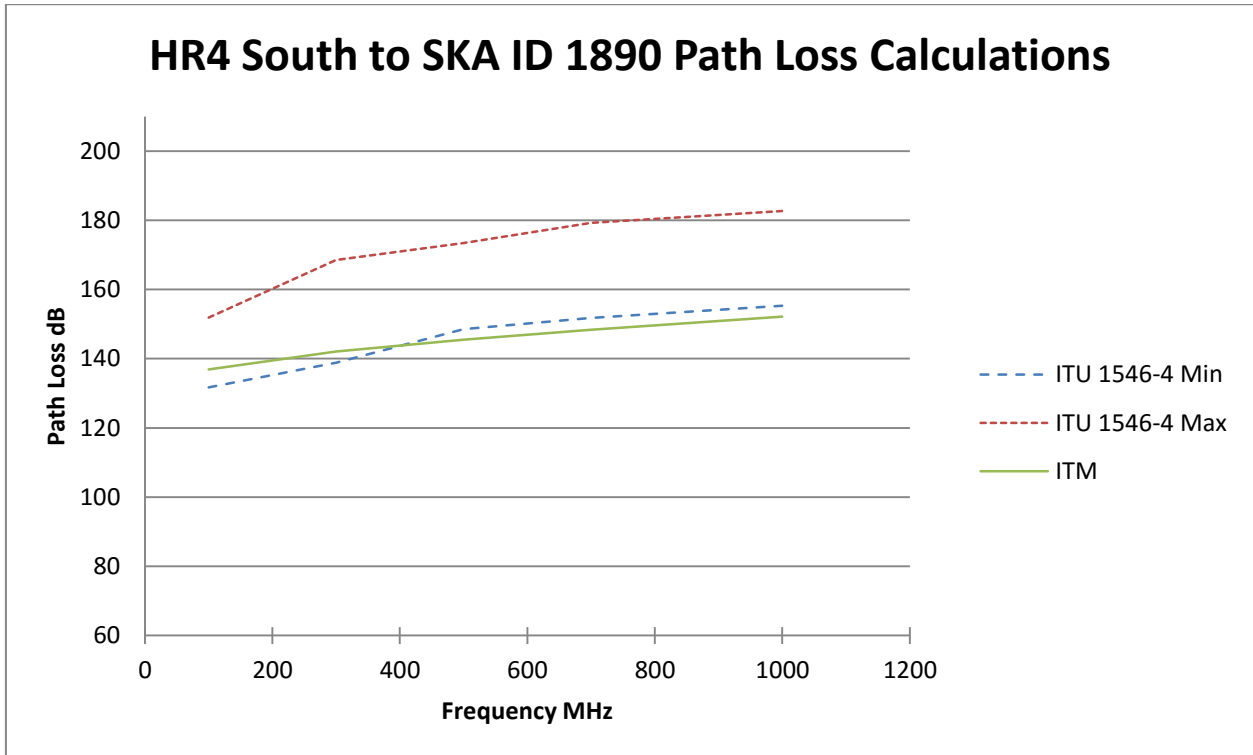
Graph 2: HR4 South to SKA ID 1890 Calculation Results
