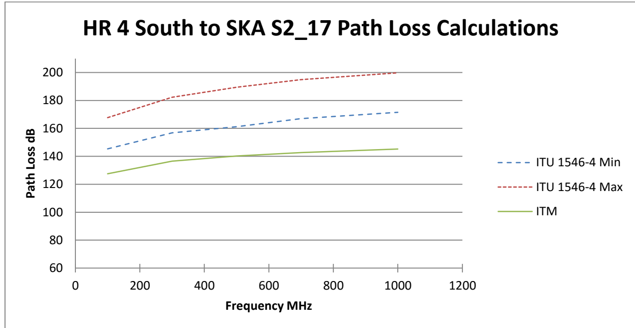
Graph 3: HR4 South to SKA S2 17 Calculation Results
