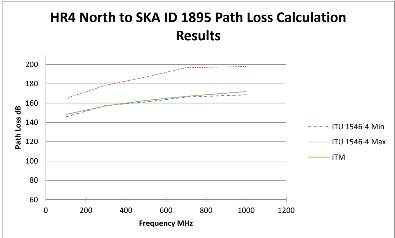
Graph 1: HR4 North to SKA 1895 Path Loss Calculation Results
