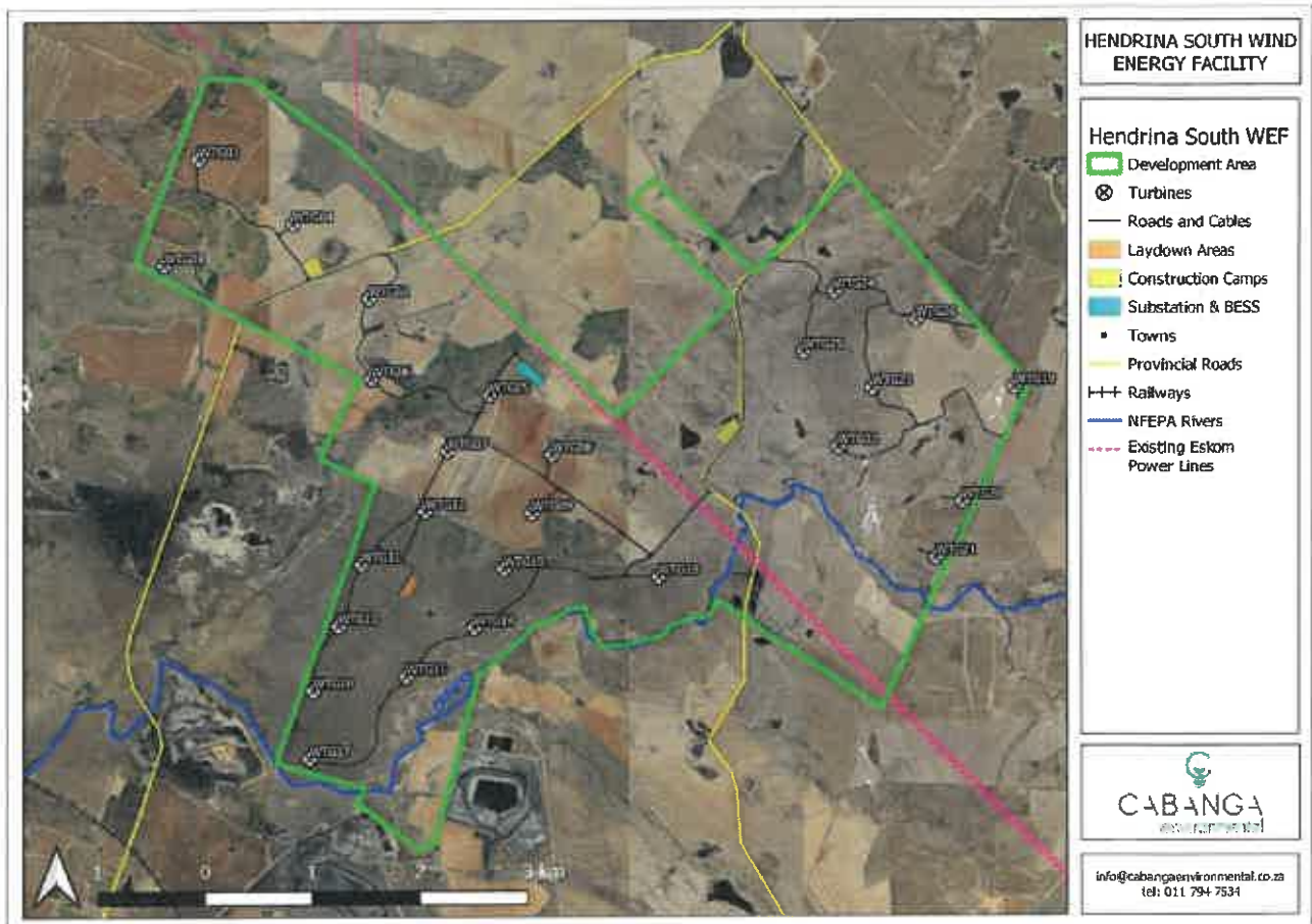
Plan 4: South WEF Layout Map
