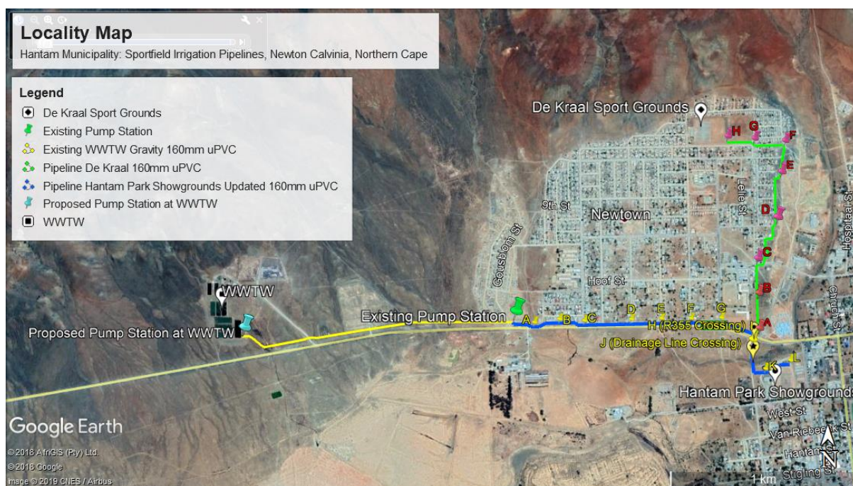
Figure 1: Layout plan indicating the existing pipeline from the Calvinia WWTW to the existing pump station (yellow line). The blue line indicates the rising main pipeline to Hantam Park Showgrounds. The green line indicates the rising main pipeline to De Kraal Sport Grounds.
