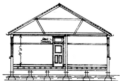
SECTION AB
