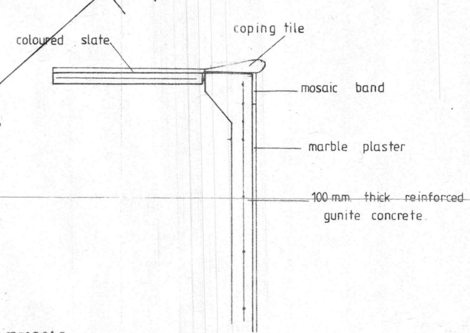
DETAIL SECTION
