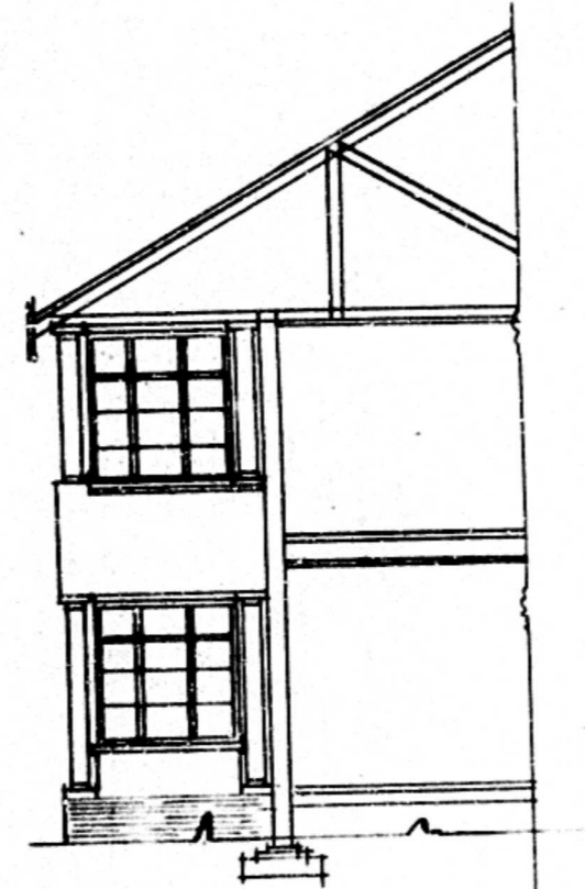
PART SECTION AA
