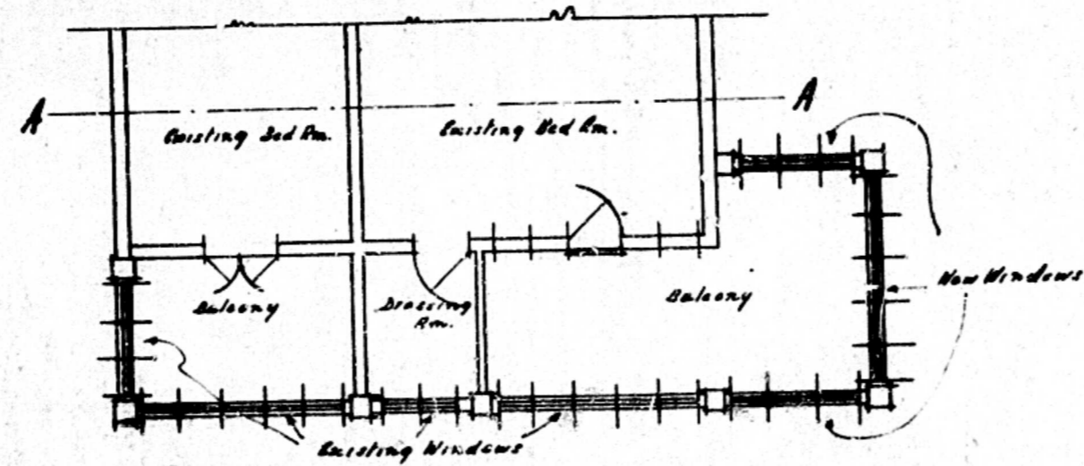
PART FIRST FLOOR PLAN
