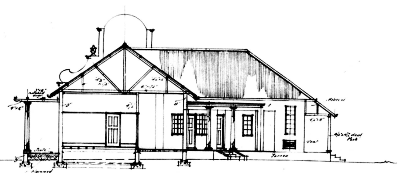
Section C-D.
