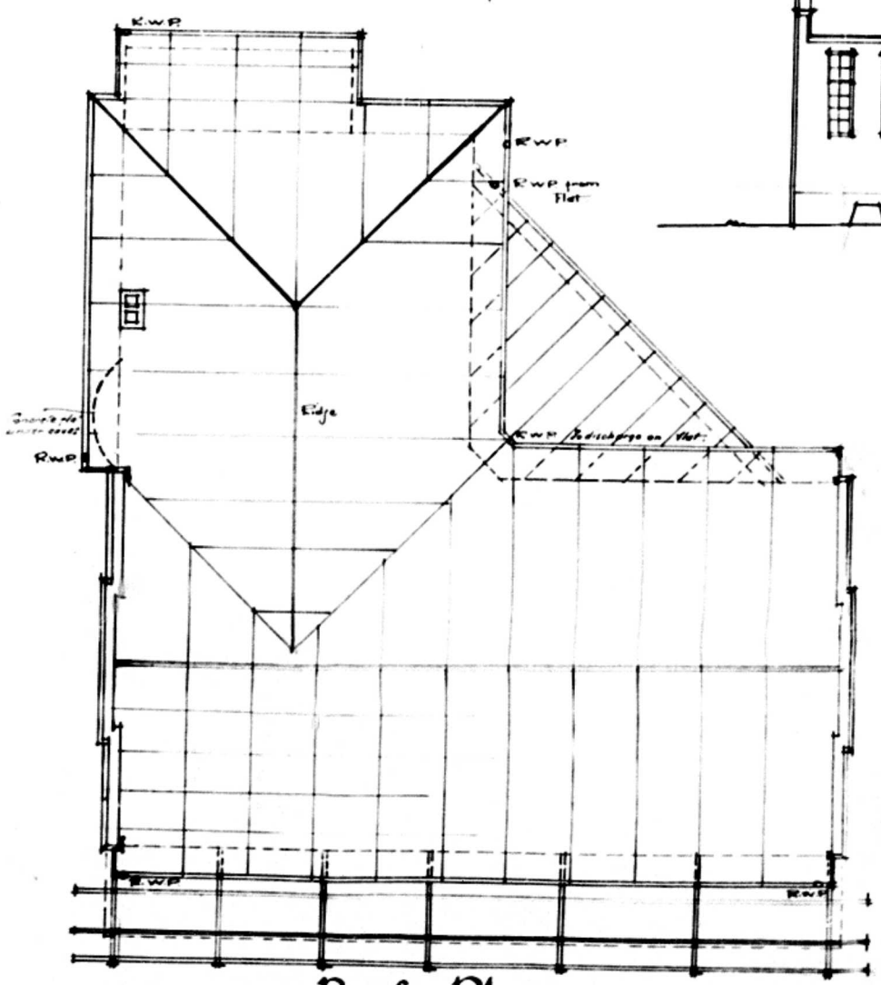
Roof Plan.
