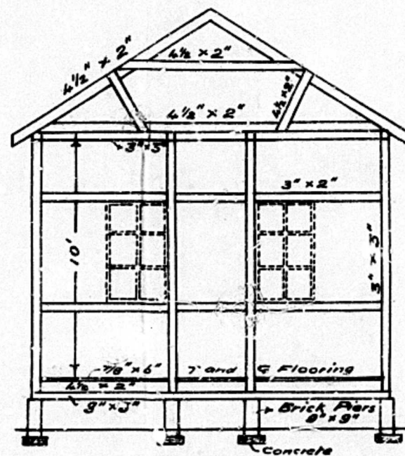
Cross Section
