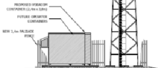
Alternative 1 Mast Elevation - Lattice Mast
