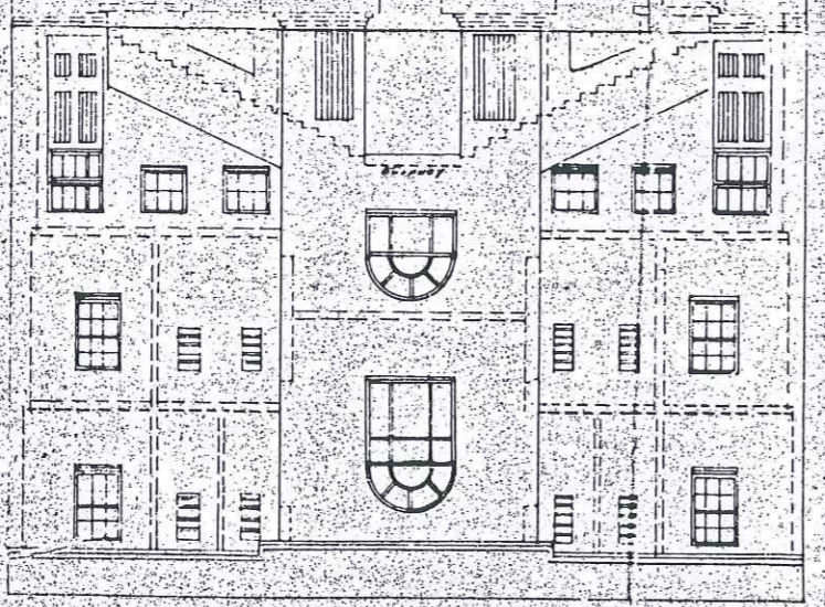
BACK ELEVATION
