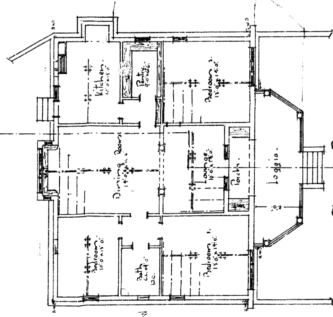
FLOOR PLAN
