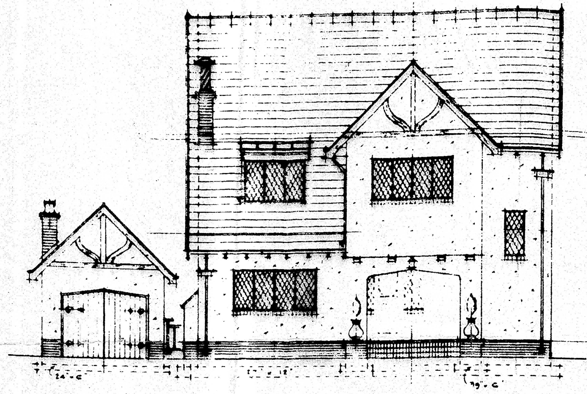
FRONT ELEVATION
