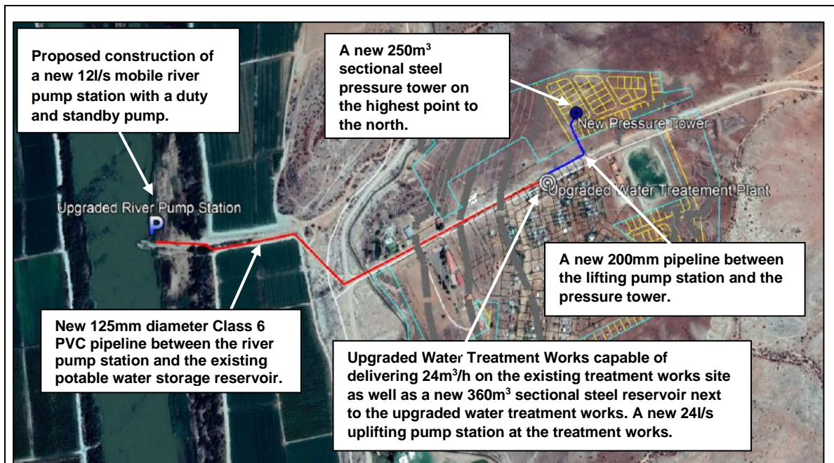
Figure 5. Recommended upgrades to existing bulk water infrastructure for the proposed Gariep Housing Development. Source: Engineering Services Investigation Report, August 2020.
