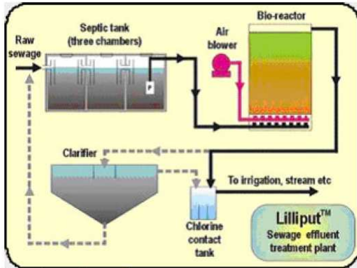
Figure 2: Process Plan
