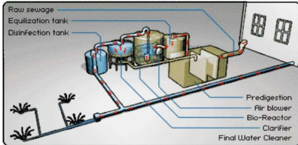
Figure 1: Process Overview
