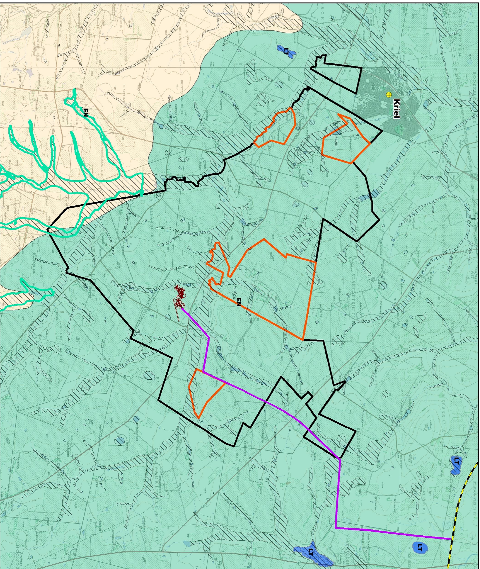
Figure 17: National Freshwater Ecological Priority Areas and Threatened Ecosystems
