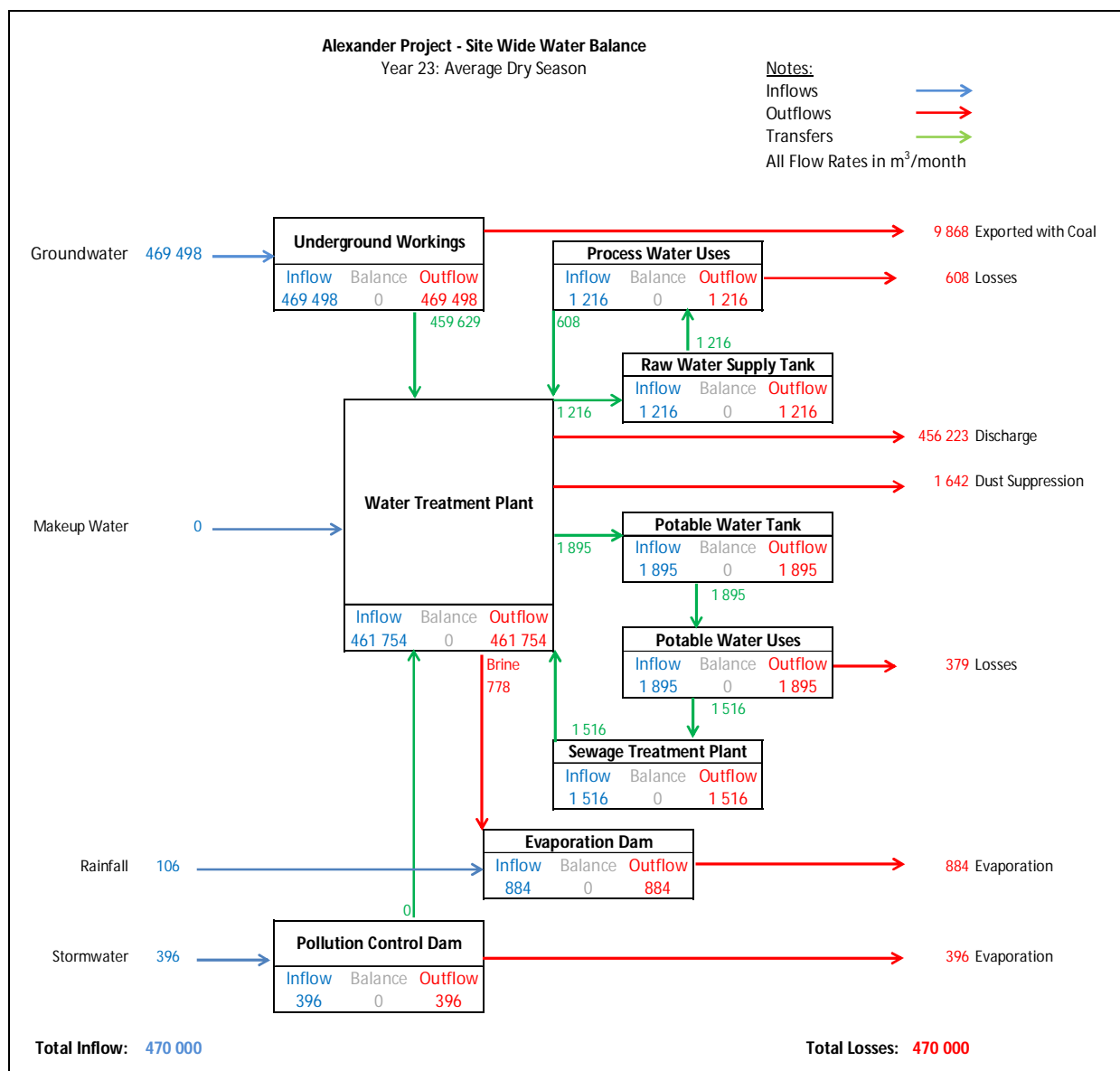
FIGURE 6: DRY SEASON WATER BALANCE (SLR, 2016)
