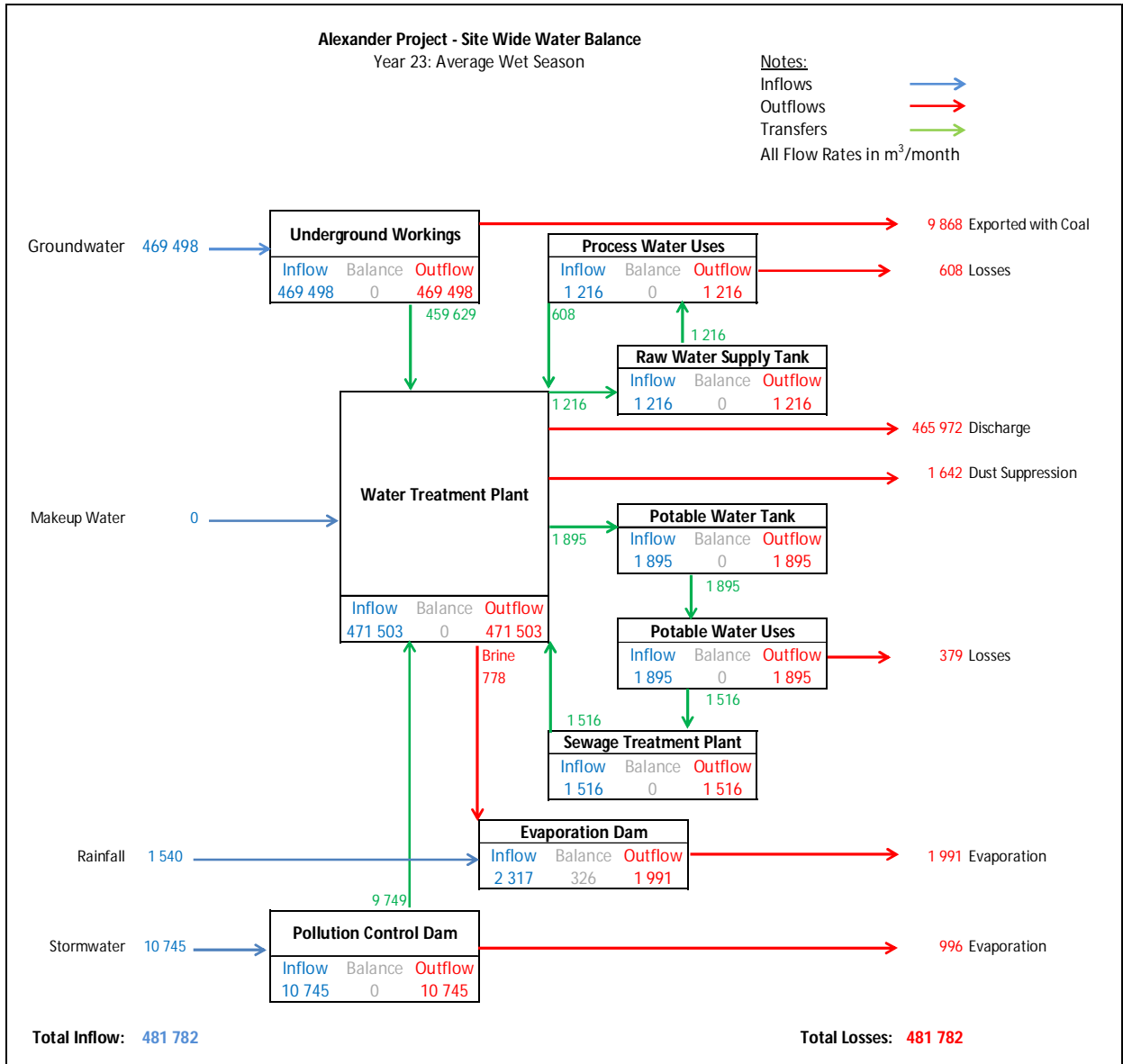
FIGURE 7: WET SEASON WATER BALANCE (SLR, 2016)
