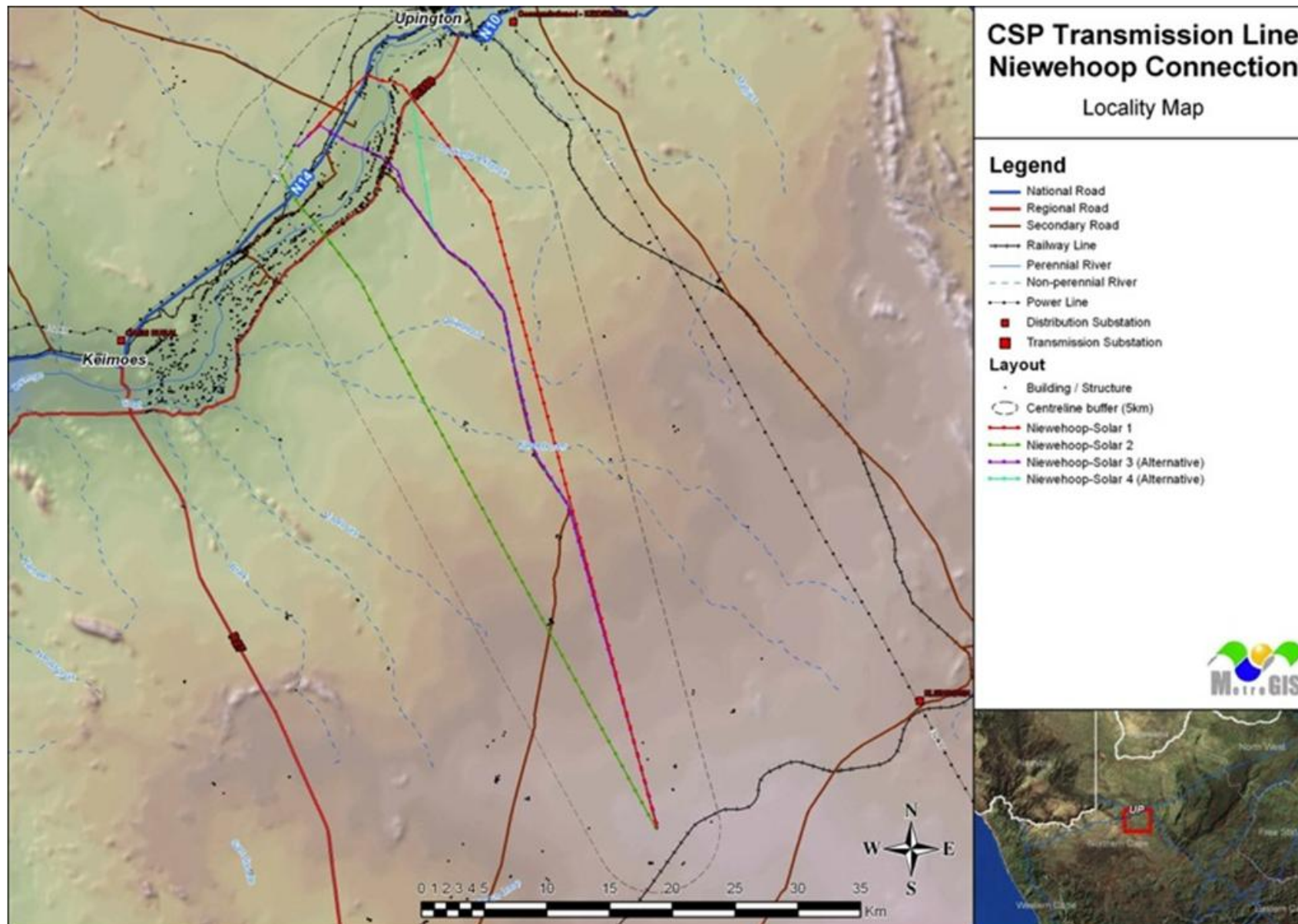
Figure 7-35: Locality and proposed alignment of the Nieuwehoop Corridor and alternatives.
