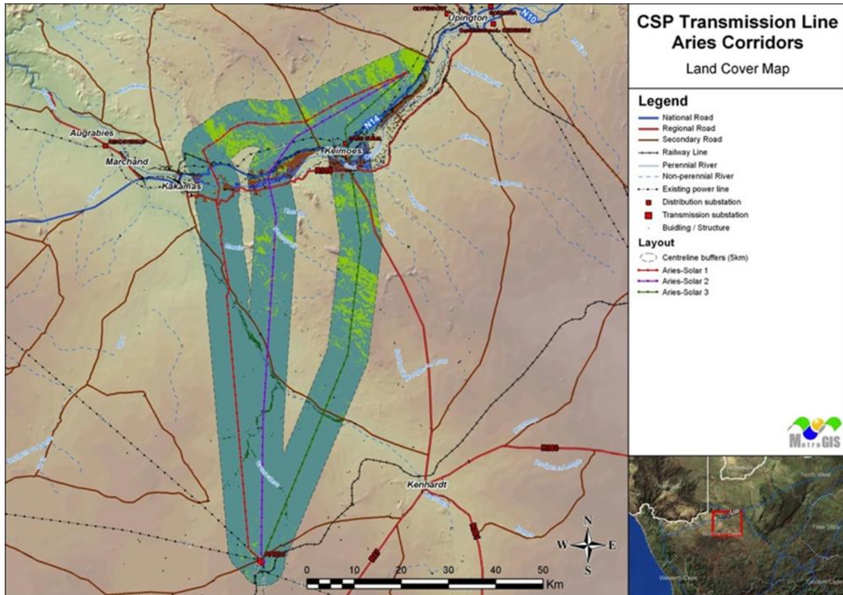
Figure 7-36: Land cover and land use along the Aries Corridor and alternatives
