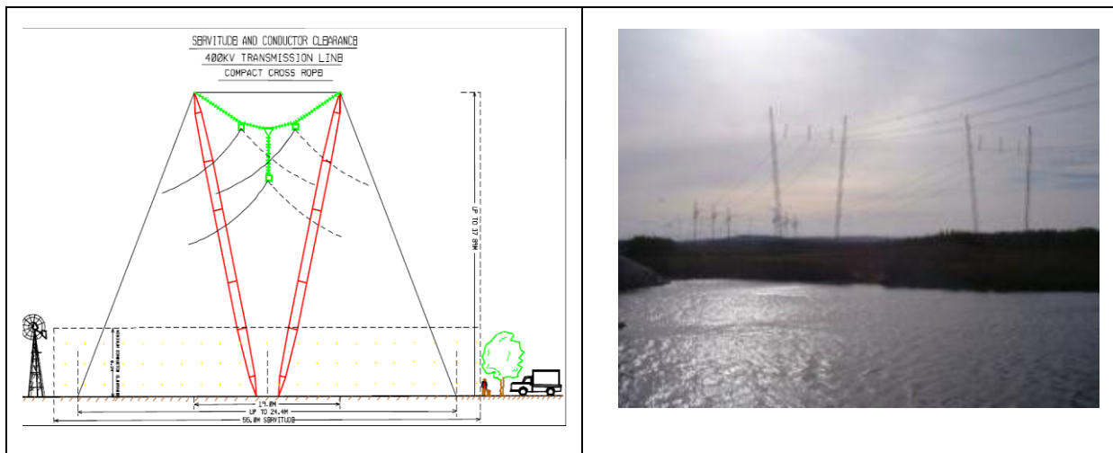
Figure 6-4: Compact cross rope suspension tower.
