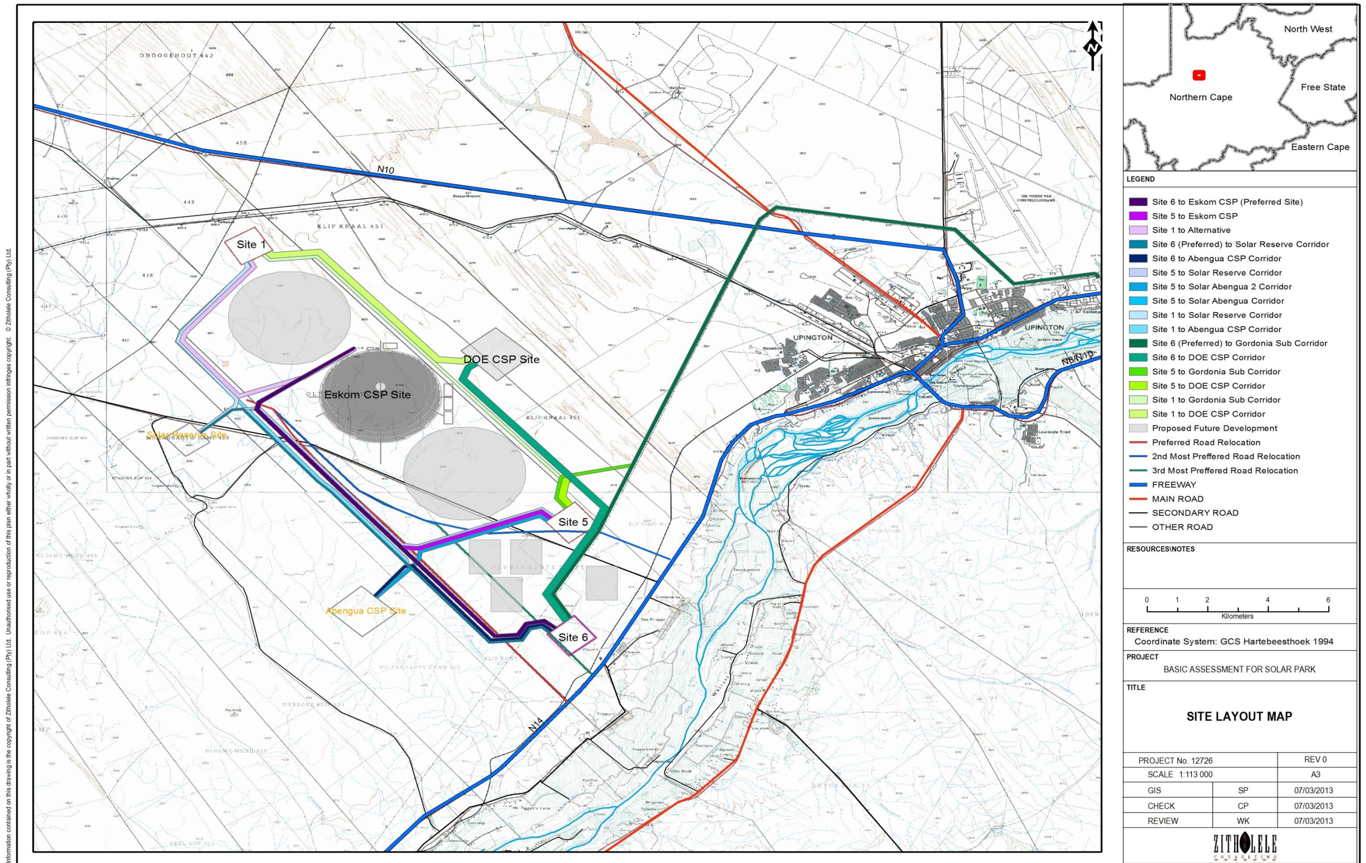
Figure 6-6: Alternative substation sites
