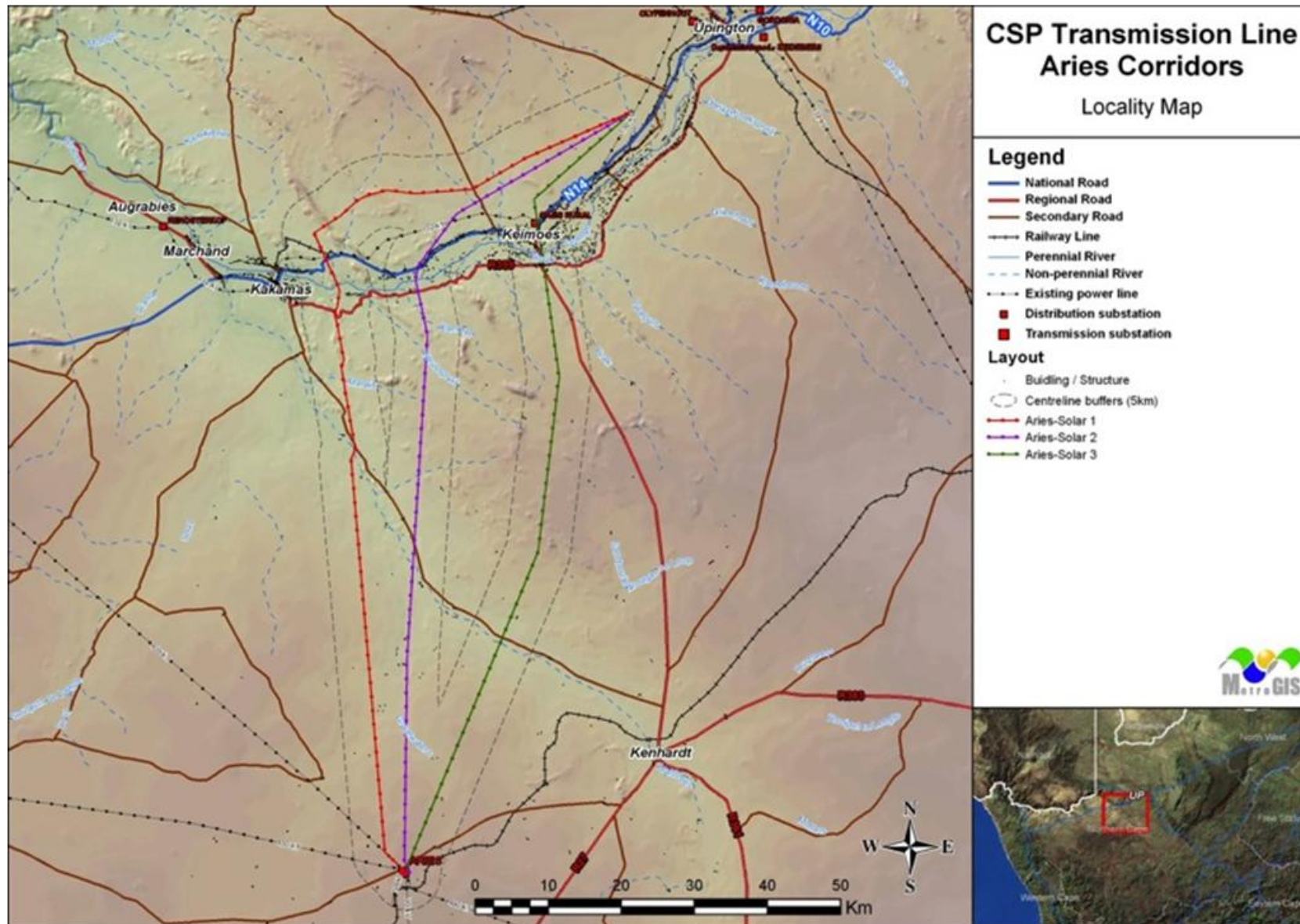
Figure 7-34: Locality and proposed alignment of the Aries Corridor and alternatives
