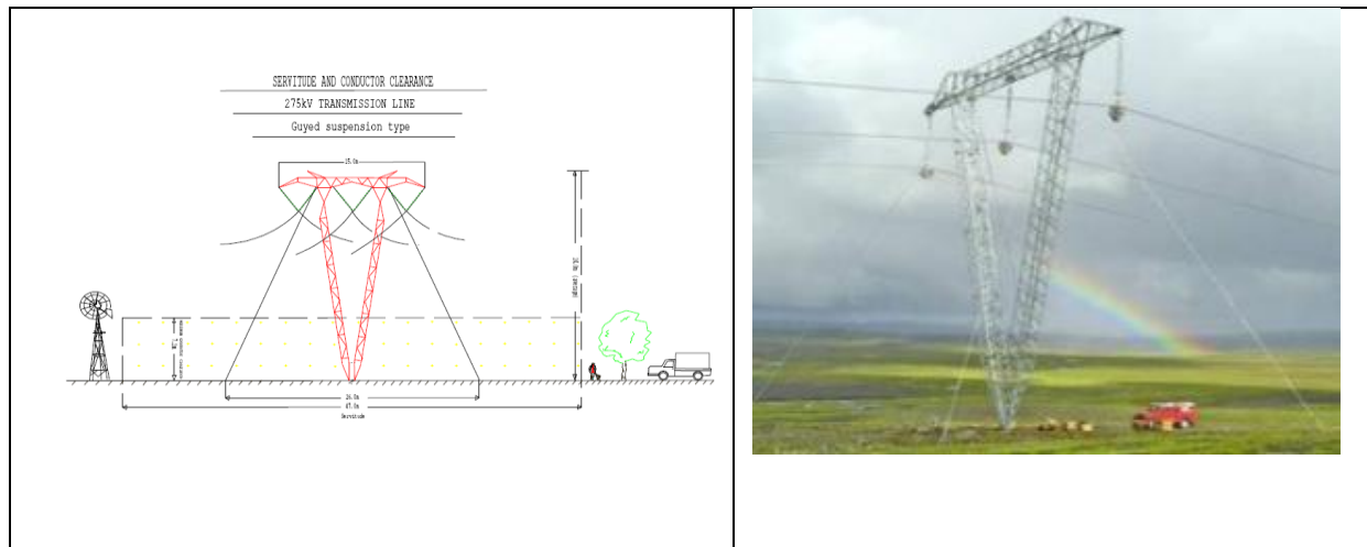
Figure 6-5: Guyed-V suspension tower.
