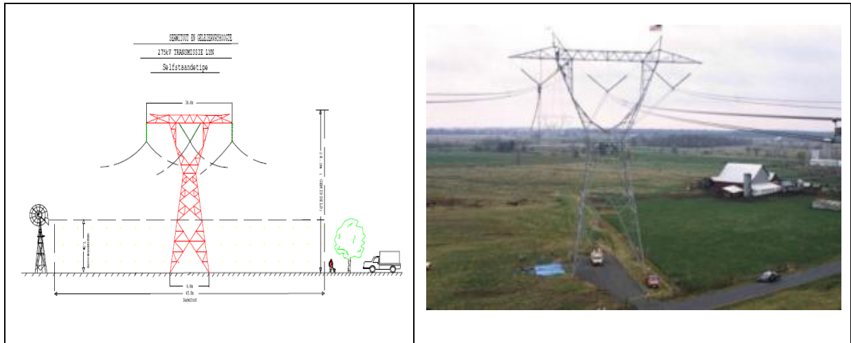
Figure 6-1: Self-supporting suspension tower.
