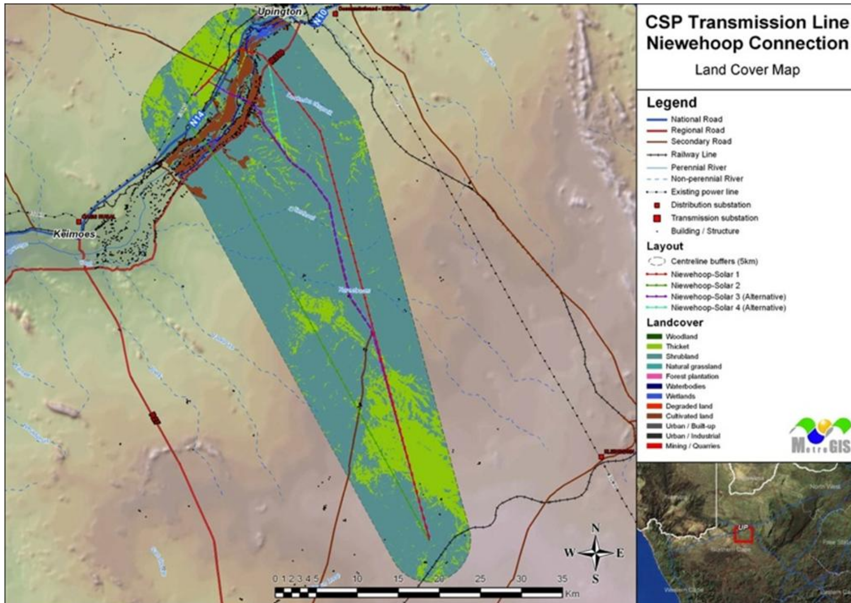
Figure 7-37 Land cover and land use along the Nieuwehoop Corridor and alternatives.
