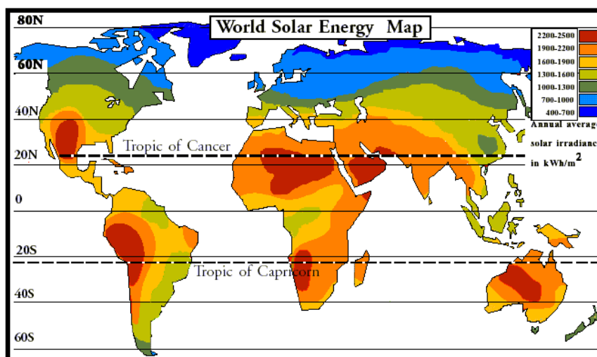
Figure 1-5: Model of solar radiation patterns
