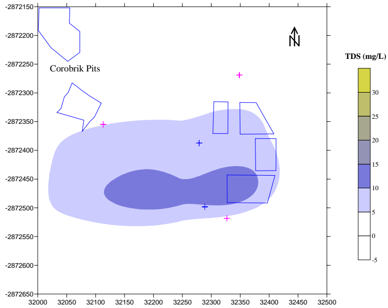
Figure 91. Modelled TDS concentrations in the deep aquifer system – end 2021.
