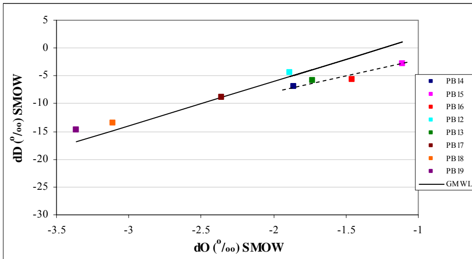
Figure 13. \delta\text{D} versus \delta^{18}\text{O} for the groundwater samples from the Raw Water Dam and Sewage Plant.
