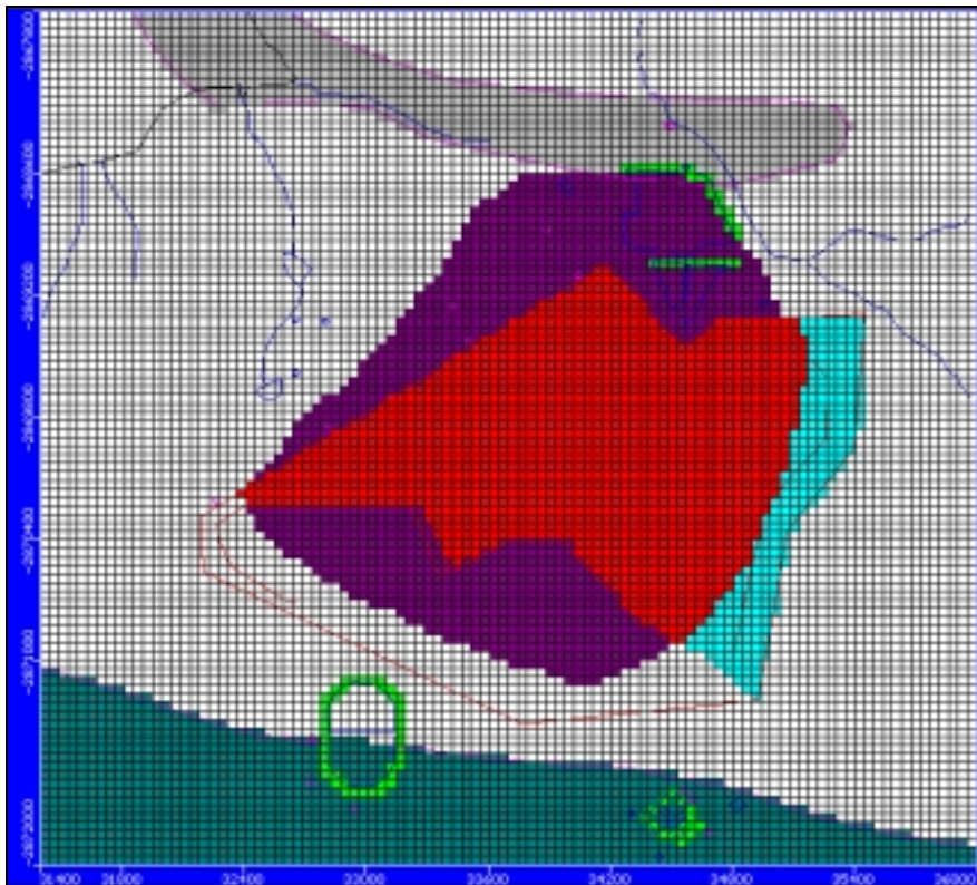
Figure 18 Geohydrological zone distribution in Layer 2.
