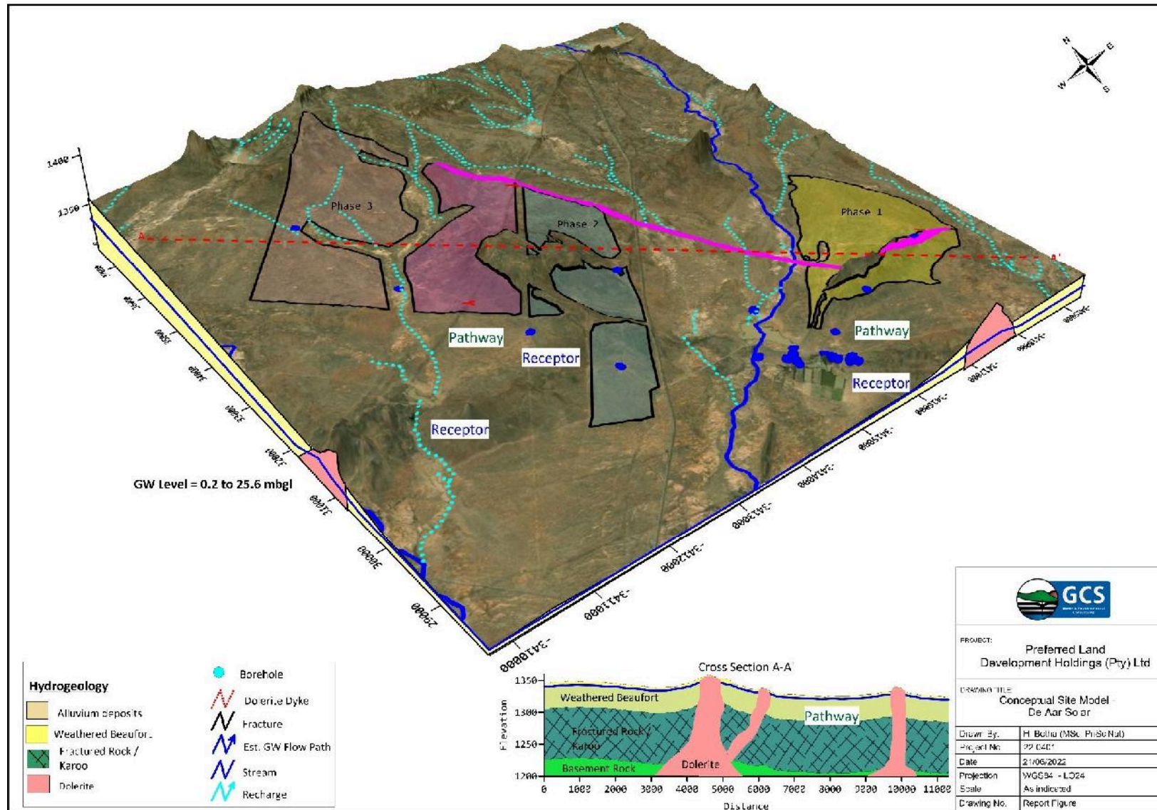
Figure 6-1: Site conceptual model (SCM)
