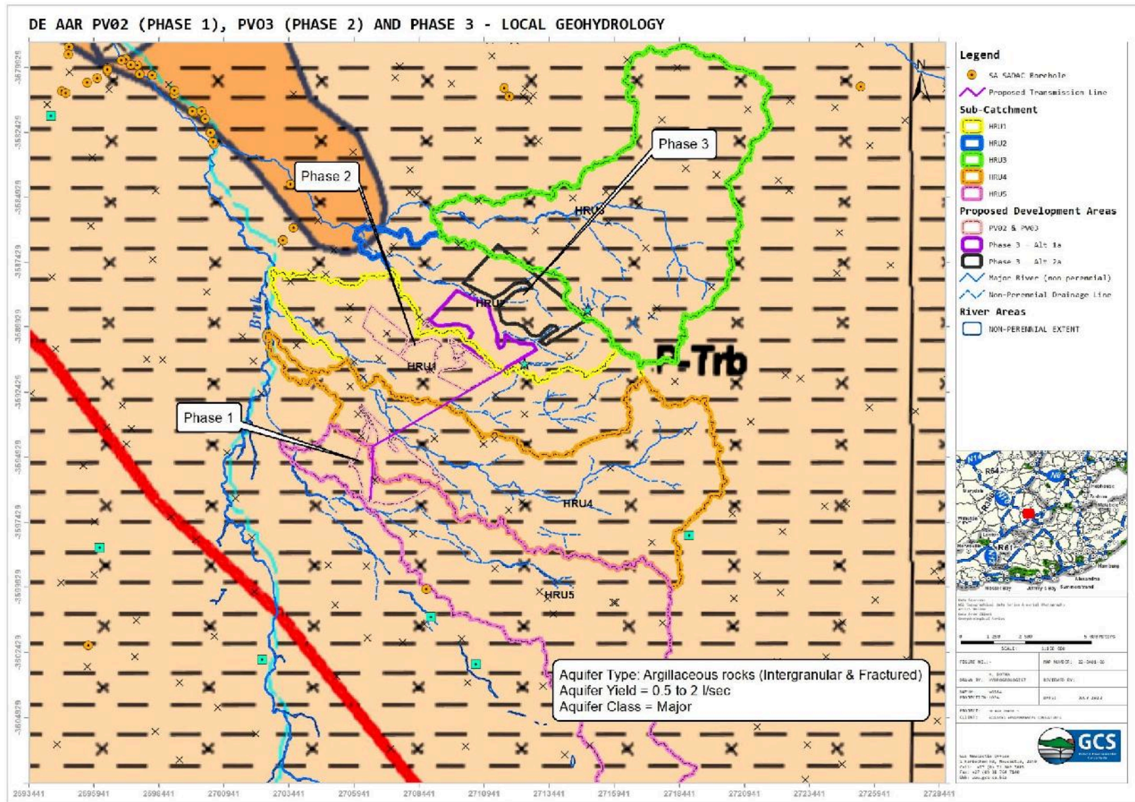
Figure 5-2 Local hydrogeology
