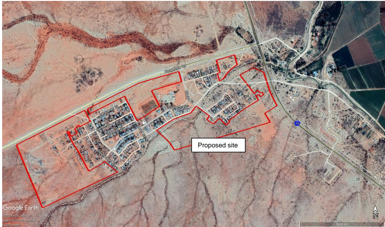
Figure 3: Google Earth image of the surrounding landscape, showing the location of the proposed development in relation with the existing residential areas.
