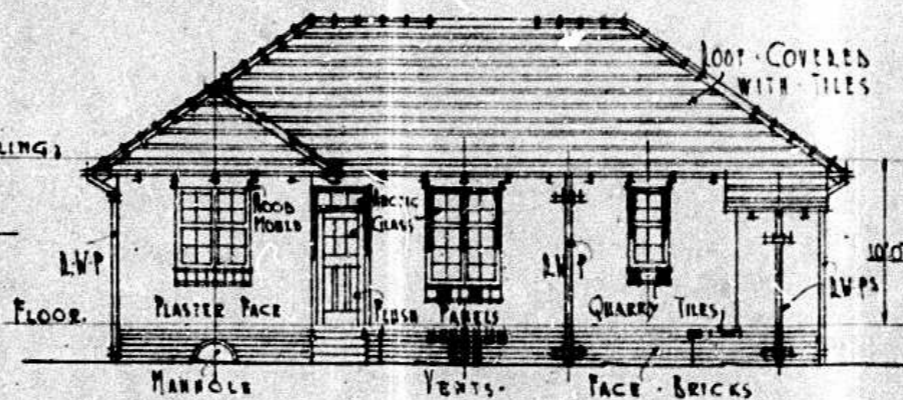
BACK ELEVATION
