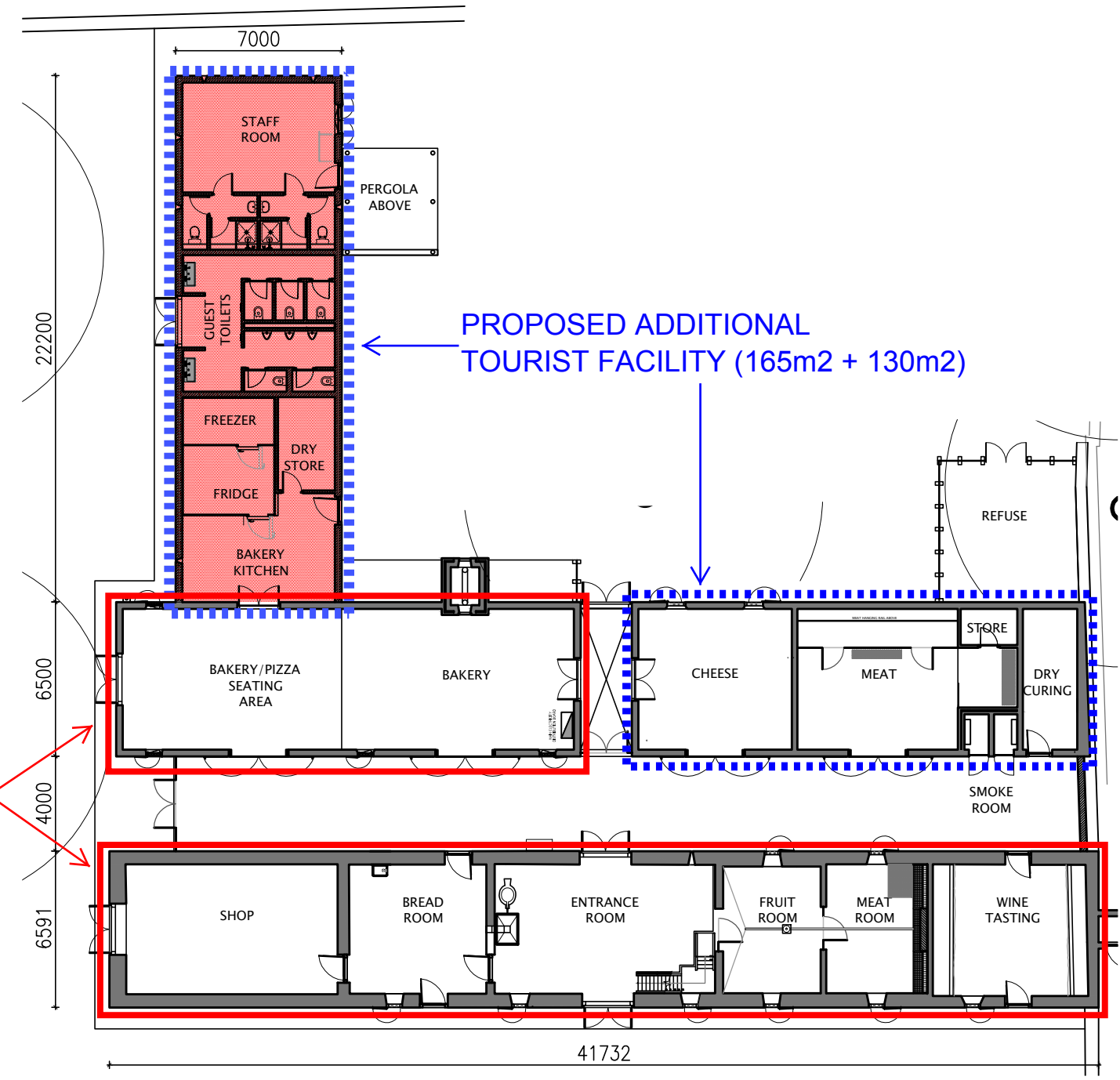
PROPOSED FLOOR PLAN 1:250 @A3 7 TOILETS
