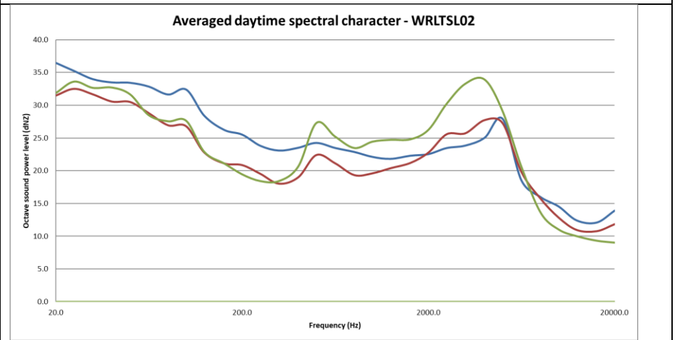
Figure 4-17: Average daytime frequencies at WRLTSL02
