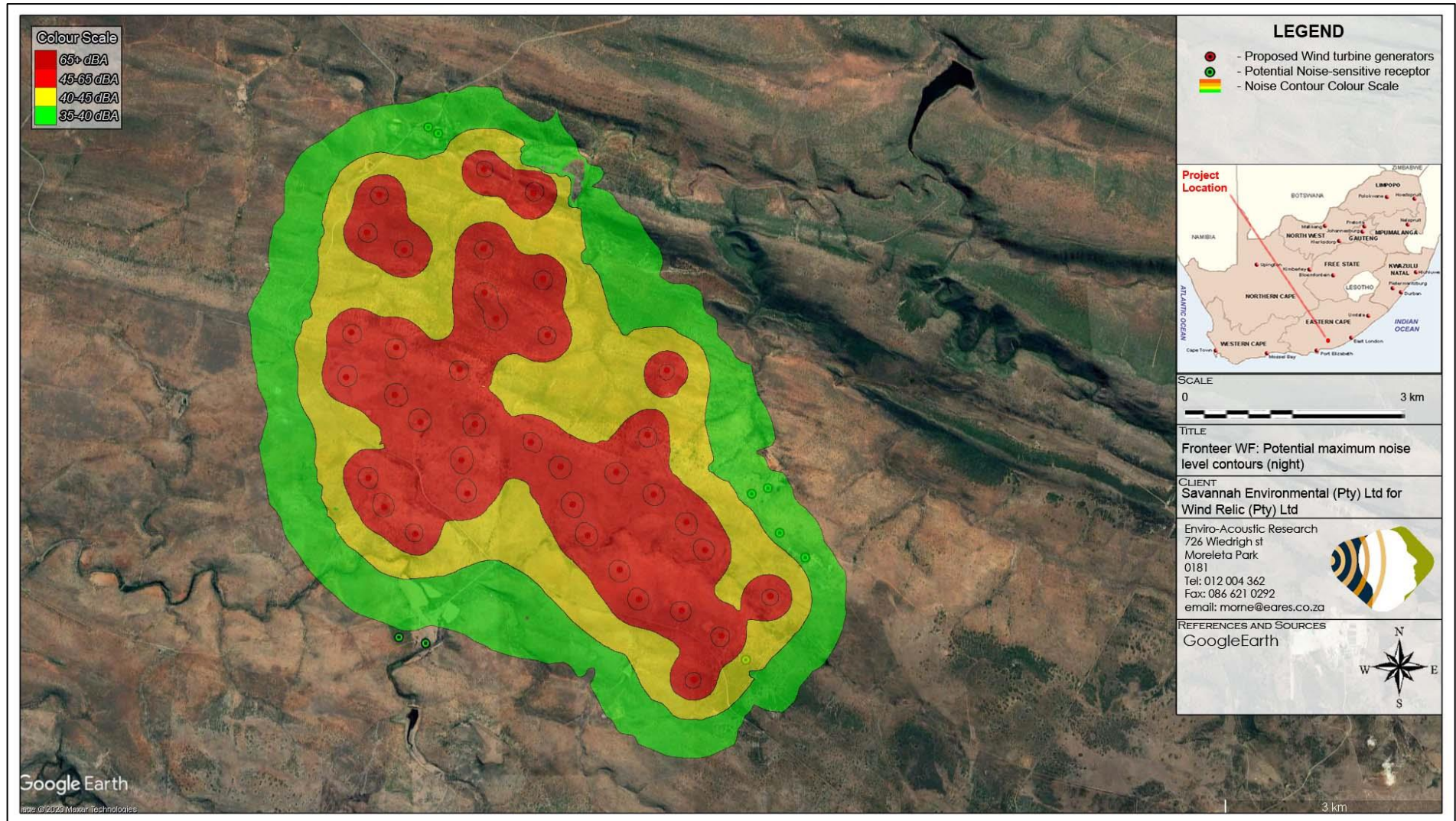
Figure 8-4: Projected maximum night-time operational noise rating levels due to operation of Frontier WF
