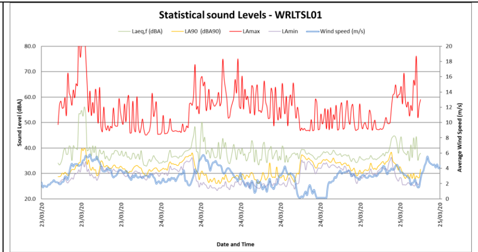
Figure 4-3: Maximum, minimum and Statistical sound levels at WRLTSL01
