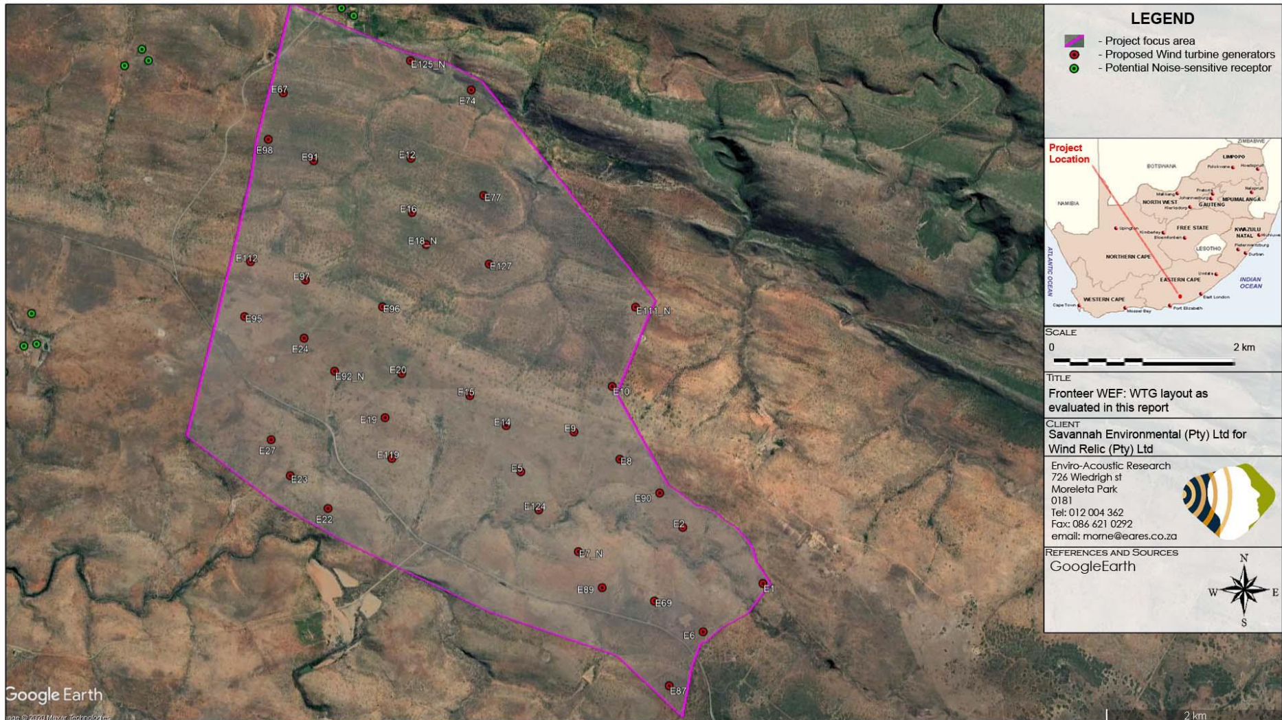
Figure 8-1: Proposed WTG Layout of the Frontier WF
