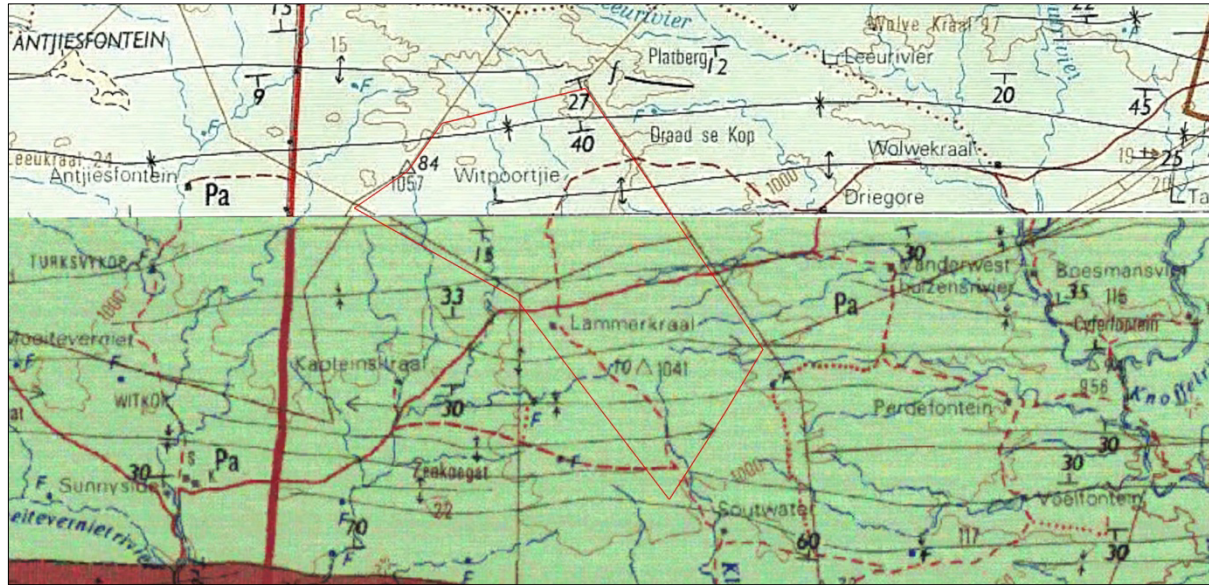
Figure 5-3 Extract from the 1:250 000 Geological Map sheets 3222 Beaufort West and 3322 Oudtshoorn
