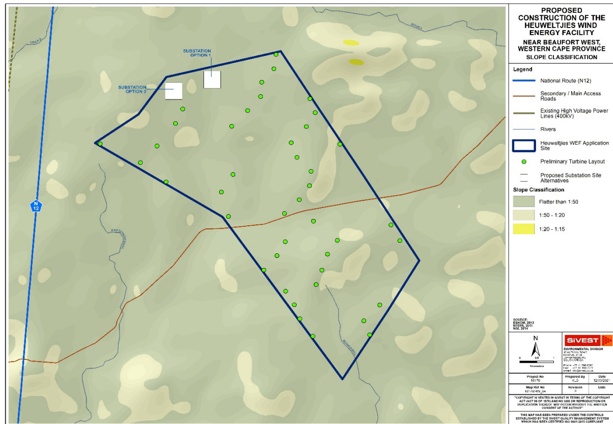
Figure 5-2 Slope classification chart of the WEF site
