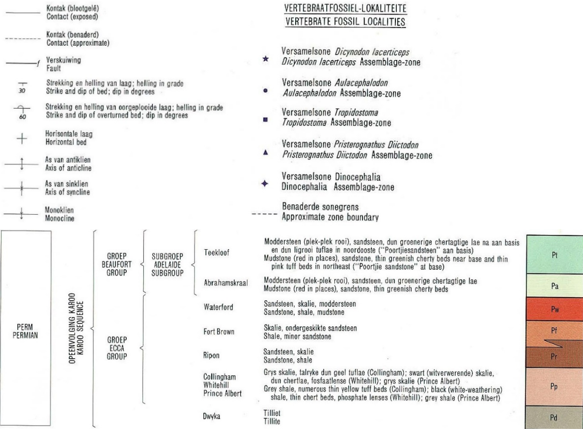
Figure 5-3 1:250 000 Geological Map Legend; Structures and Geological Sequences
