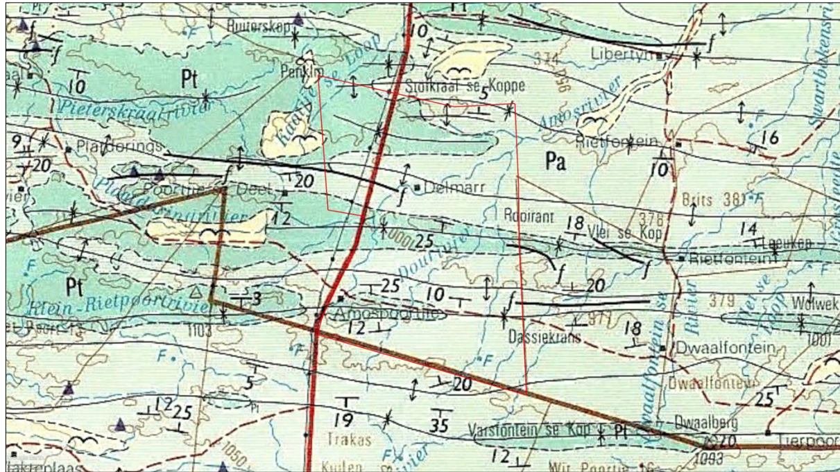
Figure 5-2 Extract from the 1:250 000 Geological Map sheets 3222 Beaufort West
