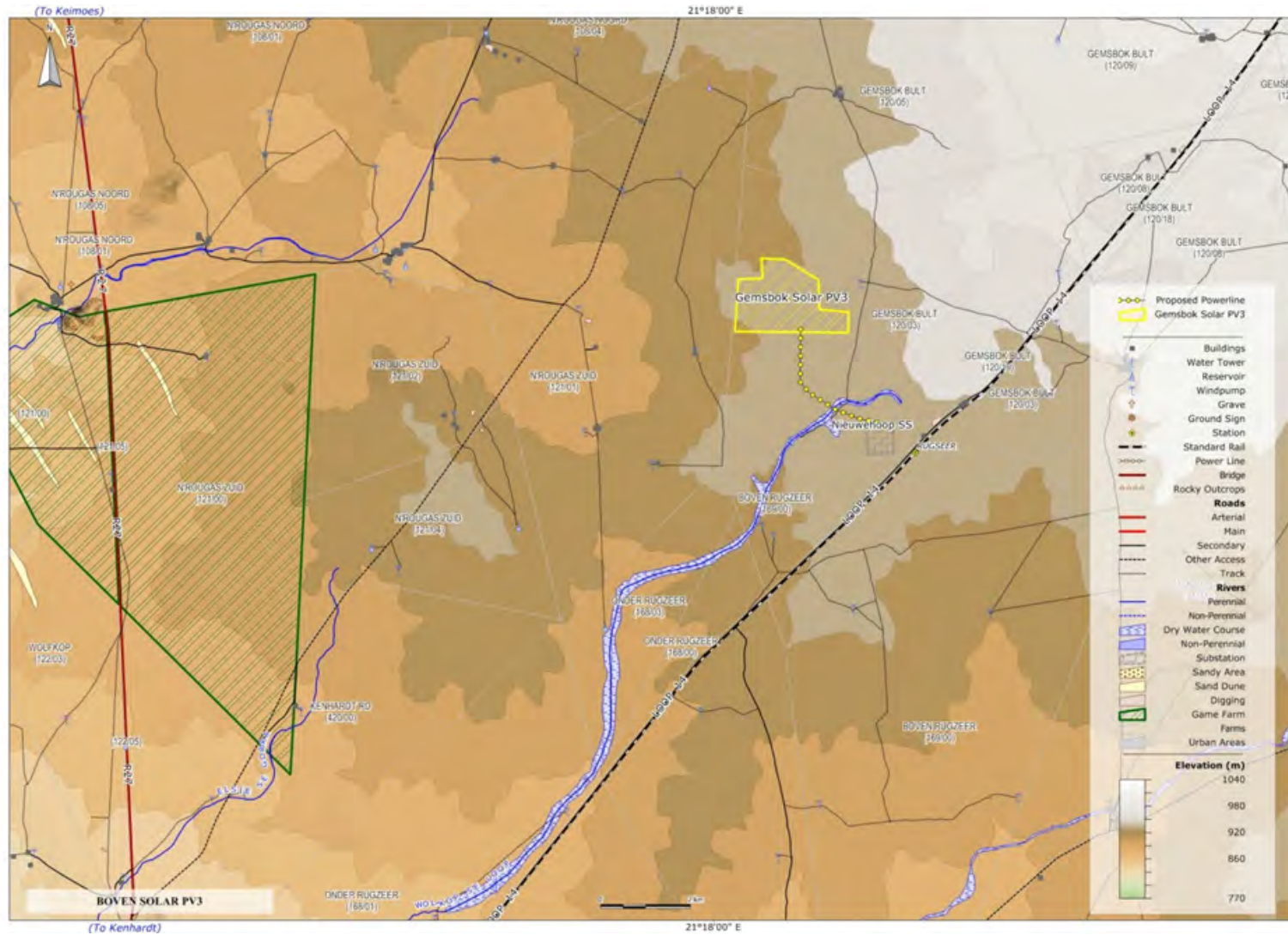
Figure 7-1: Proposed Gemsbok Solar PV3 plant site.
