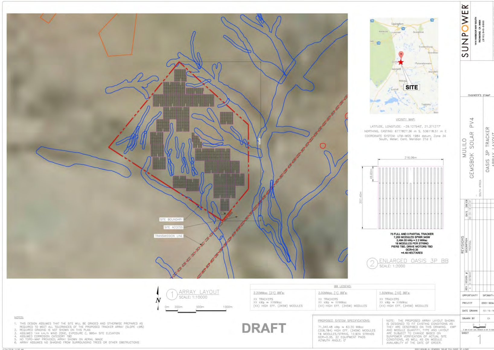
Figure 17.3: Layout for the proposed Gemsbok Solar PV4 Facility.
