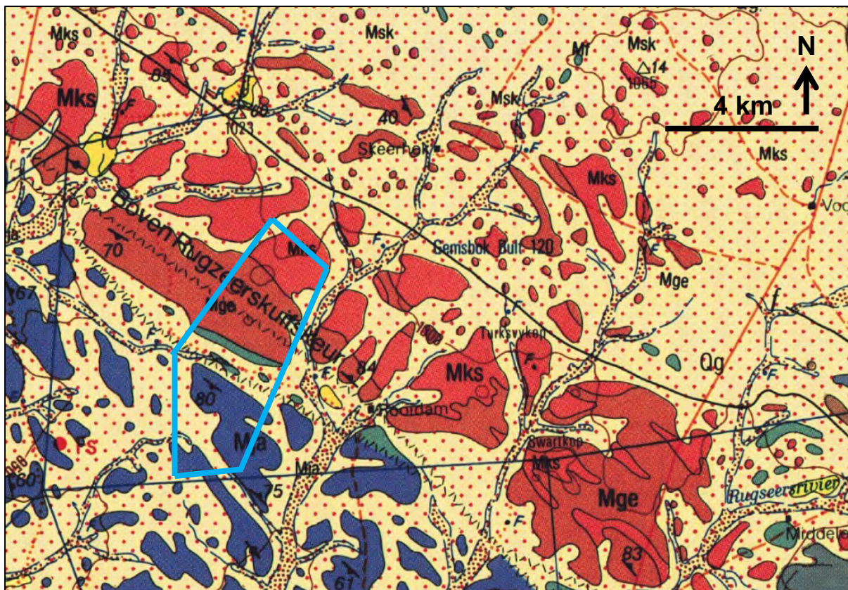
Figure 13.1: Extract from 1: 250 000 scale geological map sheet 2920 Kenhardt (Council for Geoscience, Pretoria) showing the geology of the Gemsbok Solar PV4 study area on the Portion 3 of Gemsbok Bult Farm 120, situated c. 32 km to the NE of Kenhardt, Northern Cape. The area - including the preferred and alternative sites as well as associated transmission lines - is approximately indicated by the pale blue polygon.
