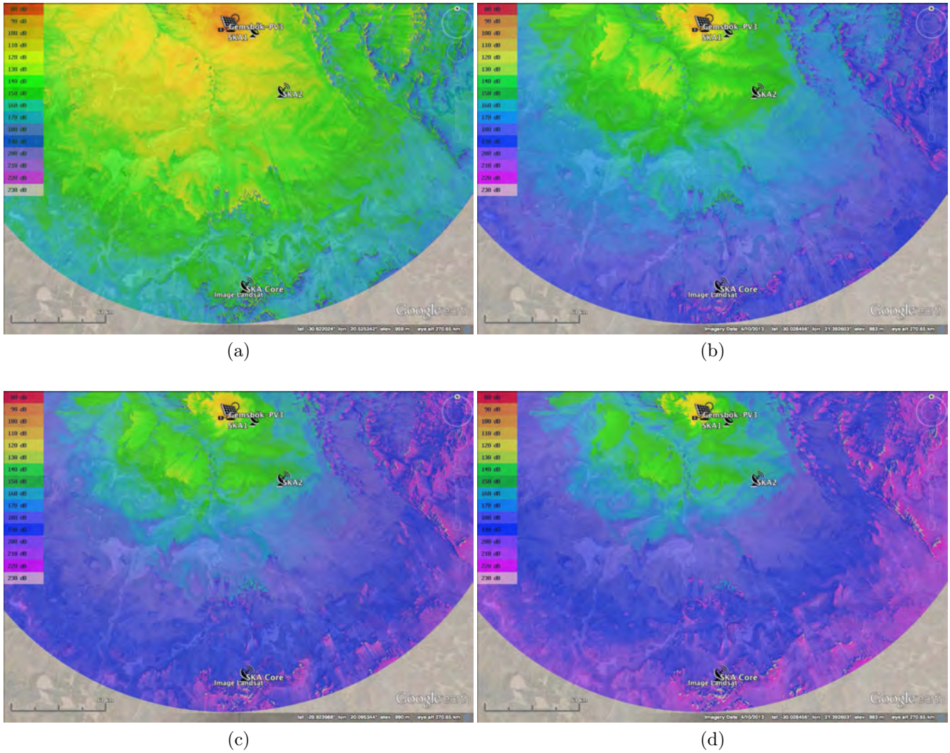
Figure 21: TPL attenuation maps for preferred site location of Gembok PV3 to the closest and core SKA telescopes for (a) 100 MHz (b) 1000 MHz (c) 2000 MHz and (d) 3000 MHz.
