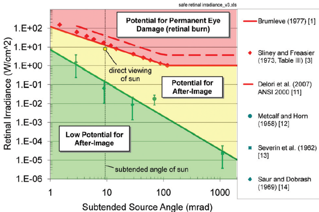
Figure 3: Solar Glare Hazard Plot [1]
