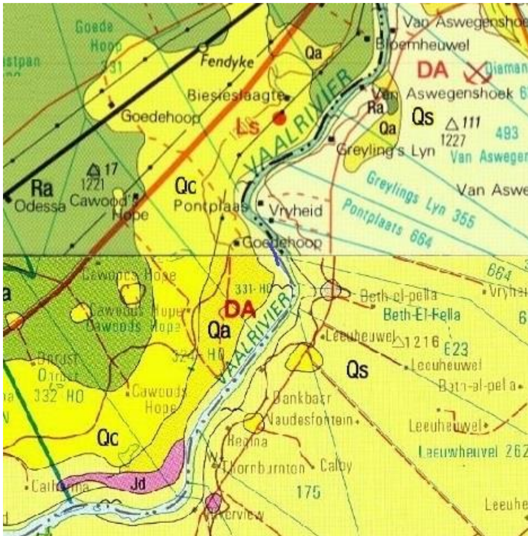
Figure 2: Geological map of the study area and surroundings (adapted from the 2824 Kimberley (lower part) and the 2724 Christiana (upper part) 1:250 000 geology maps (Council for Geoscience; 1993, 1994))
