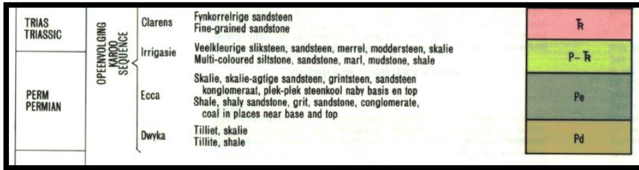
Figure 4: Lithostratigraphic column of the development area (Walraven 1981).
