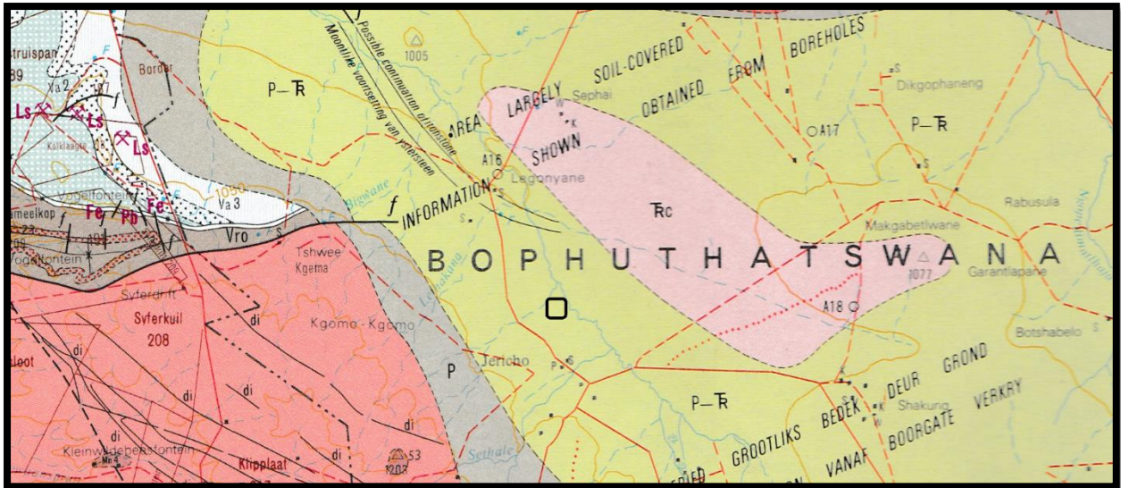
Figure 3: Geology of the development area (1h).
