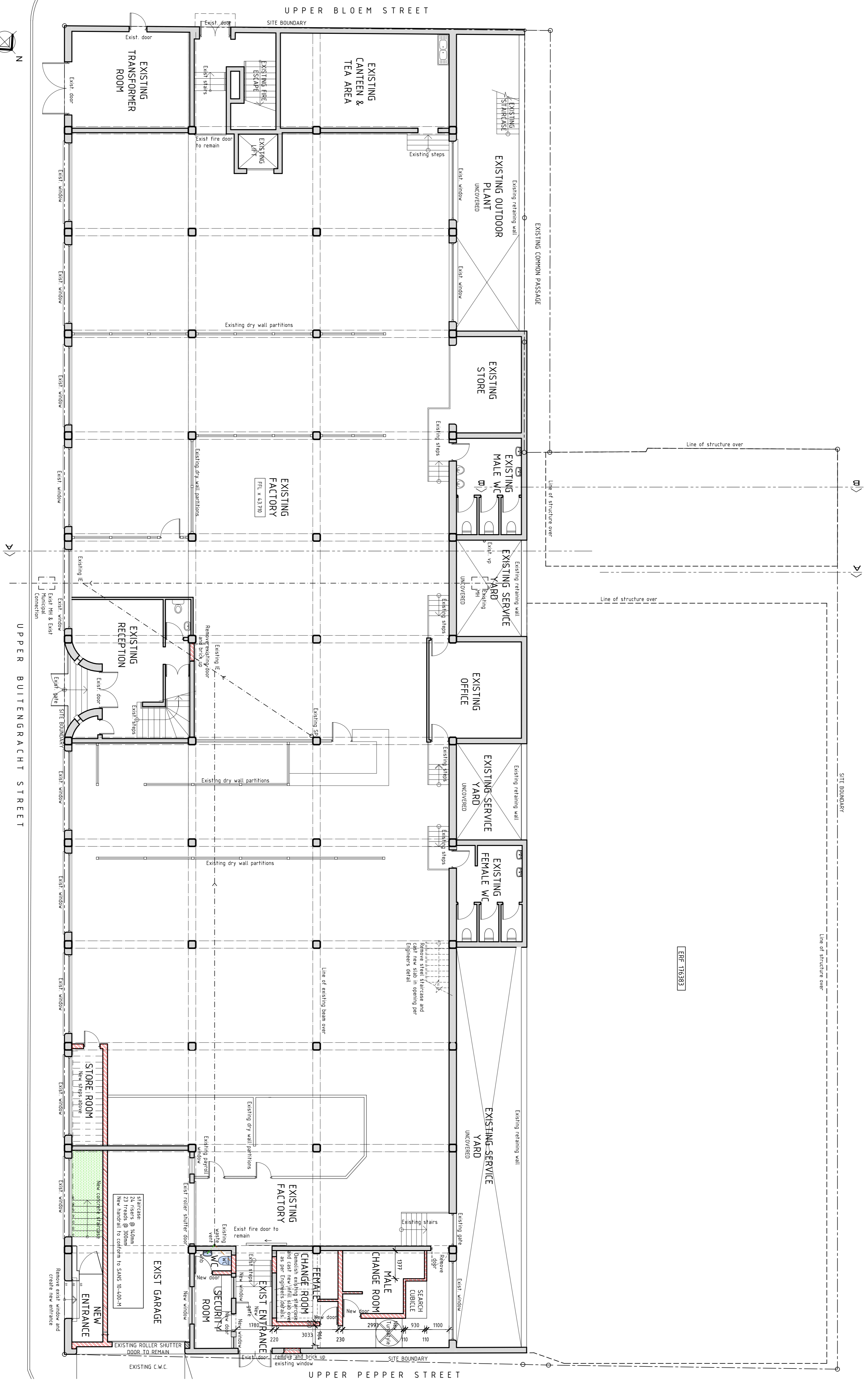
GROUND STOREY PLAN SCALE 1:100
