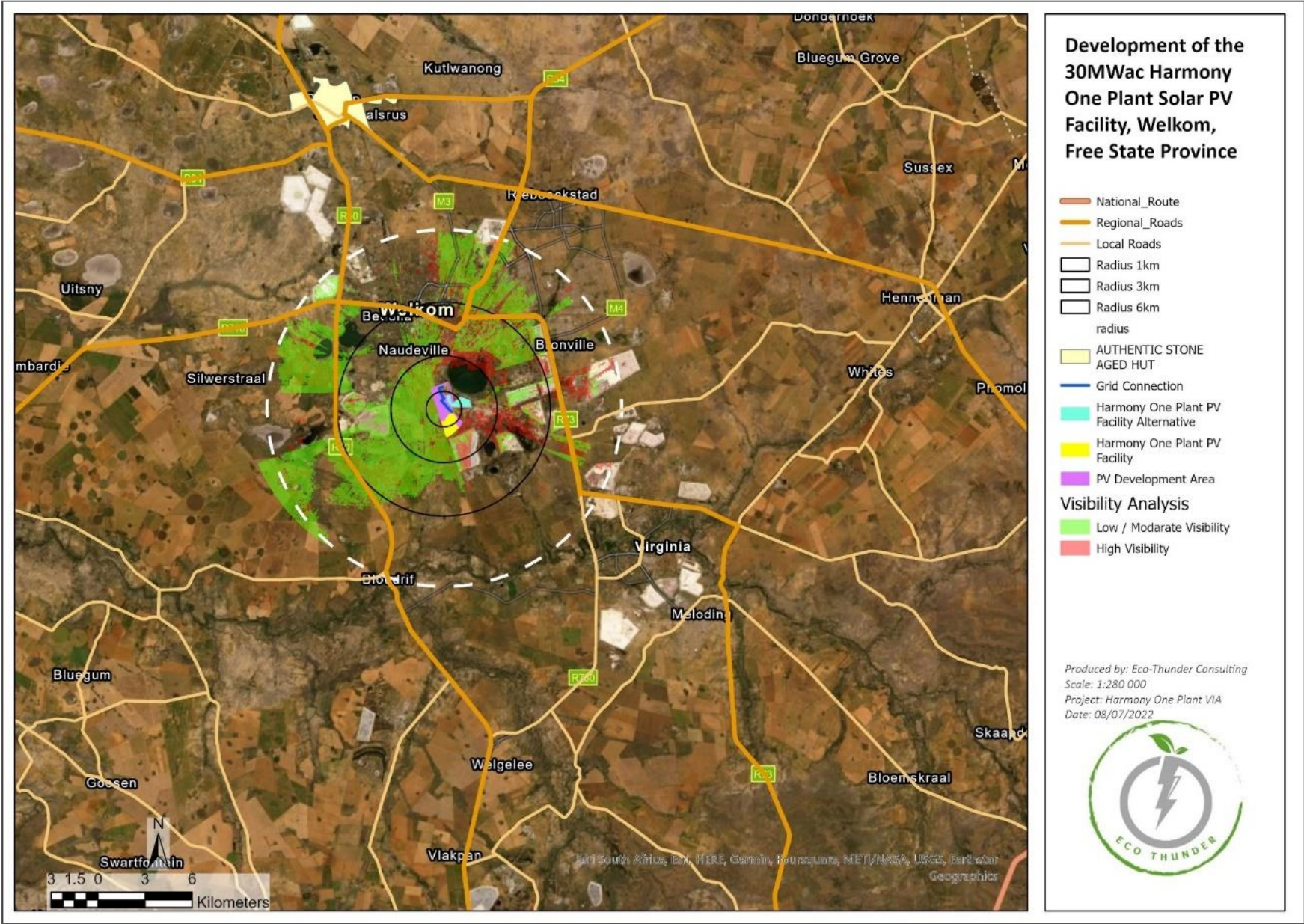
Figure 21: Viewshed analysis
