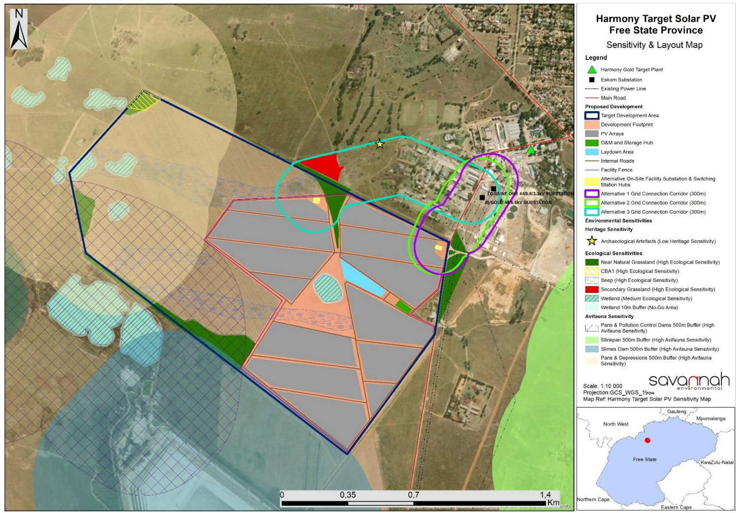
Figure 1: Layout and sensitivity map of the development footprint and grid connection corridor for the 30 MW Harmony Target Solar PV Facility, as was assessed as part of the EIA process.
