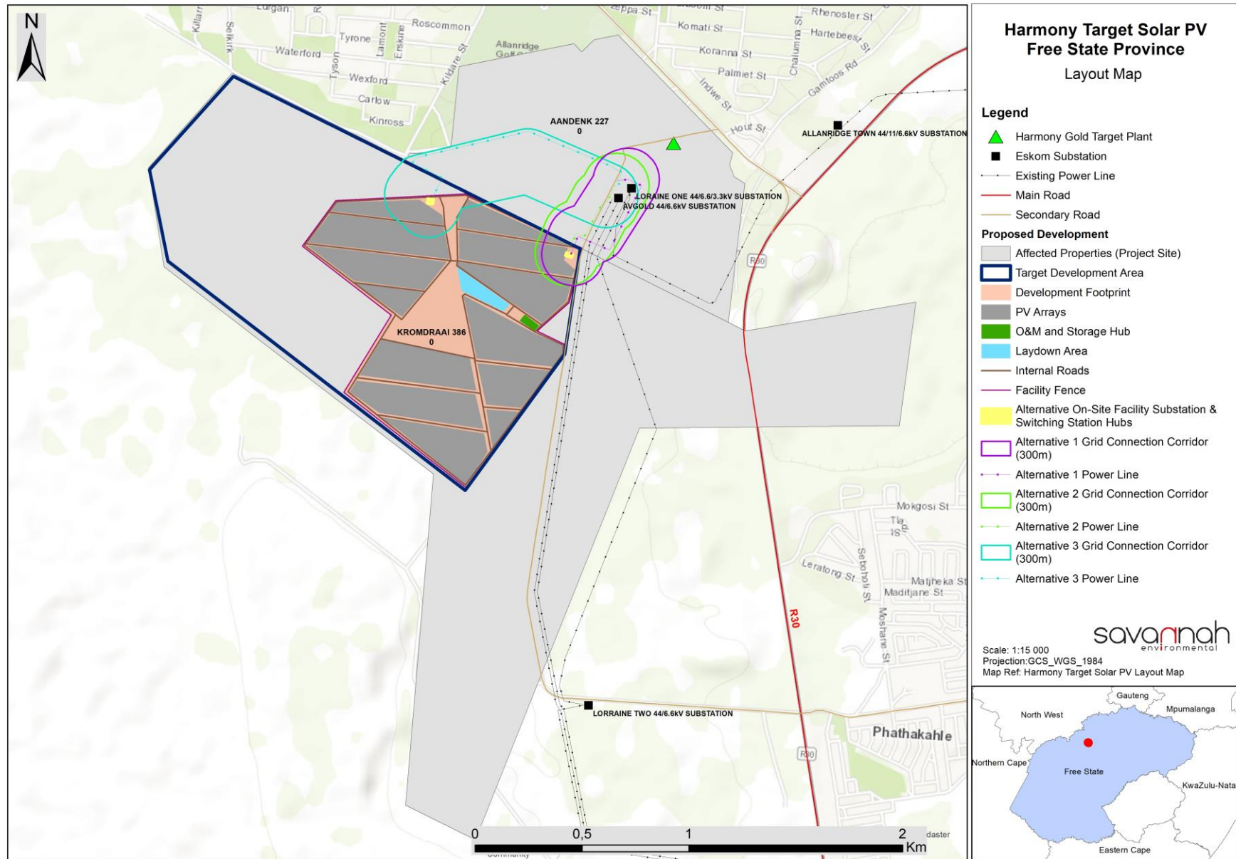
Figure 2.2: The layout of the Harmony Target Solar PV Facility, as assessed within the EIA Report
