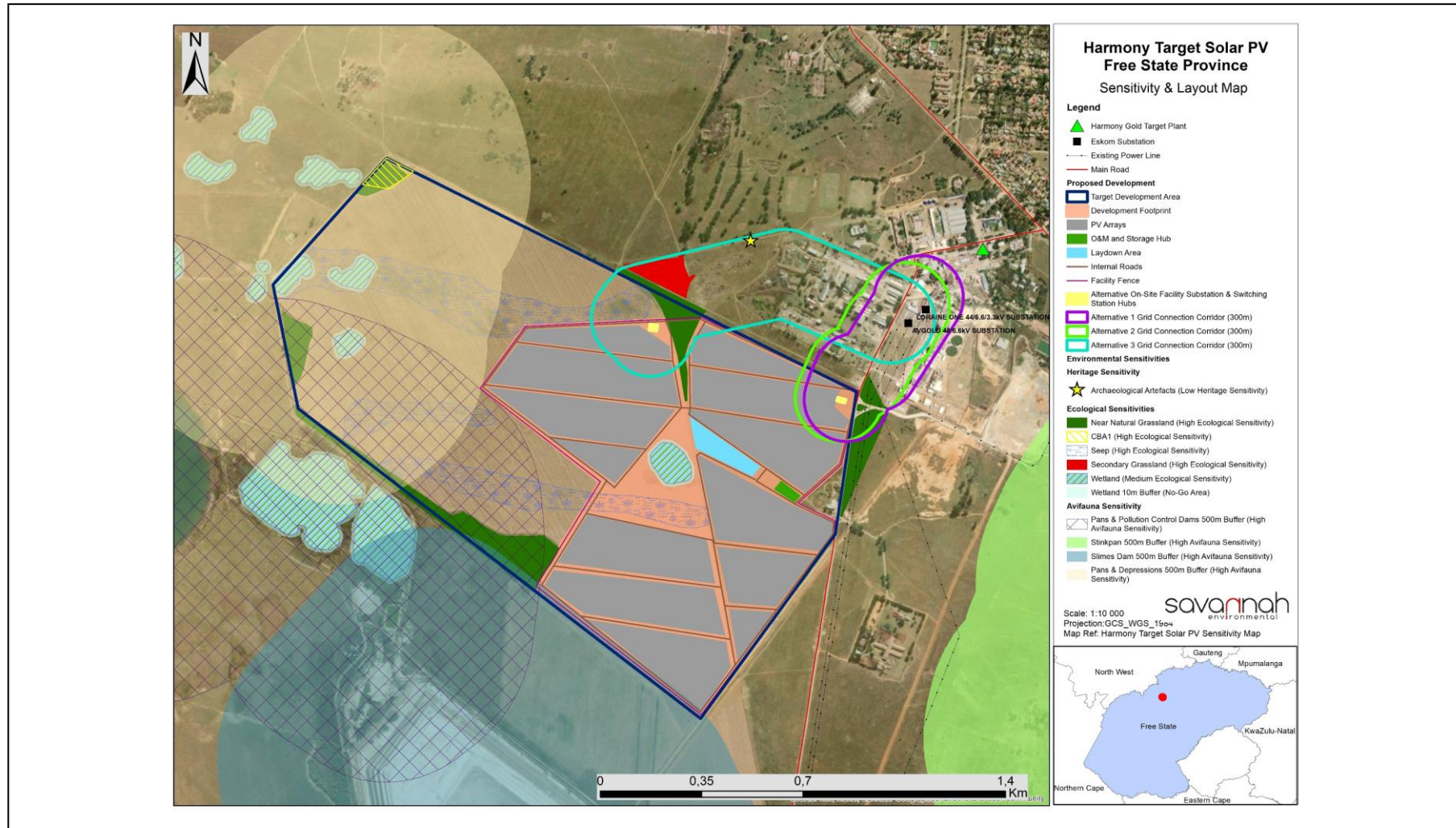
Figure 1: Layout and sensitivity map of the development footprint and grid connection corridor for the 30MW Harmony Target Solar PV Facility, as was assessed as part of the BA process
