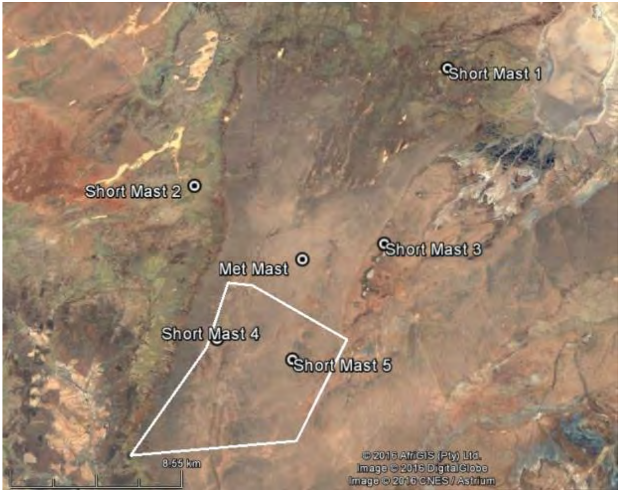
Figure 2: Overview of the passive monitoring systems on the Hartebeestlegte WEF.
