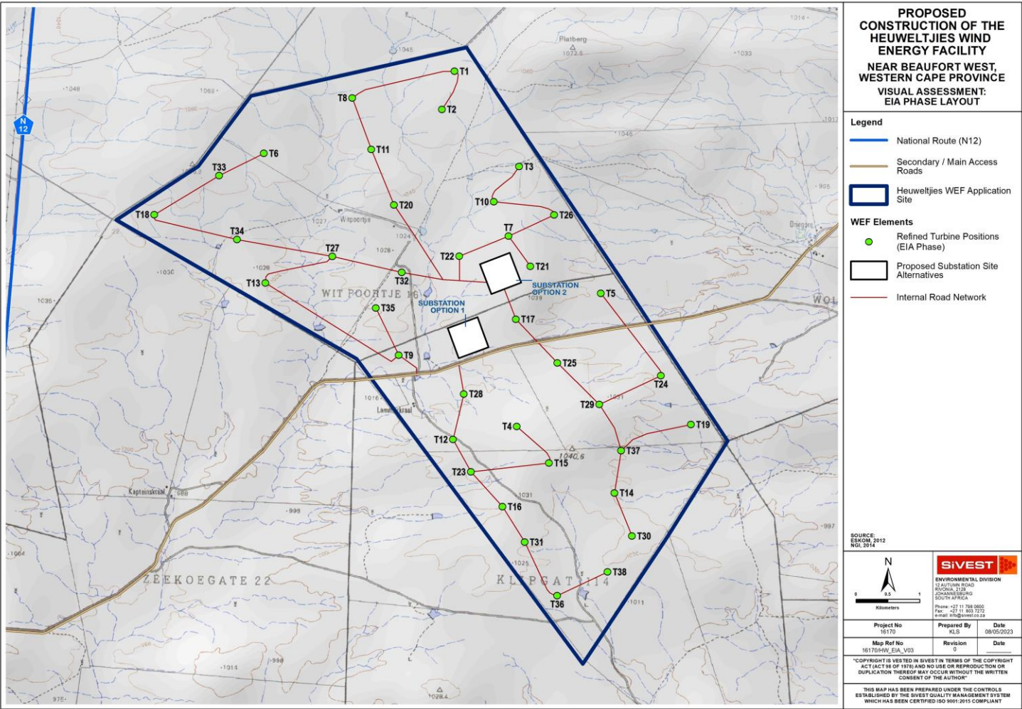
Figure 4: Preliminary Heuweltjies WEF layout
