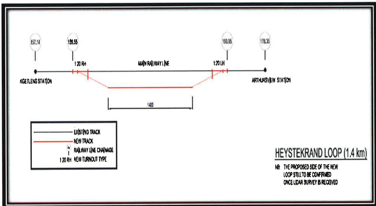
Figure 2: Diagrammatic layout for the existing line and the proposed loop
