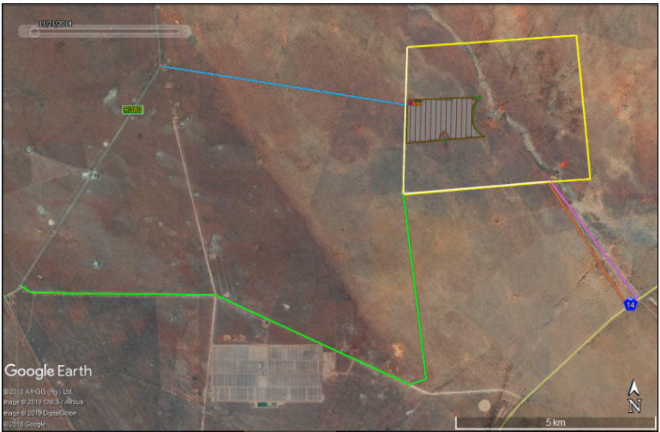
Figure 2: Aerial view of the broader study area showing the project site (yellow polygon), proposed HSD2 development area (grey hatched area), four access road alternatives (See Fig. 1 for labels) and the proposed perimeter access road (white line along western and southern margins of the site).
