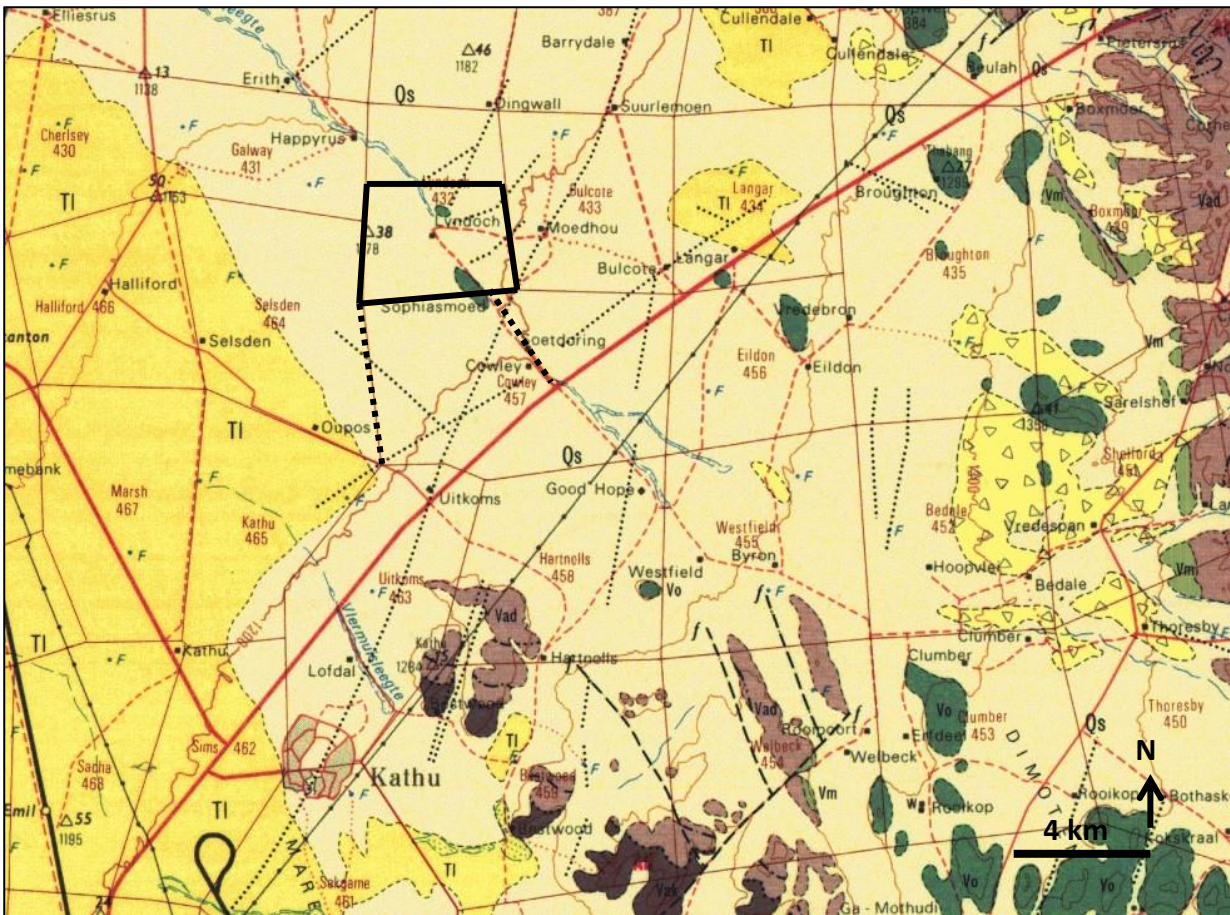
Figure 2. Extract from 1: 250 000 geological map 2722 Kuruman (Council for Geoscience, Pretoria) showing the location of the project site on the Remainder of the Farm Lyndoch 432 to the NW of the N14 near Kathu, Northern Cape (black polygon) together with access road alternatives (black dotted lines). Note that the road and railway networks shown here are out of date.
