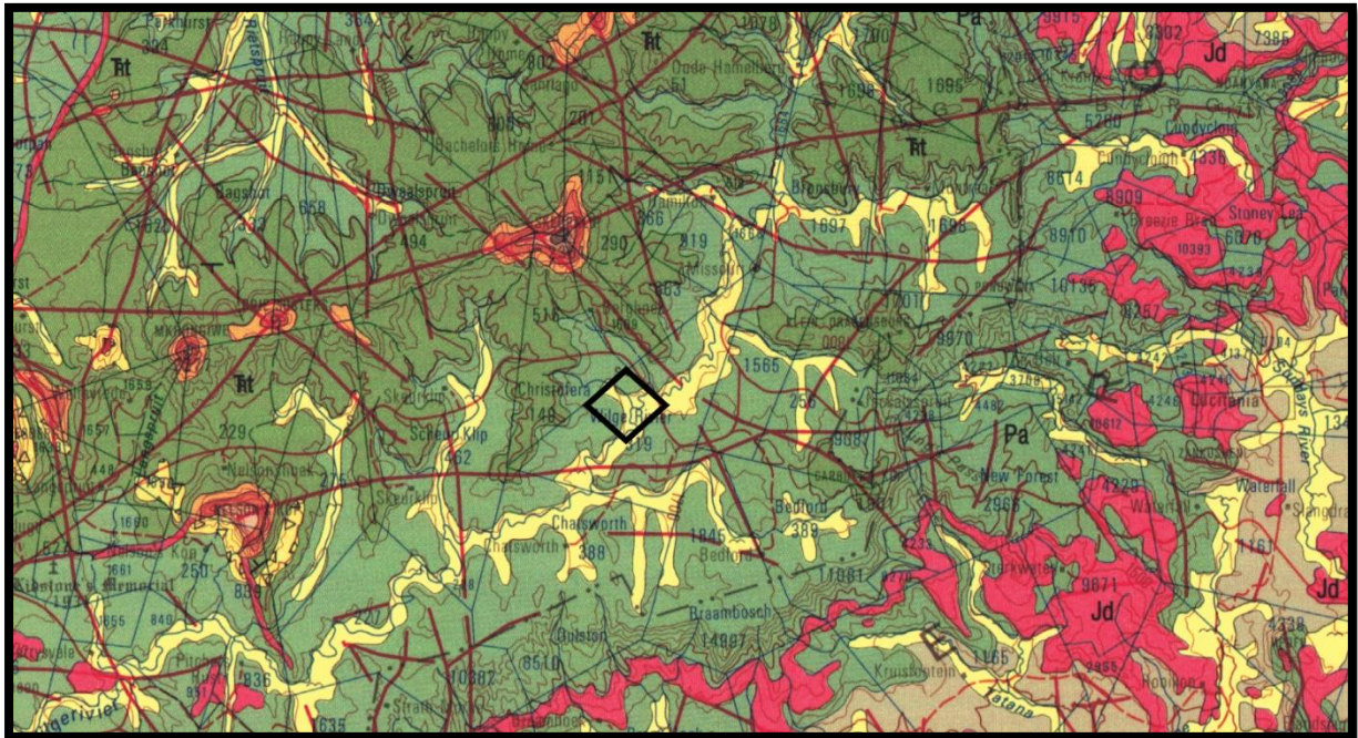
Figure 3: Geology of the development area (Verster 1998) (1h).
