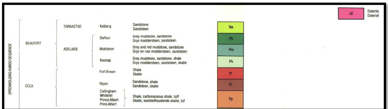
Figure 5: Lithostratigraphic column of the Karoo Supergroup (Johnson 1976)
