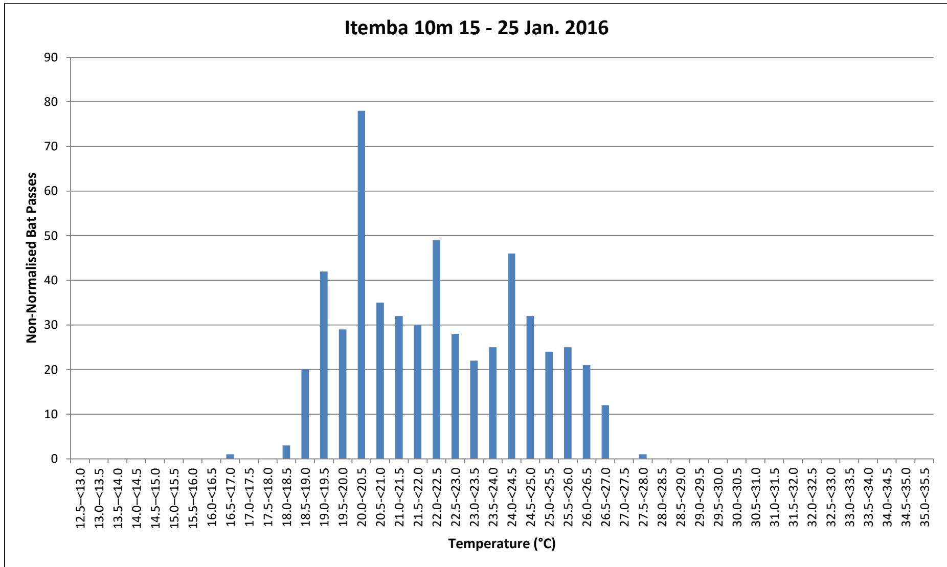
Figure 57: Sum of bat passes (Non-normalised) per Temperature category for Itemba 10m (15 – 25 January 2016).
