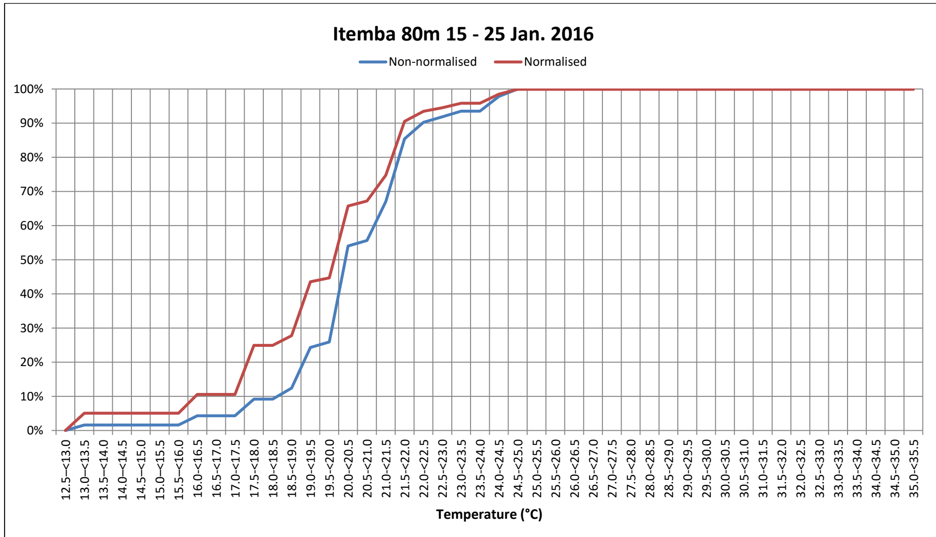
Figure 64: Cumulative percentage of normalised and non-normalised bat passes per Temperature category for Itemba 80m (15 – 25 January 2016).
