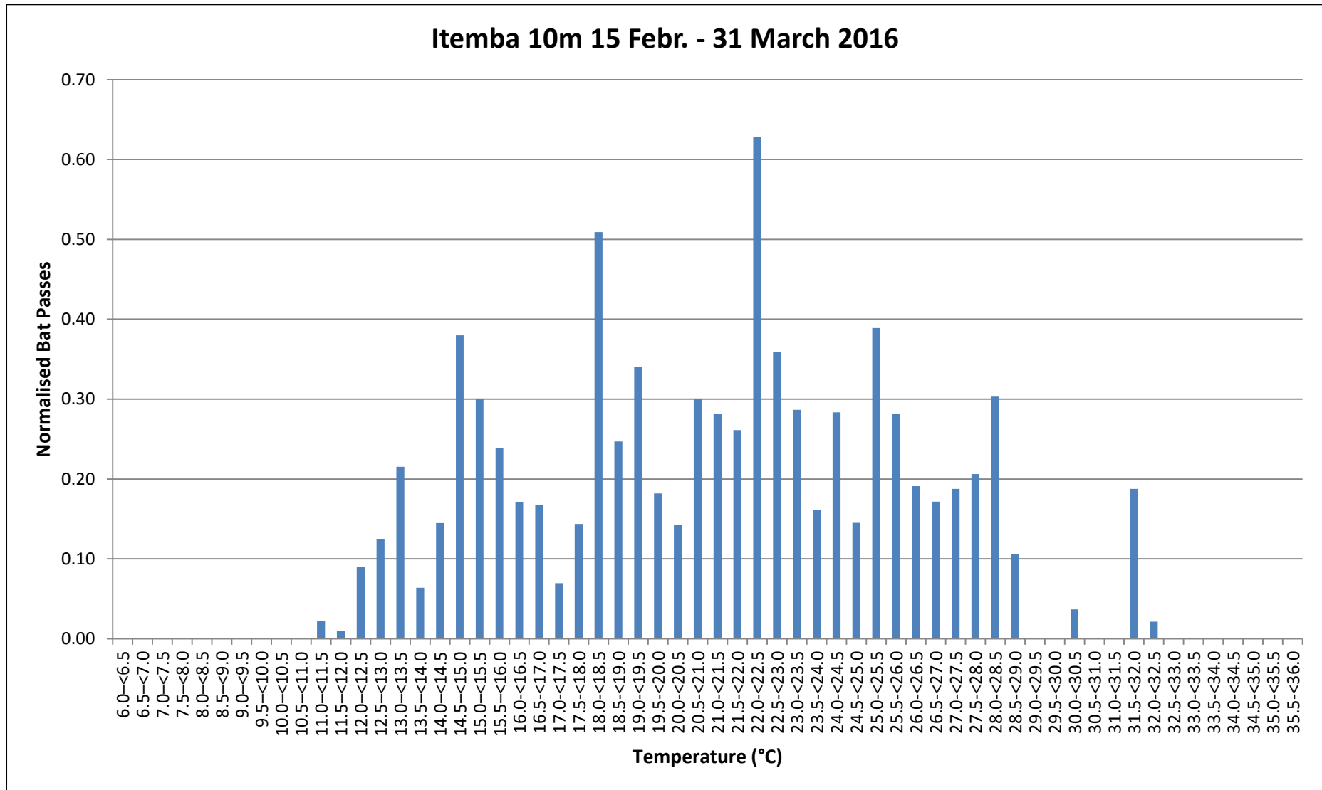
Figure 68: Sum of bat passes (Normalised) per Temperature category for Itemba 10m (15 February – 31 March 2016).
