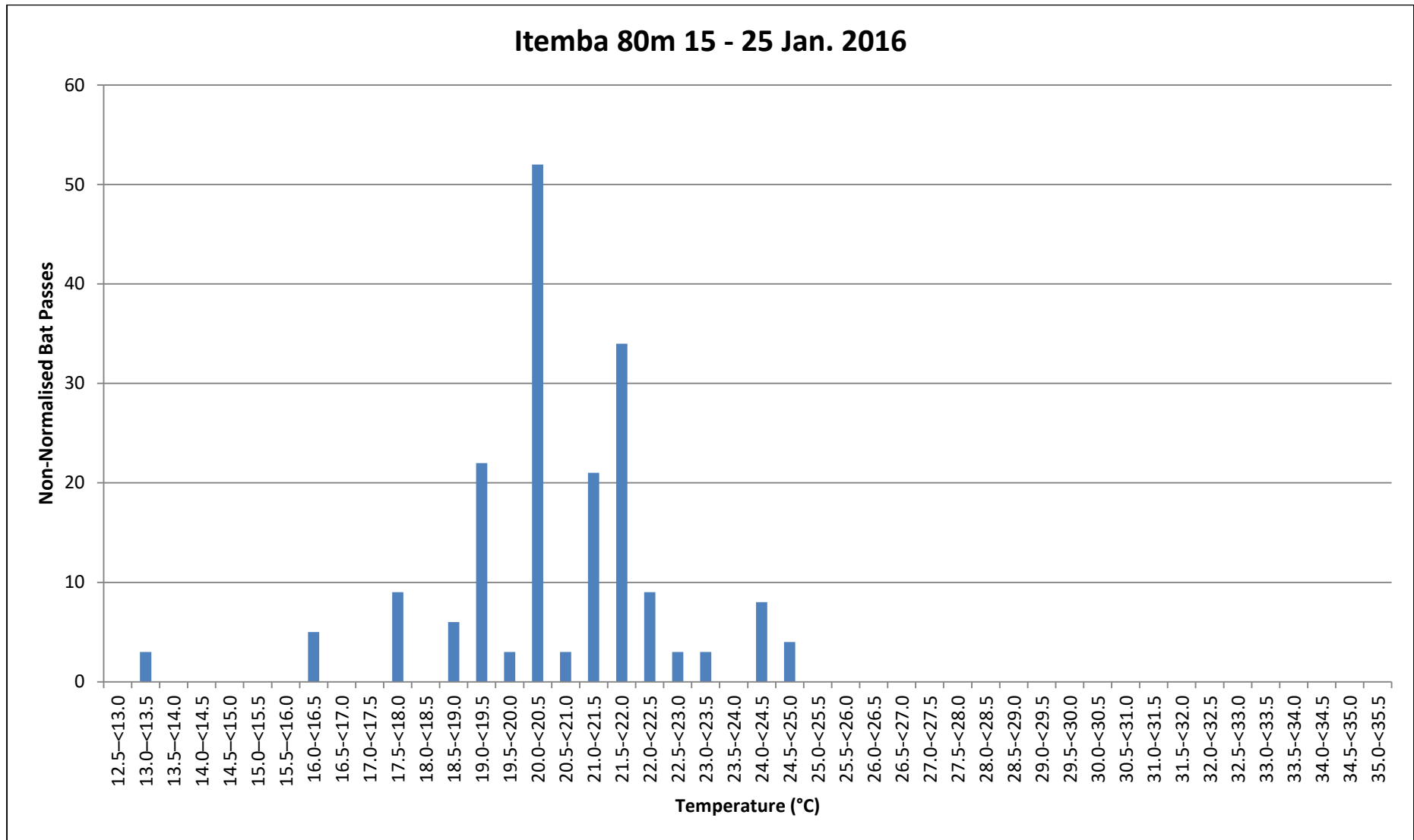
Figure 63: Sum of bat passes (Non-normalised) per Temperature category for Itemba 80m (15 – 25 January 2016).
