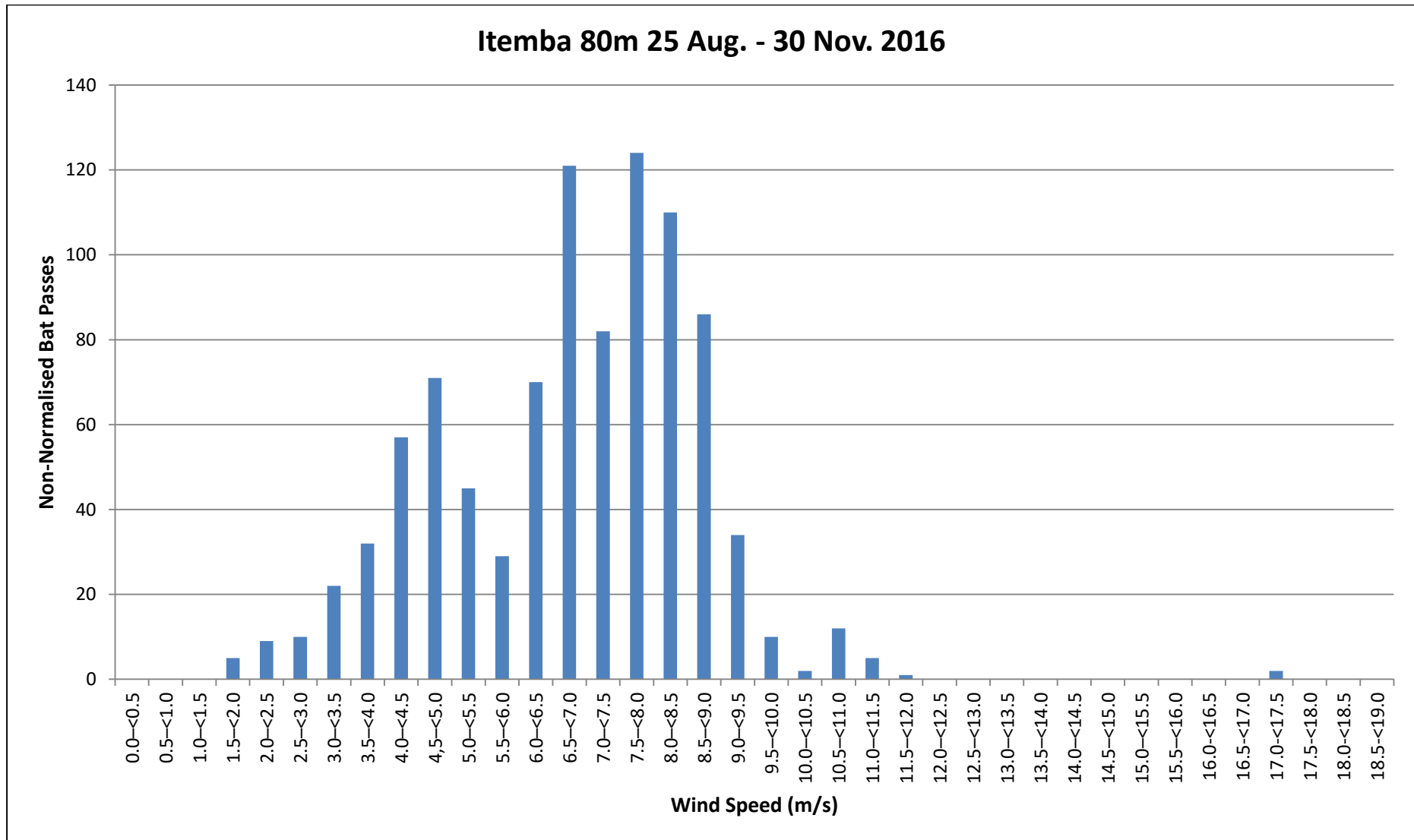
Figure 90: Sum of bat passes (Non-normalised) per Wind Speed category for Itemba 80m (25 August – 30 November 2016).
