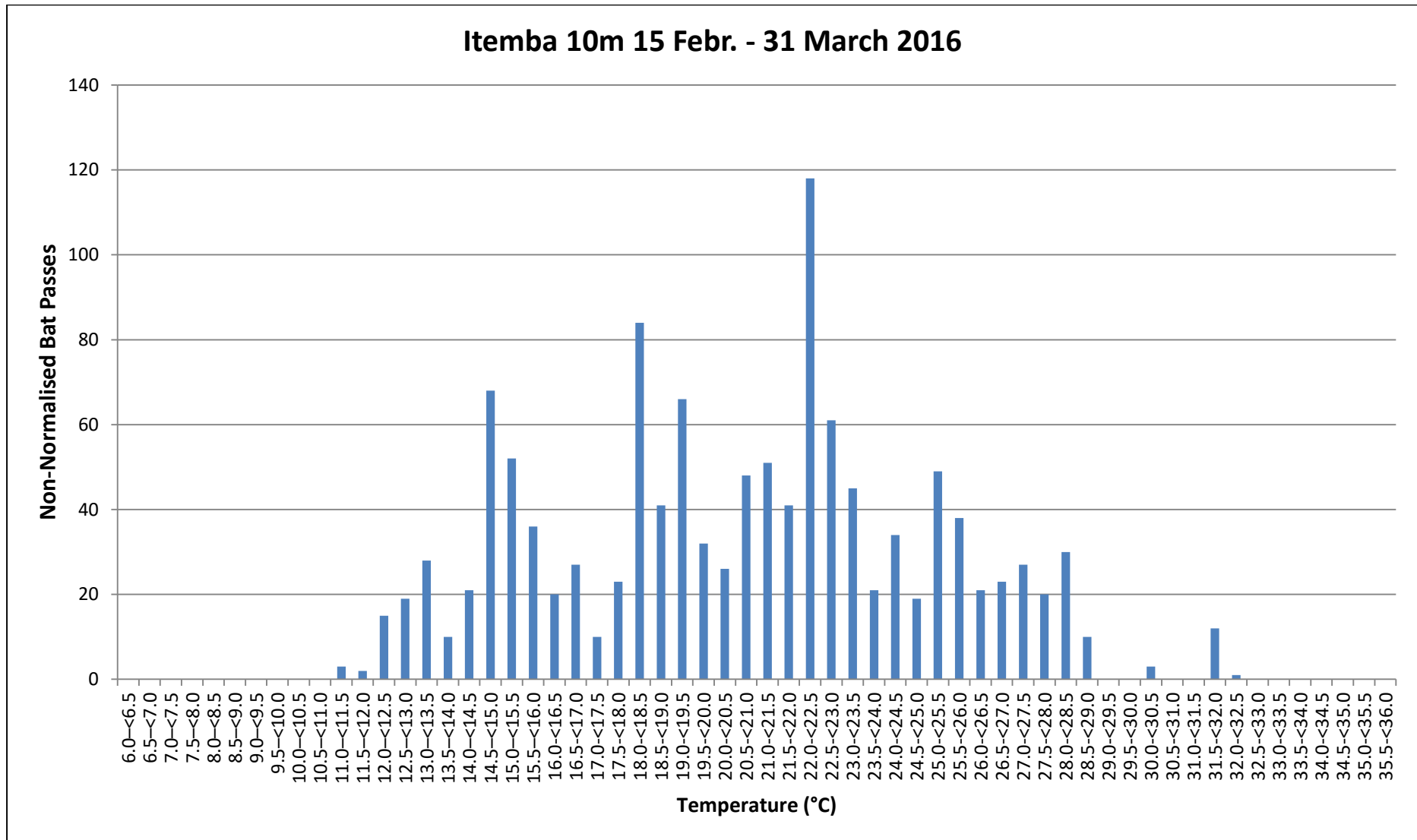
Figure 69: Sum of bat passes (Non-normalised) per Temperature category for Itemba 10m (15 February – 31 March 2016).
