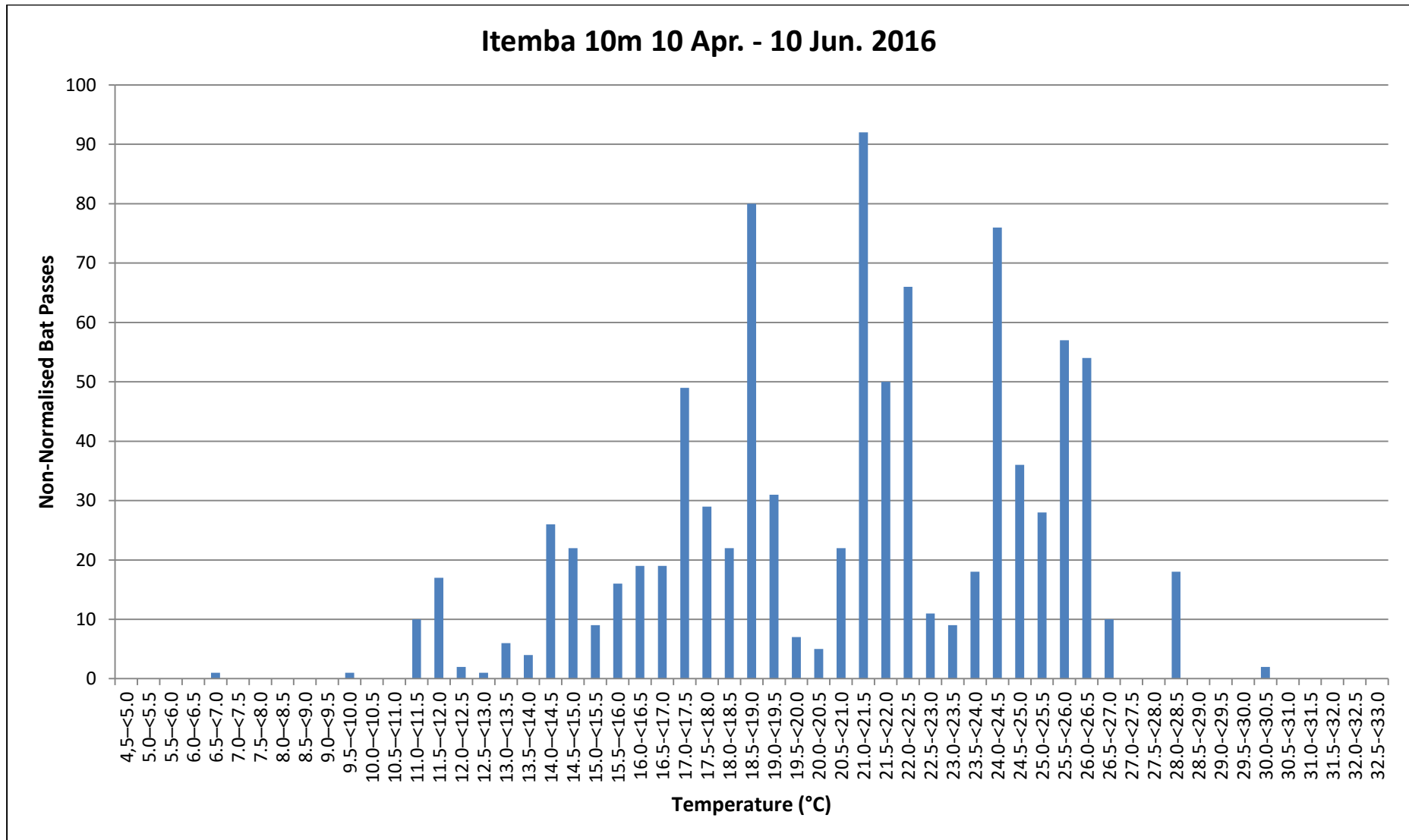
Figure 75: Sum of bat passes (Non-normalised) per Temperature category for Itemba 10m (10 April – 10 June 2016).
