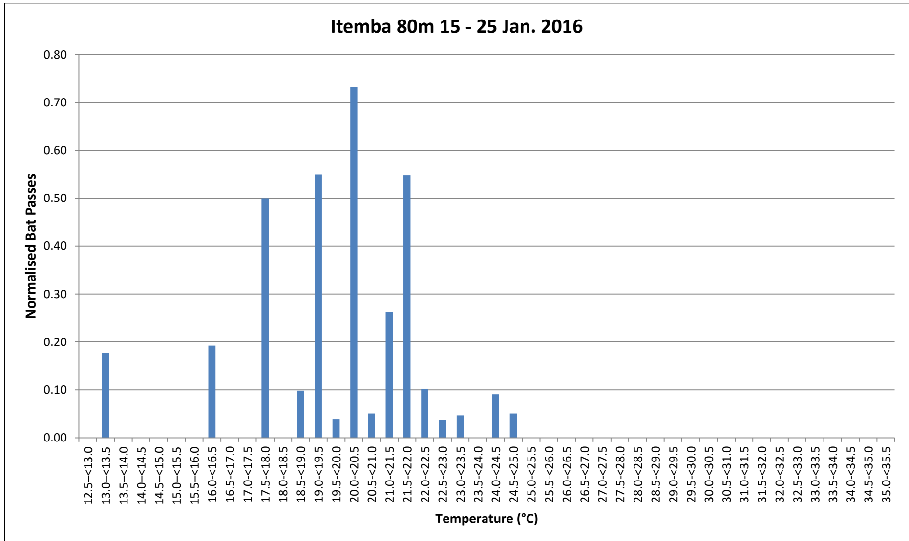
Figure 62: Sum of bat passes (Normalised) per Temperature category for Itemba 80m (15 – 25 January 2016).
