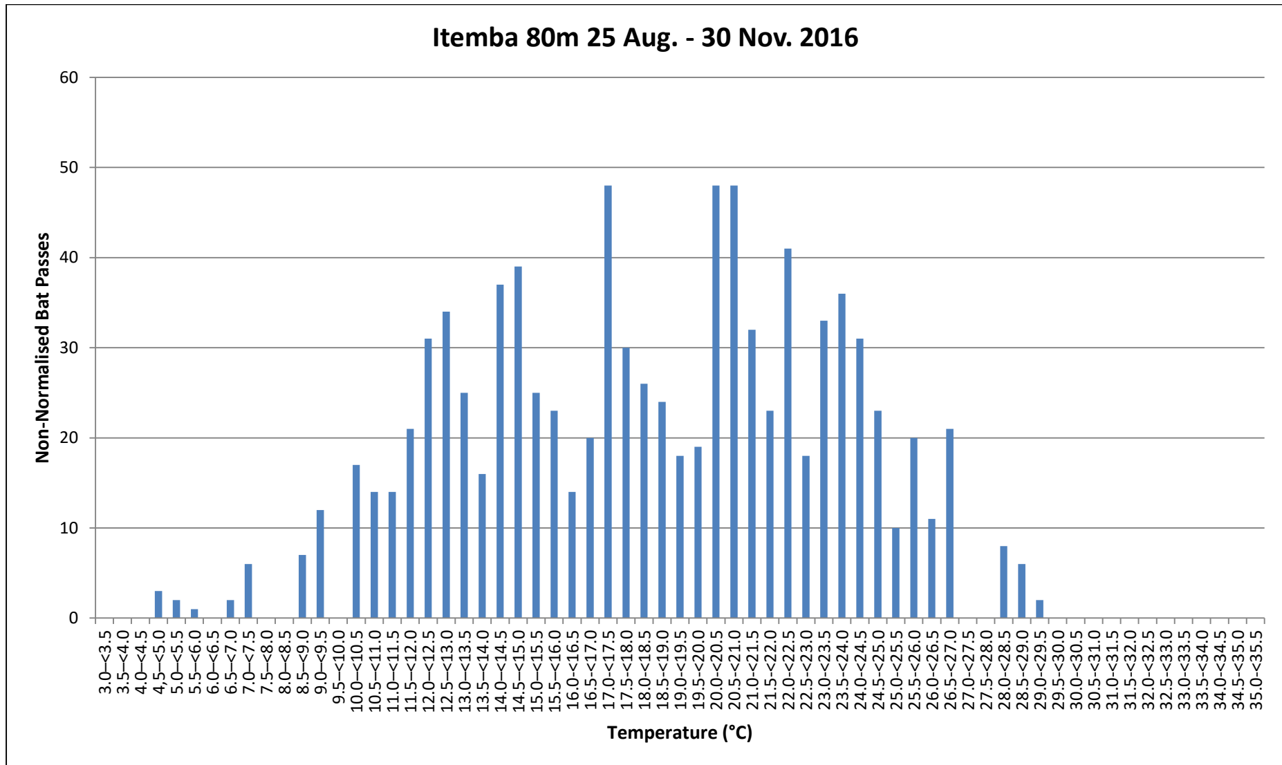
Figure 87: Sum of bat passes (Non-normalised) per Temperature category for Itemba 80m (25 August – 30 November 2016).
