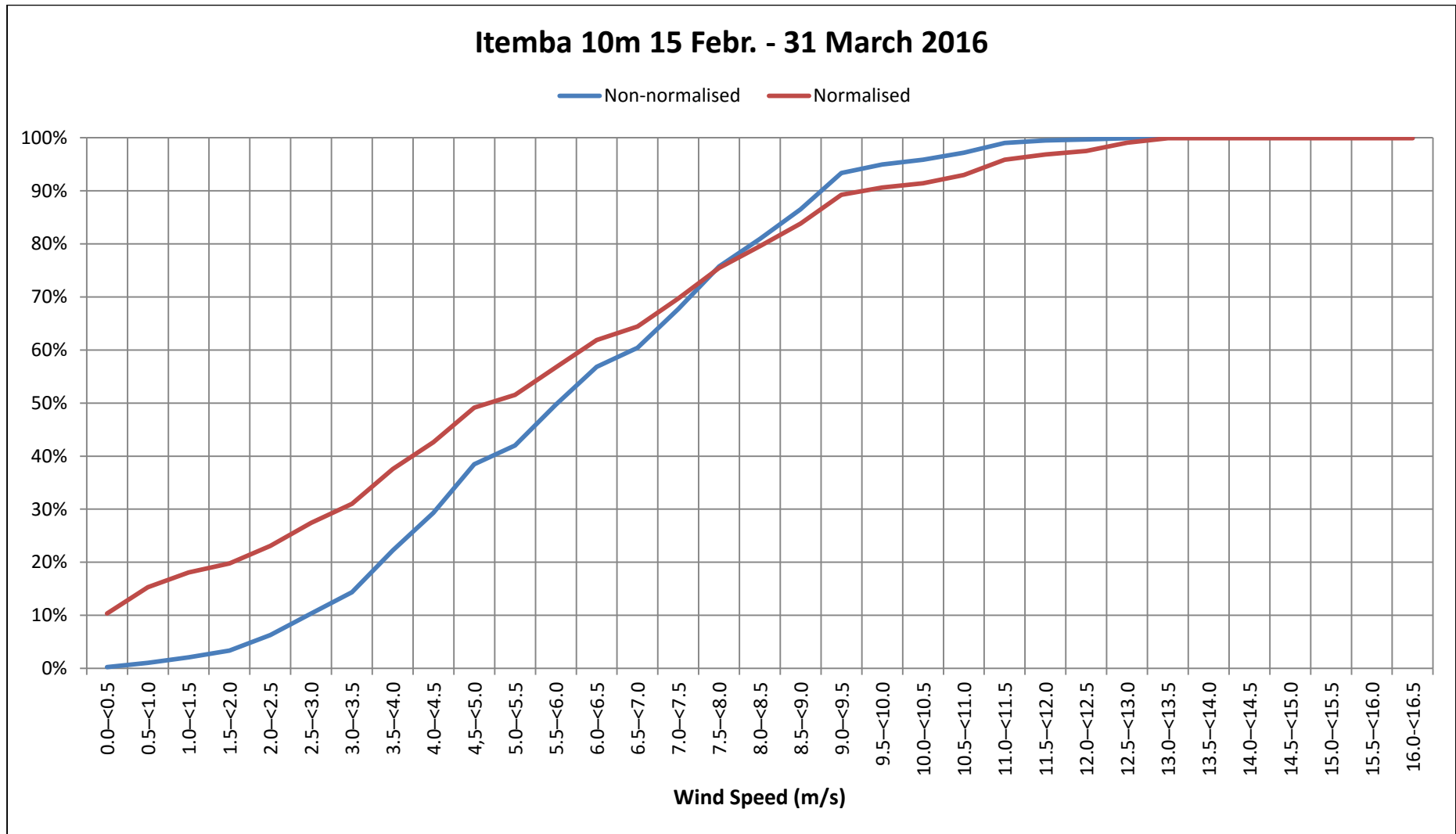
Figure 73: Cumulative percentage of normalised and non-normalised bat passes per Wind Speed category for Itemba 10m (15 February – 31 March 2016).
