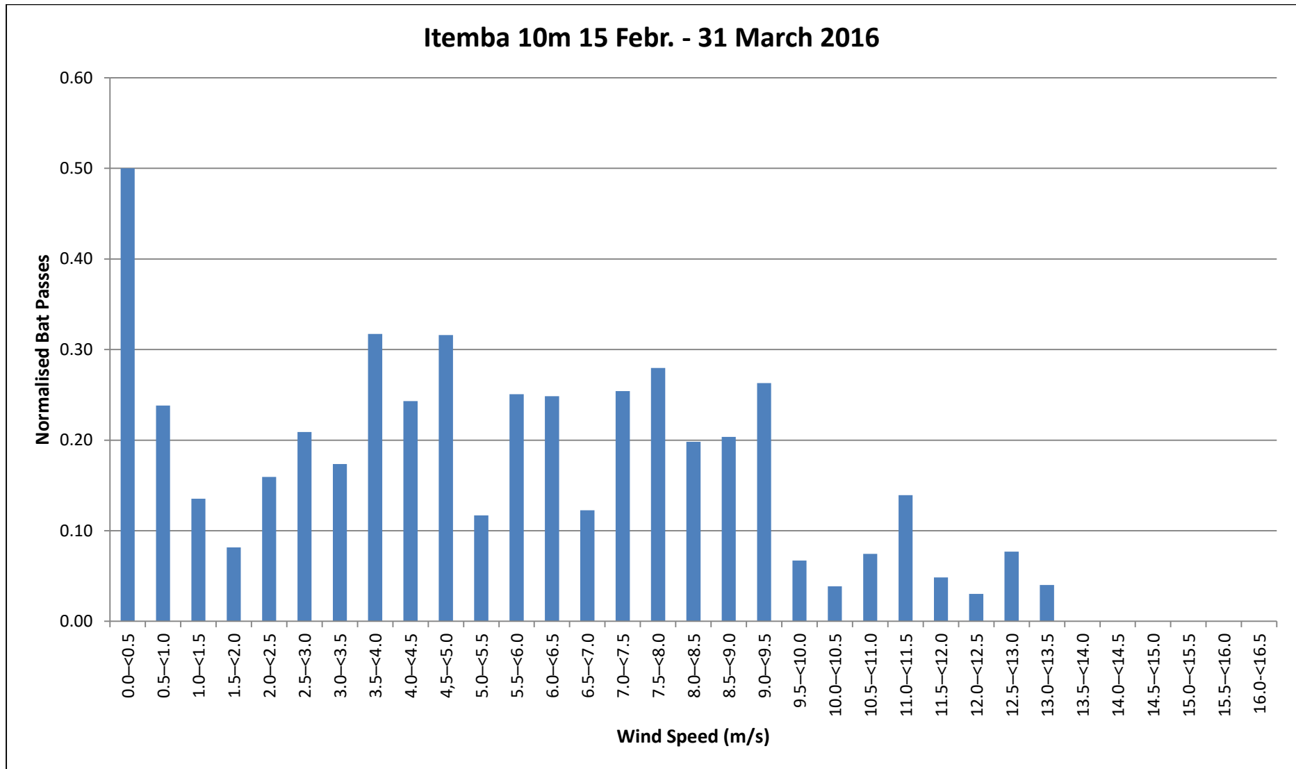
Figure 71: Sum of bat passes (Normalised) per Wind Speed category for Itemba 10m (15 February – 31 March 2016).
