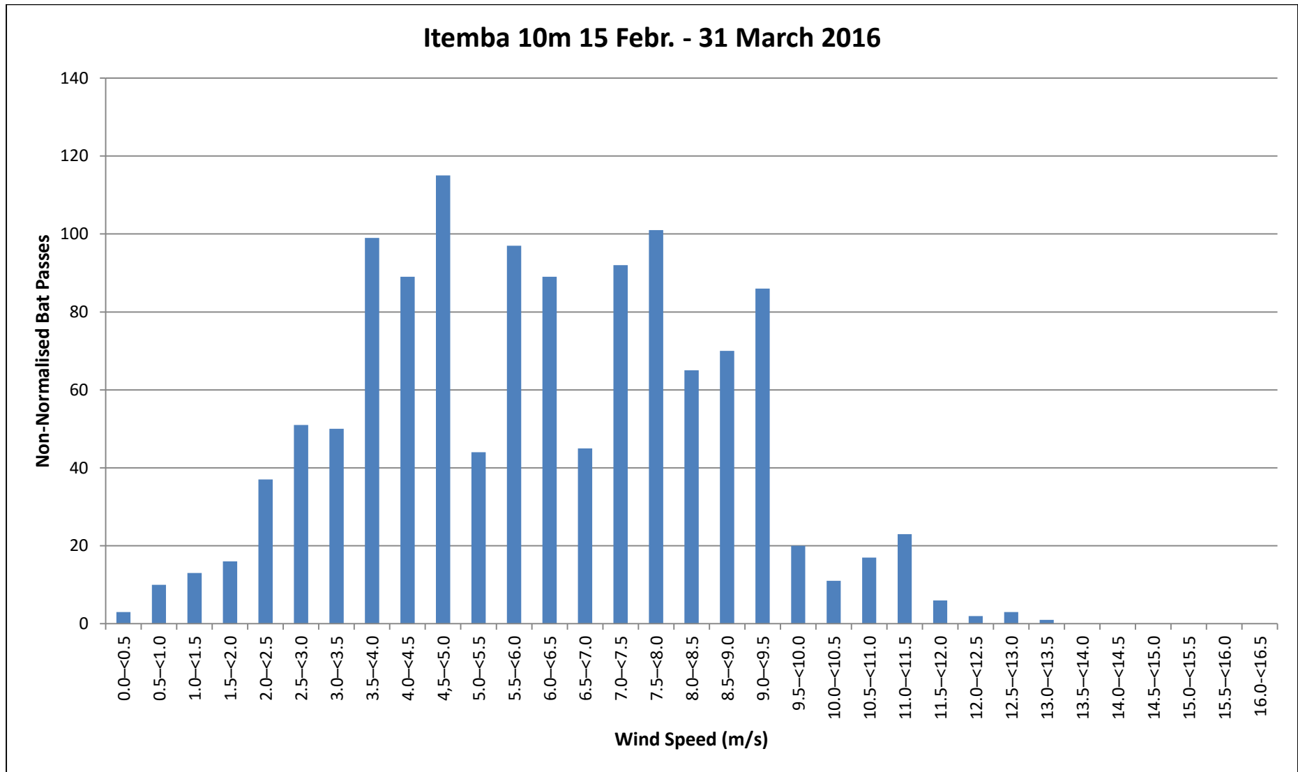
Figure 72: Sum of bat passes (Non-normalised) per Wind Speed category for Itemba 10m (15 February – 31 March 2016).
