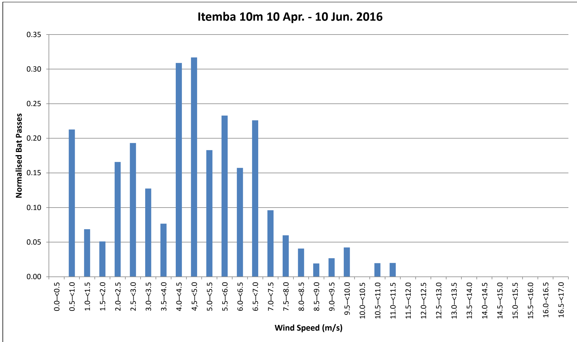
Figure 77: Sum of bat passes (Normalised) per Wind Speed category for Itemba 10m (10 April – 10 June 2016).
