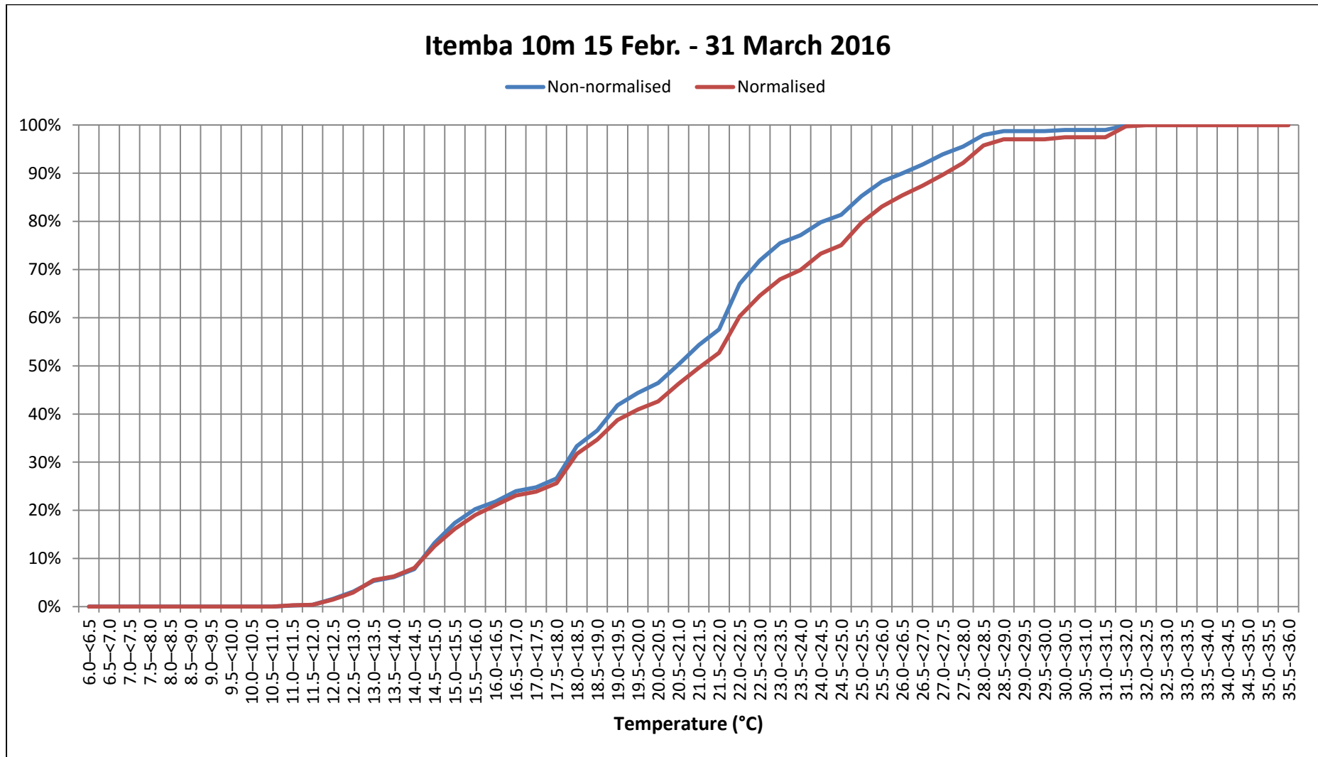
Figure 70: Cumulative percentage of normalised and non-normalised bat passes per Temperature category for Itemba 10m (15 February – 31 March 2016).
