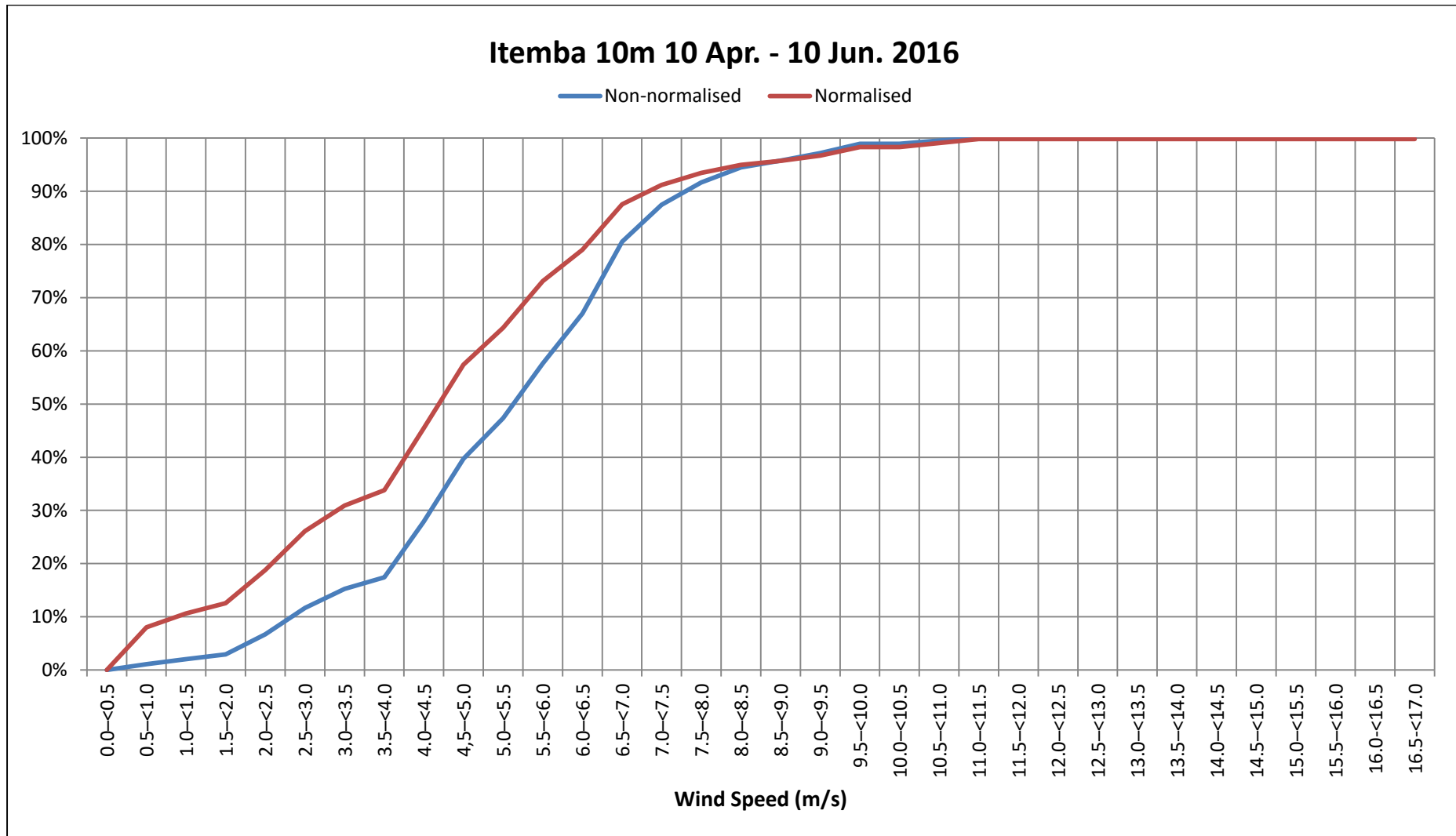
Figure 79: Cumulative percentage of normalised and non-normalised bat passes per Wind Speed category for Itemba 10m (10 April – 10 June 2016).
