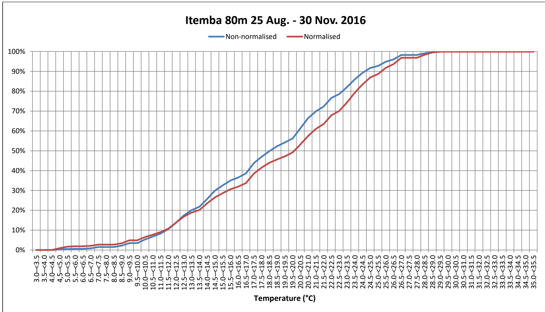
Figure 88: Cumulative percentage of normalised and non-normalised bat passes per Temperature category for Itemba 80m (25 August – 30 November 2016).
