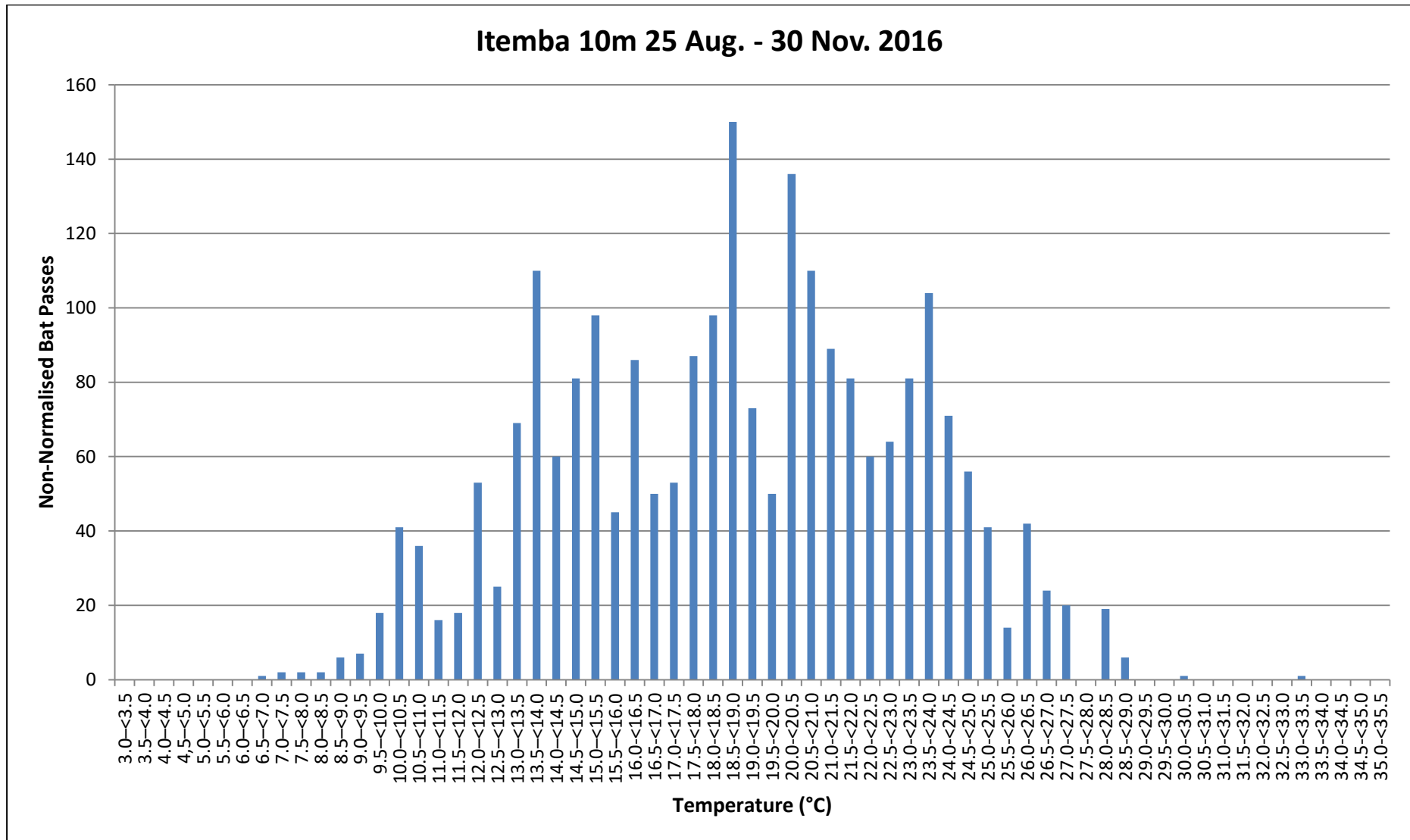
Figure 81: Sum of bat passes (Non-normalised) per Temperature category for Itemba 10m (25 August – 30 November 2016).
