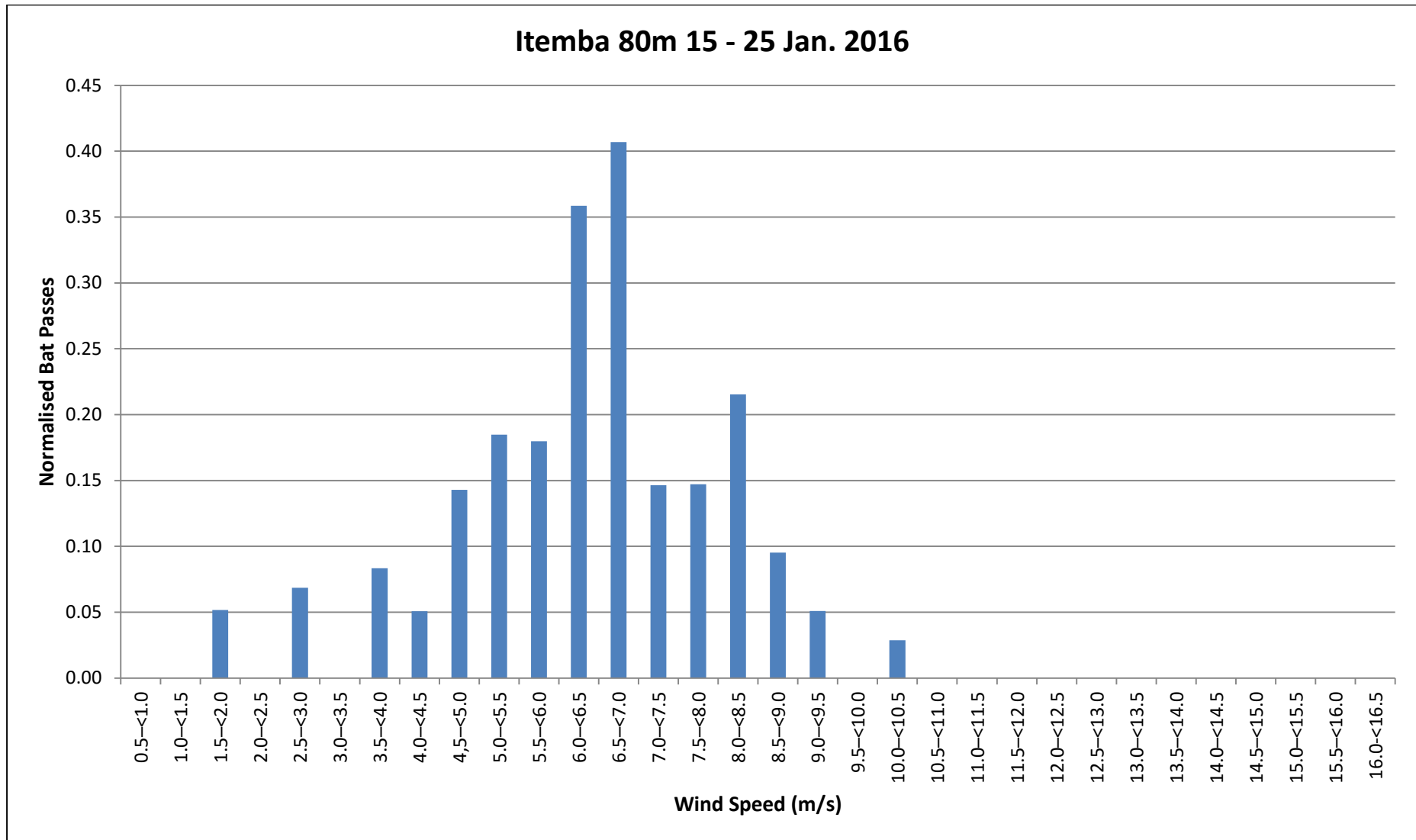
Figure 65: Sum of bat passes (Normalised) per Wind Speed category for Itemba 80m (15 – 25 January 2016).
