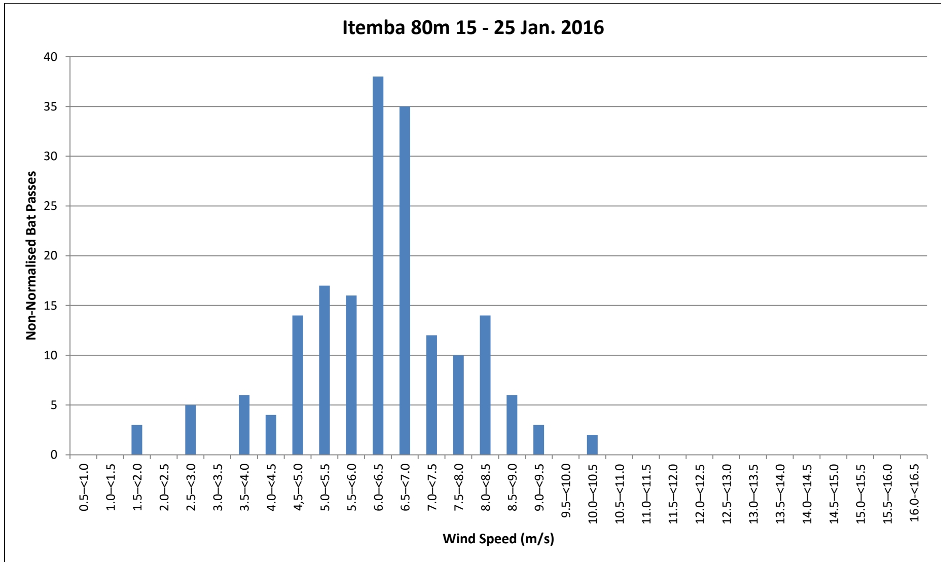
Figure 66: Sum of bat passes (Non-normalised) per Wind Speed category for Itemba 80m (15 – 25 January 2016).
