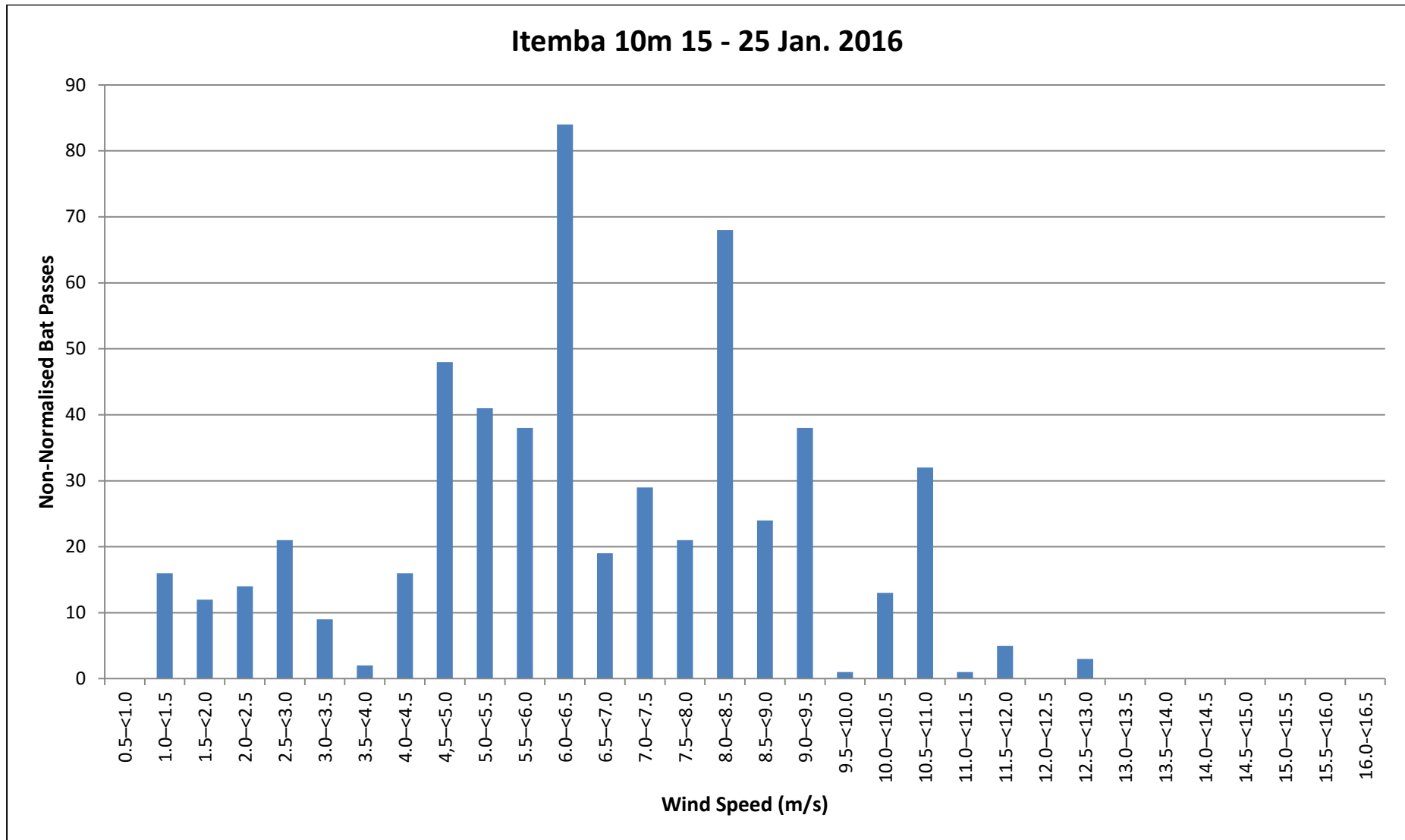
Figure 60: Sum of bat passes (Non-normalised) per Wind Speed category for Itemba 10m (15 – 25 January 2016).
