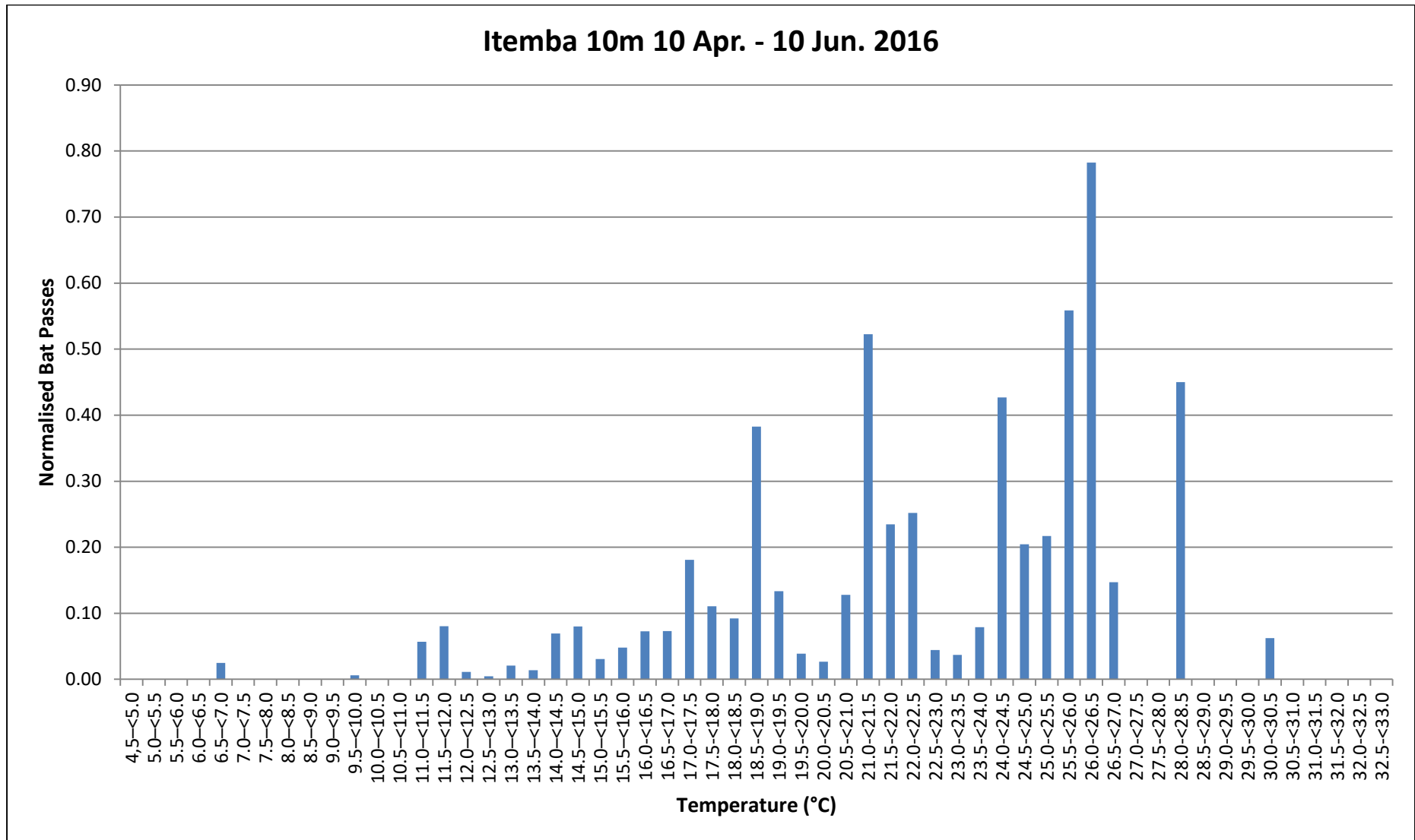
Figure 74: Sum of bat passes (Normalised) per Temperature category for Itemba 10m (10 April – 10 June 2016).
