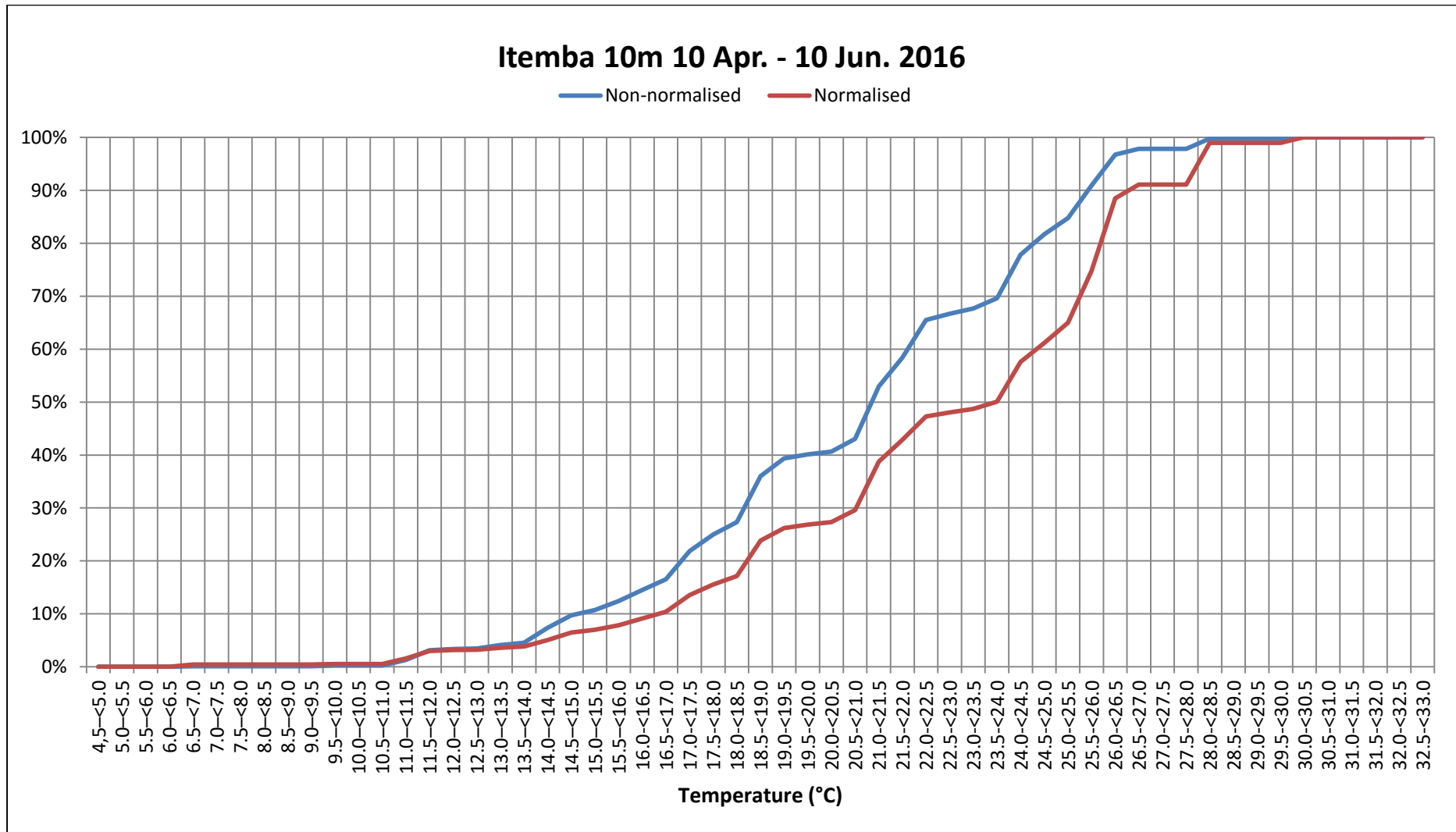
Figure 76: Cumulative percentage of normalised and non-normalised bat passes per Temperature category for Itemba 10m (10 April – 10 June 2016).
