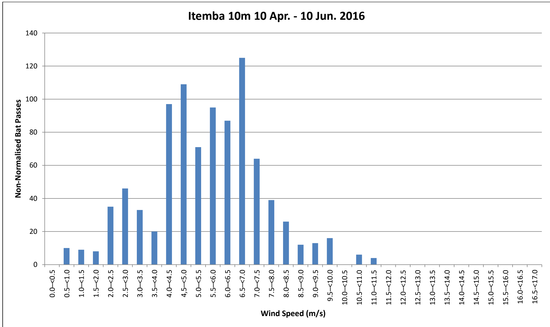
Figure 78: Sum of bat passes (Non-normalised) per Wind Speed category for Itemba 10m (10 April – 10 June 2016).
