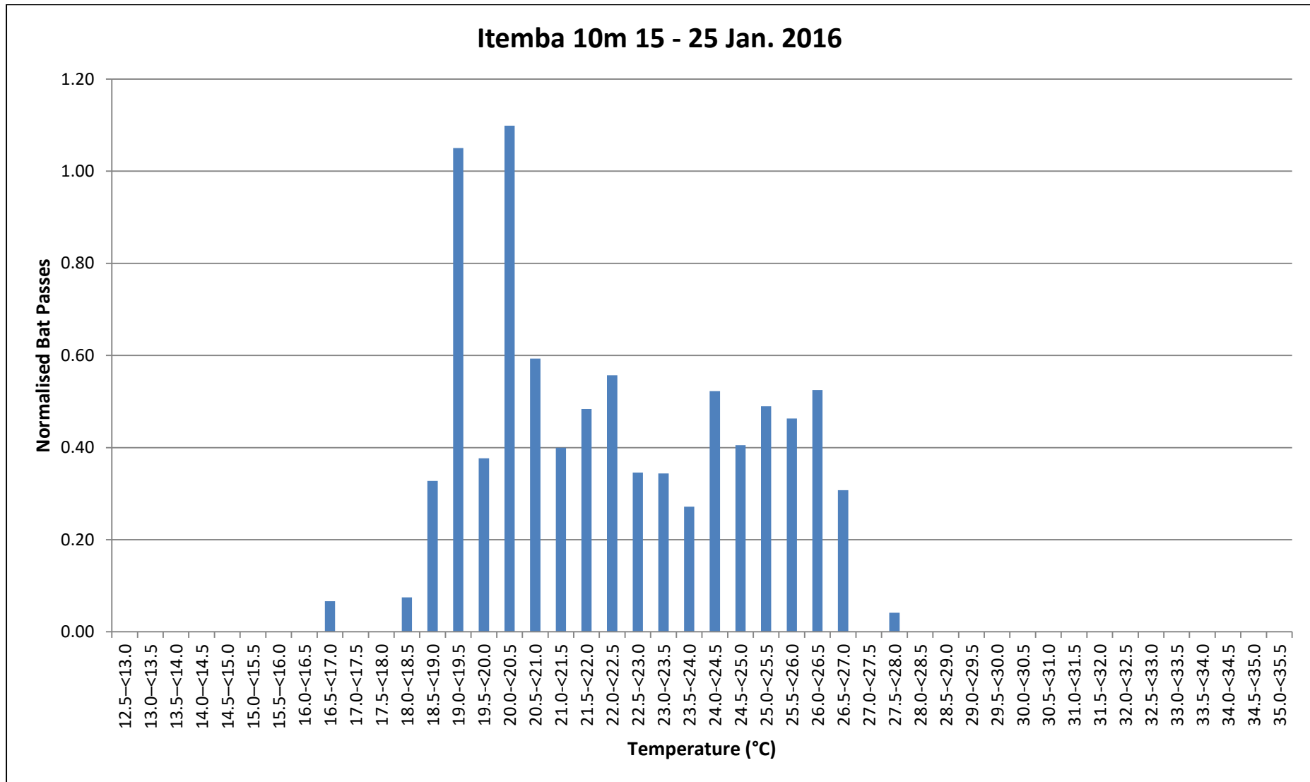
Figure 56: Sum of bat passes (Normalised) per Temperature category for Itemba 10m (15 – 25 January 2016).
