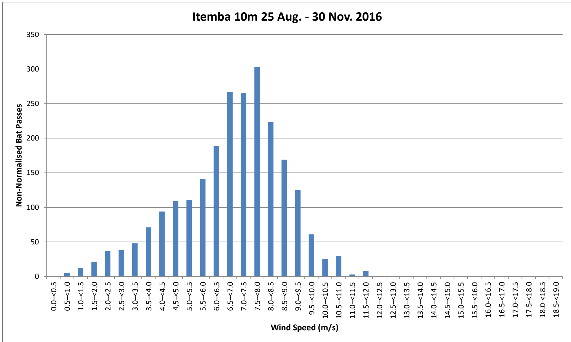
Figure 84: Sum of bat passes (Non-normalised) per Wind Speed category for Itemba 10m (25 August – 30 November 2016).
