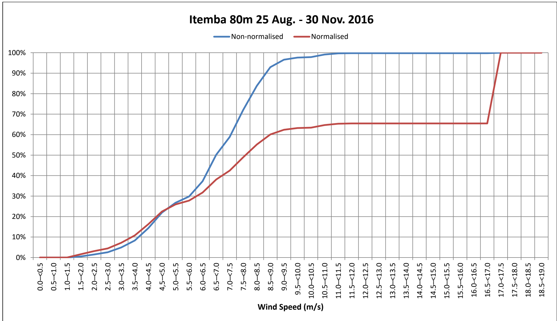
Figure 91: Cumulative percentage of normalised and non-normalised bat passes per Wind Speed category for Itemba 80m (25 August – 30 November 2016).
