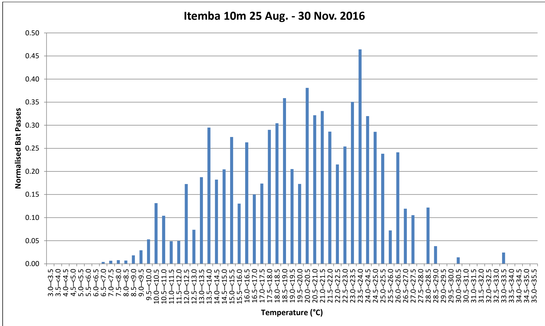
Figure 80: Sum of bat passes (Normalised) per Temperature category for Itemba 10m (25 August – 30 November 2016).
