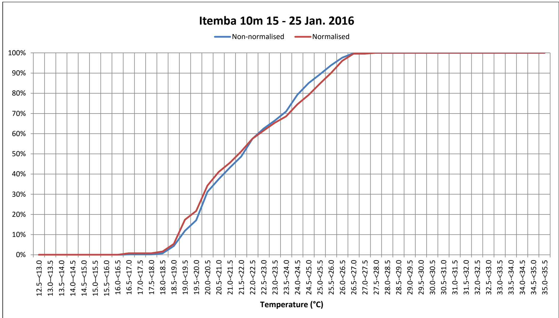
Figure 58: Cumulative percentage of normalised and non-normalised bat passes per temperature category for Itemba 10m (15 – 25 January 2016).
