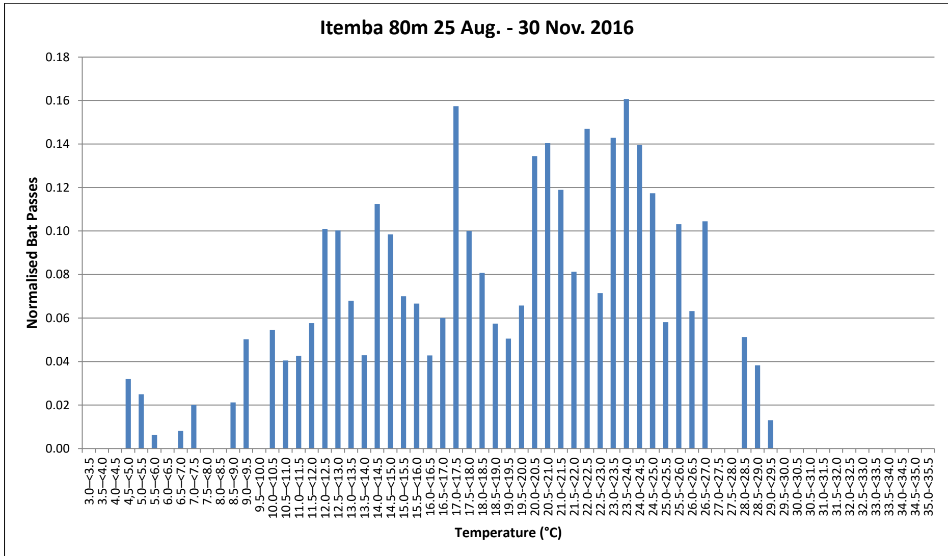
Figure 86: Sum of bat passes (Normalised) per Temperature category for Itemba 80m (25 August – 30 November 2016).
