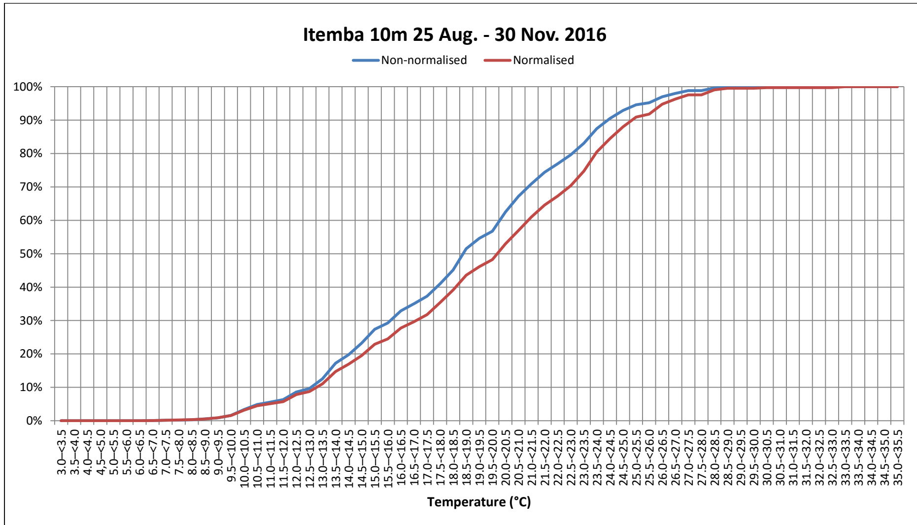
Figure 82: Cumulative percentage of normalised and non-normalised bat passes per Temperature category for Itemba 10m (25 August – 30 November 2016).
