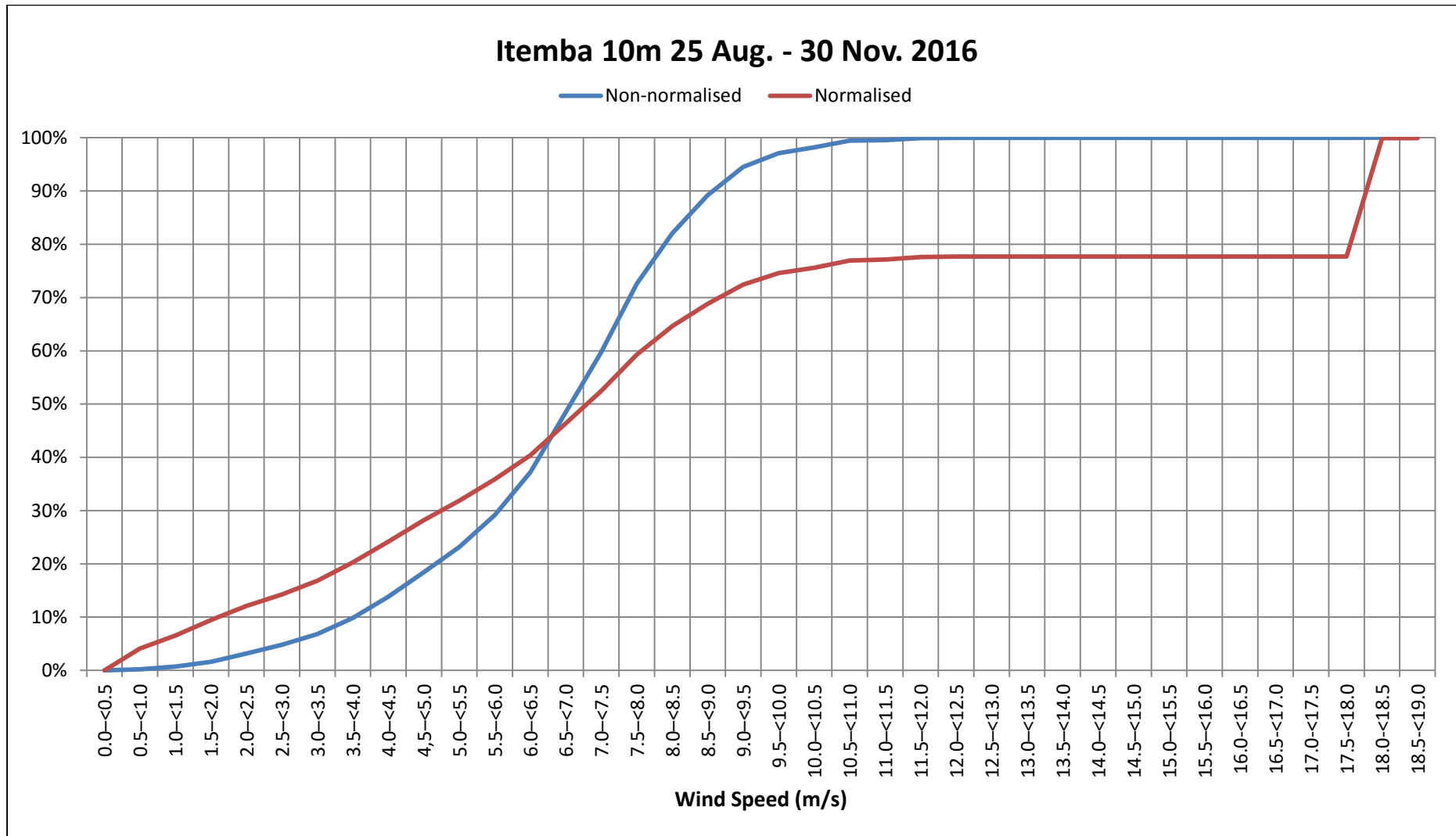
Figure 85: Cumulative percentage of normalised and non-normalised bat passes per Wind Speed category for Itemba 10m (25 August – 30 November 2016).
