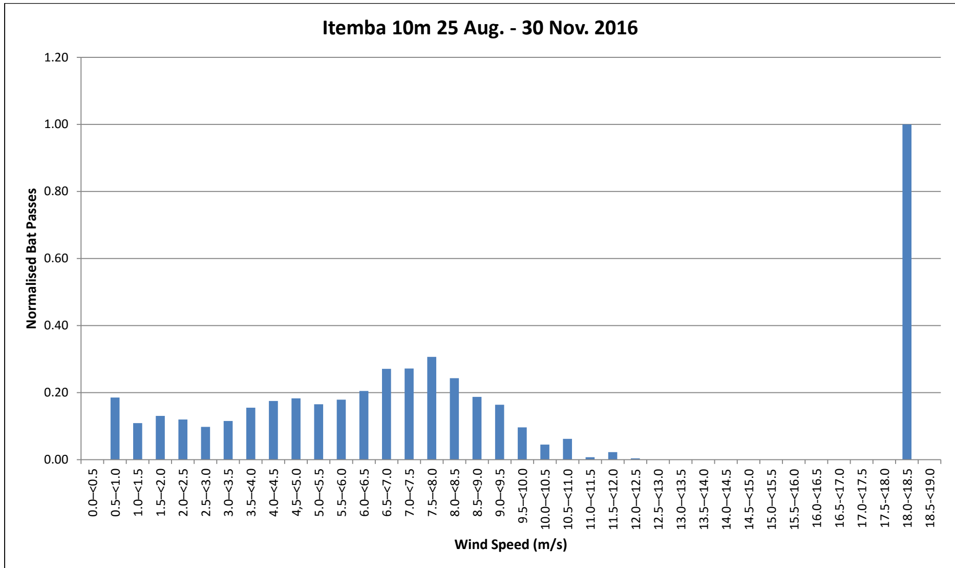
Figure 83: Sum of bat passes (Normalised) per Wind Speed category for Itemba 10m (25 August – 30 November 2016).
