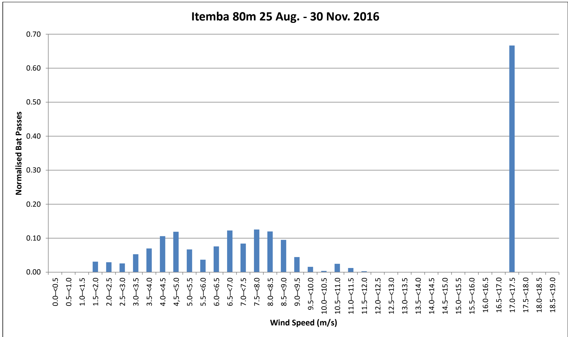
Figure 89: Sum of bat passes (Normalised) per Wind Speed category for Itemba 80m (25 August – 30 November 2016).
