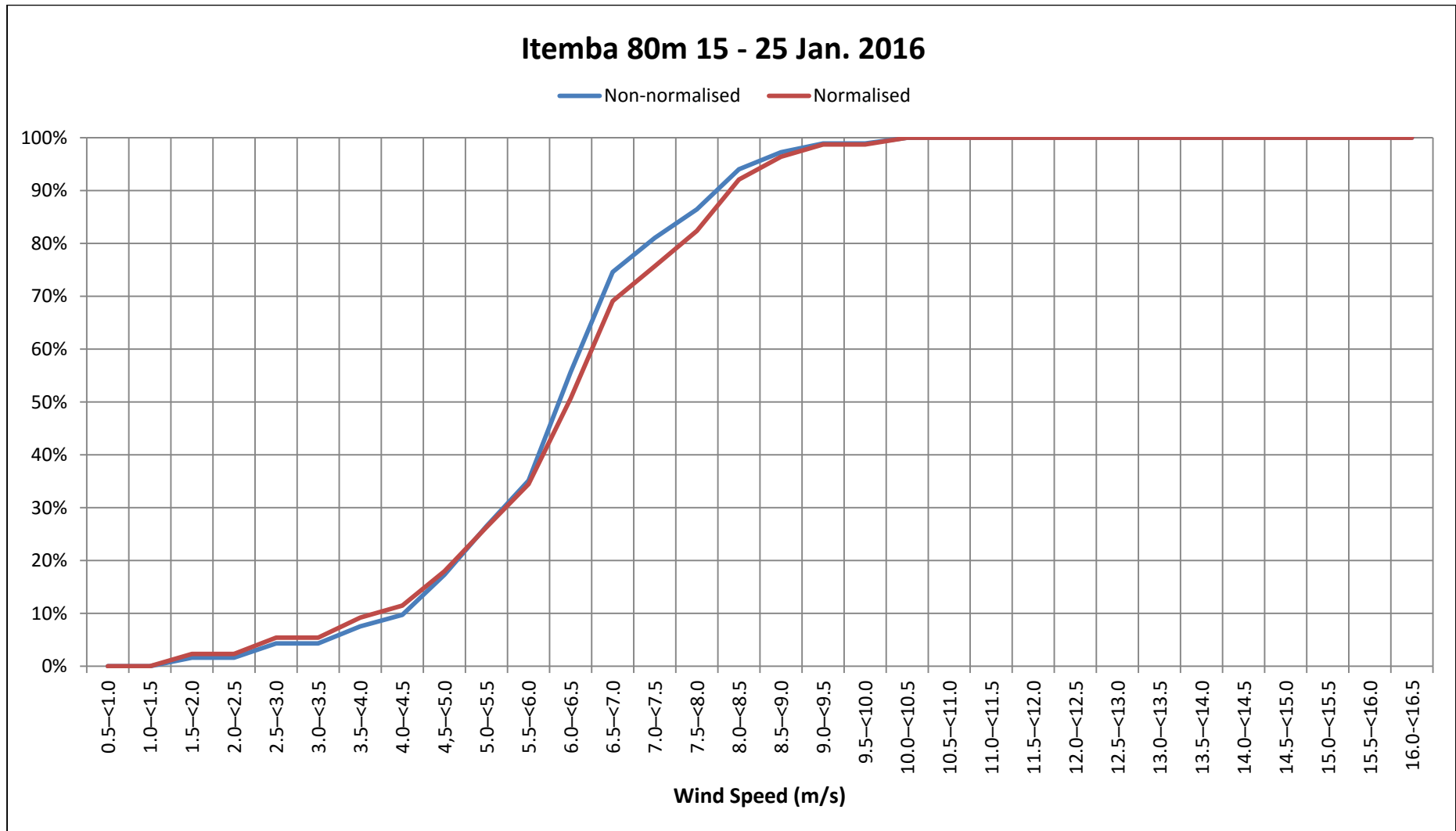
Figure 67: Cumulative percentage of normalised and non-normalised bat passes per Wind Speed category for Itemba 80m (15 – 25 January 2016).
