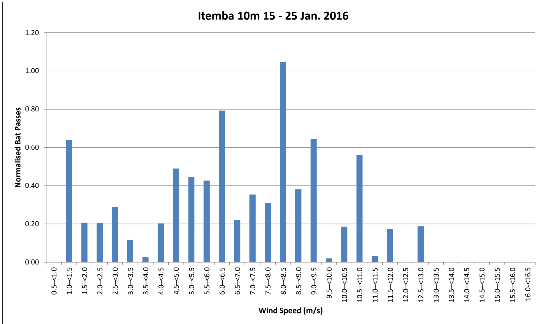
Figure 59: Sum of bat passes (Normalised) per Wind Speed category for Itemba 10m (15 – 25 January 2016).
