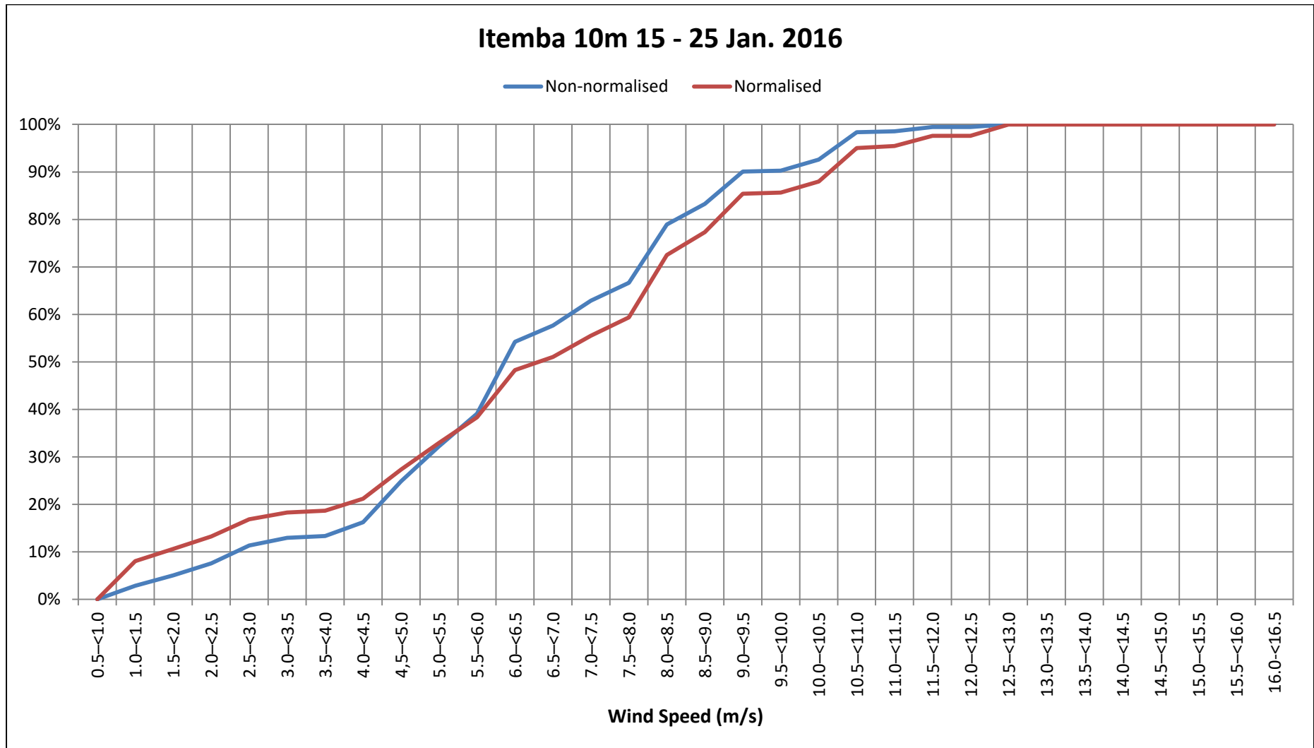
Figure 61: Cumulative percentage of normalised and non-normalised bat passes per Wind Speed category for Itemba 10m (15 – 25 January 2016).
