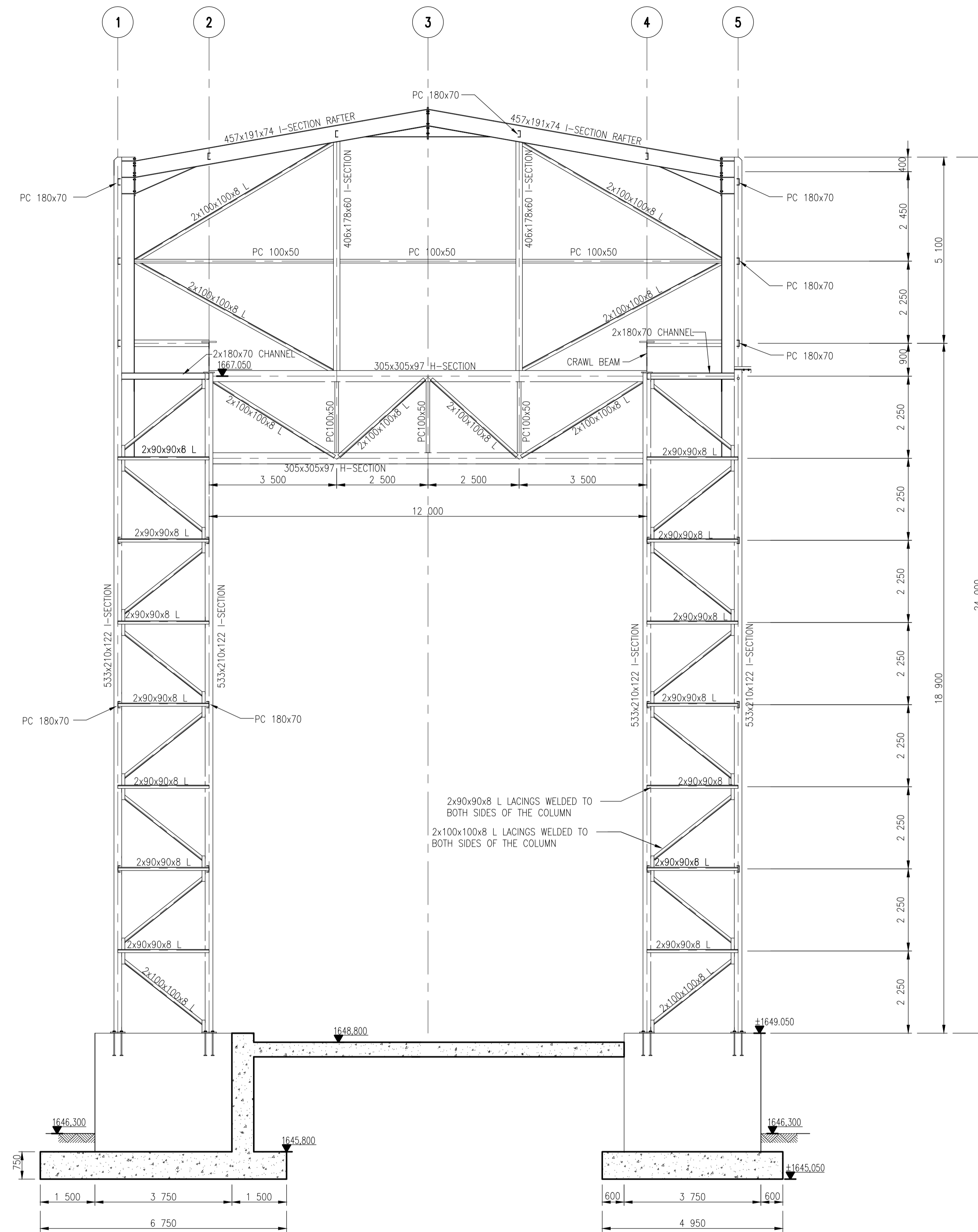
STEEL LAYOUT ON GRIDLINE A SCALE 1:75
