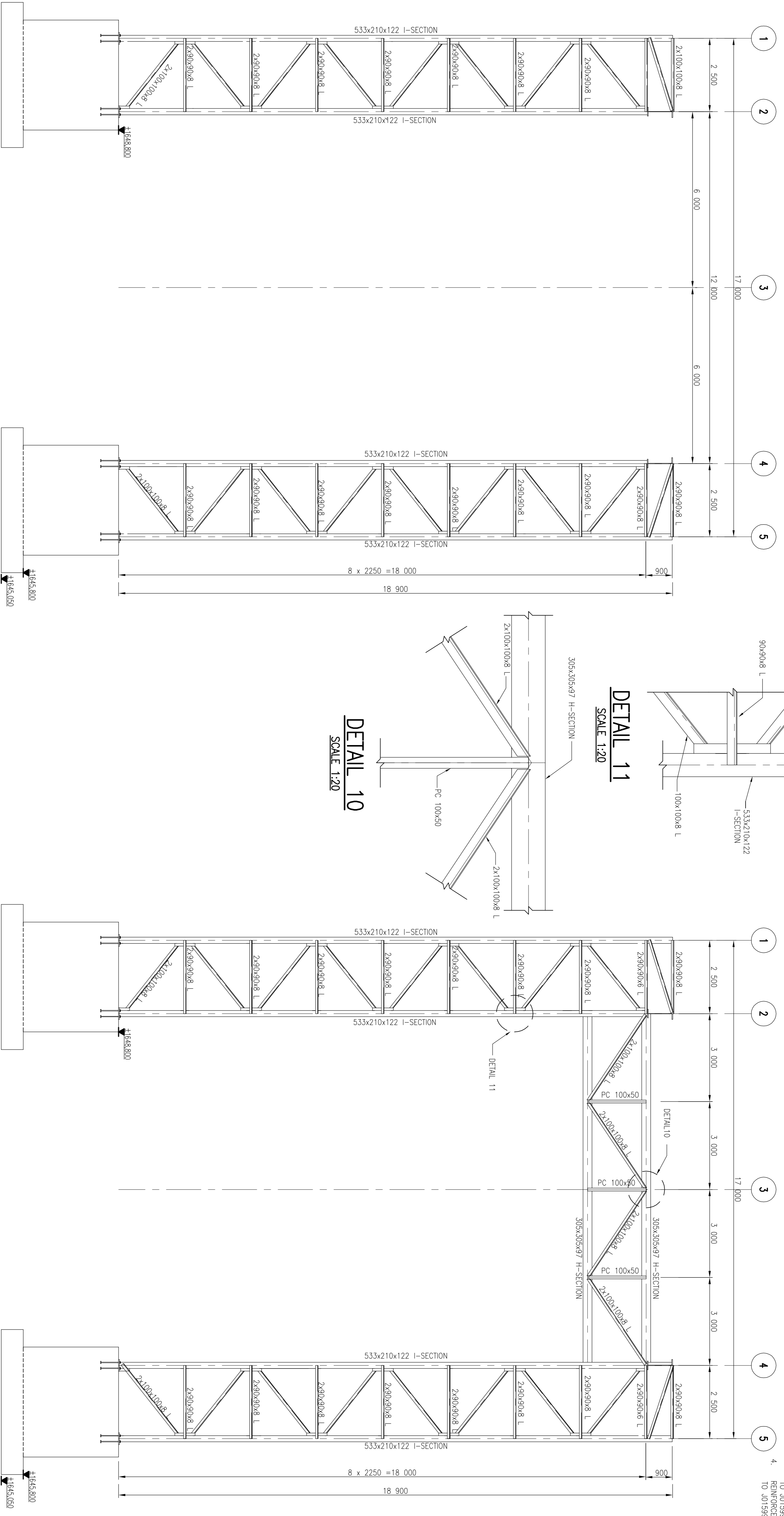
STEEL LAYOUT ON GL E, F & G SCALE 1:75
